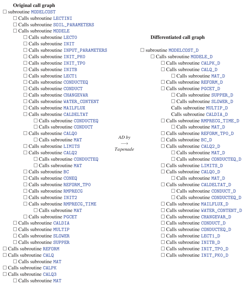
Figure E.1: Differentiation of the MHFEM code by Tapenade.
