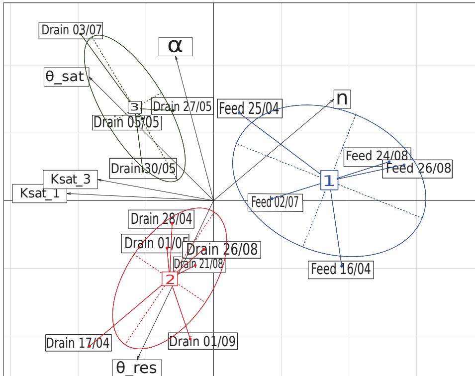
Figure 5.20: Biplot of individuals and variables - Principal Component Analysis for variables: \alpha and n : vGM form parameters. Ksat_1: Saturation hydraulic conductivity for the first layer. Ksat_3: Saturation hydraulic conductivity for the third layer. \theta_{res} : Residual water content. \theta_{sat} : Saturated water content for individuals: Feed x/y and Drain x/y represent respectively the feeding and drainage sub-period occurring at the start date day/month.
