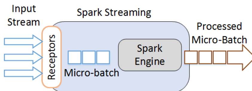
Figure 4.8: Micro-batch processing used in Spark stream. The input streams are received by receptors and it transforms in micro-batch that are executed in a traditional Map-Reduce Spark Engine.
