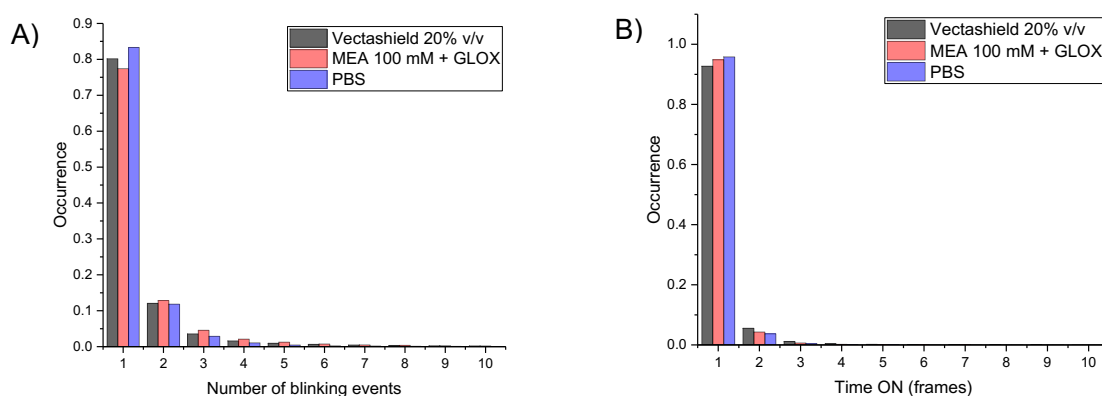
Figure S1. Comparison of the photophysical properties of overexpressed mEos2 in aqueous buffer (PBS), in the standard imaging buffer of thiols with oxygen scavenging system (MEA 100 mM + GLOX) and in the Vectashield mounting medium. A) Distributions of the number of blinks after photoactivation. B) Distributions of the ON time measured for mEos2 after photoactivation.
