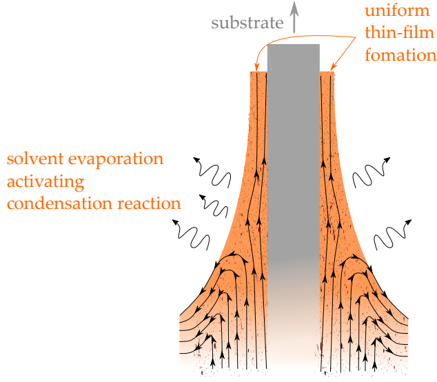
Figure 2.21: Thin film formation during dip-coating.
