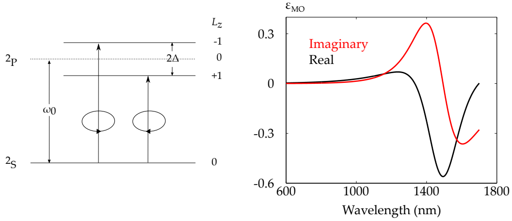
Figure 2.6: Diamagnetic transition.
