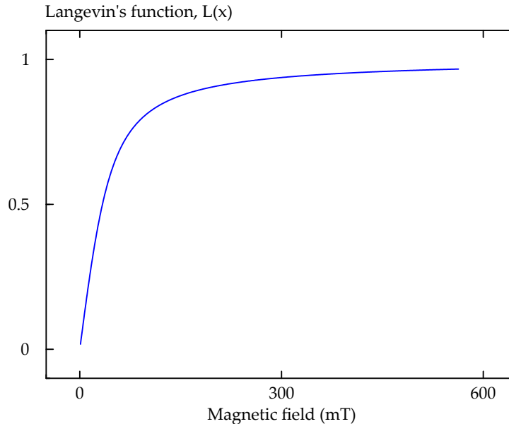
Figure 2.10: Langevin’s function.
