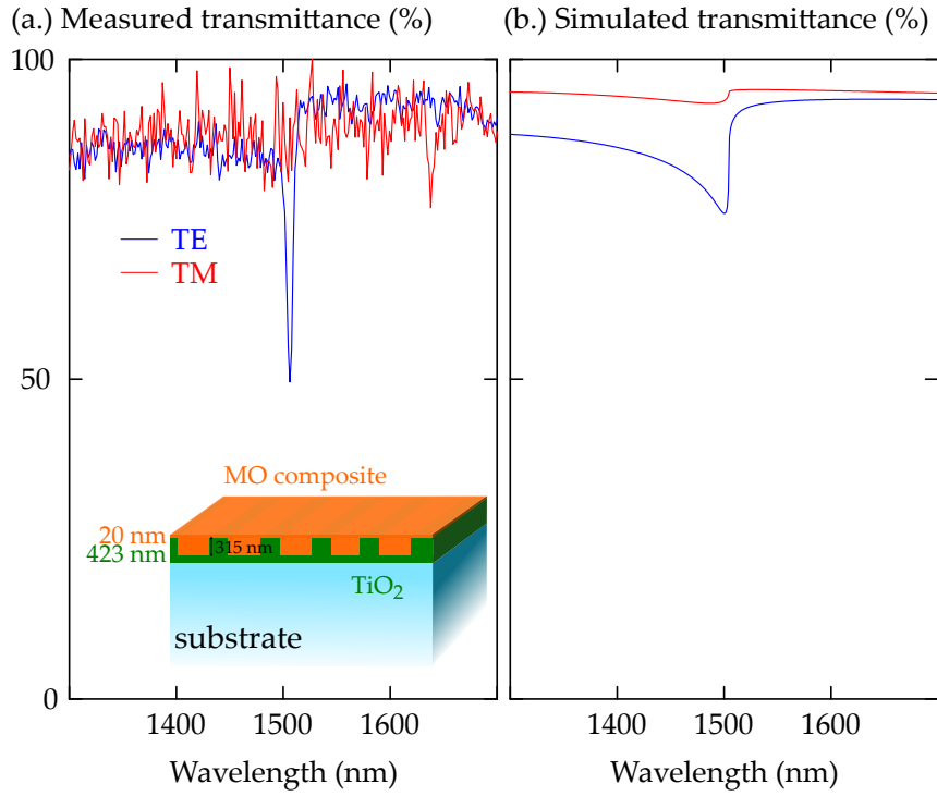
Figure 3.11: Transmittance measured (a.) and simulated (b.) of \text{TiO}_2 -based MO structure (inset) at normal incidence.
