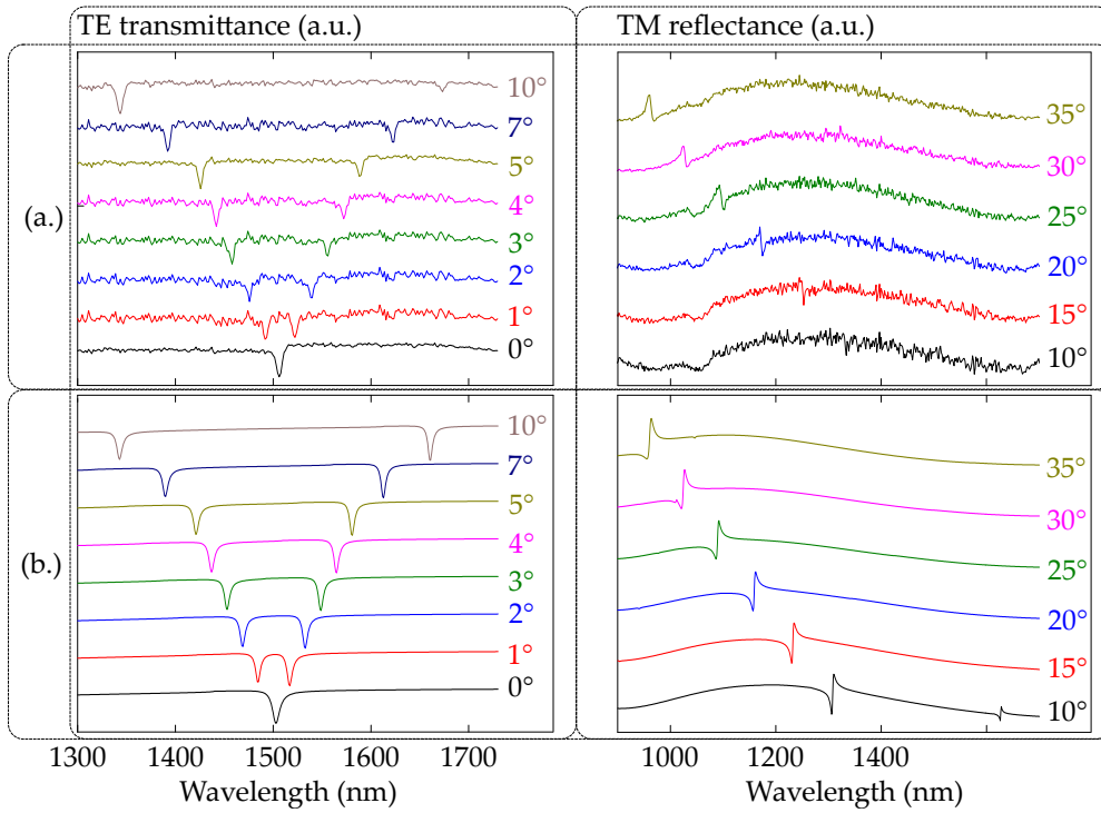
Figure 3.12: Experimental (a.) and simulated (b.) angle variation of TE transmittance (left) and TM reflectance (right) for a \text{TiO}_2 -based MO grating.
