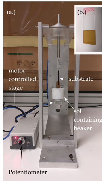
Figure 2.22: (a.) Snapshot of the dip-coating apparatus used to produce homogeneous thin-films of MO composite. (b.) (inset) MO thin film prepared by dip-coat method.
