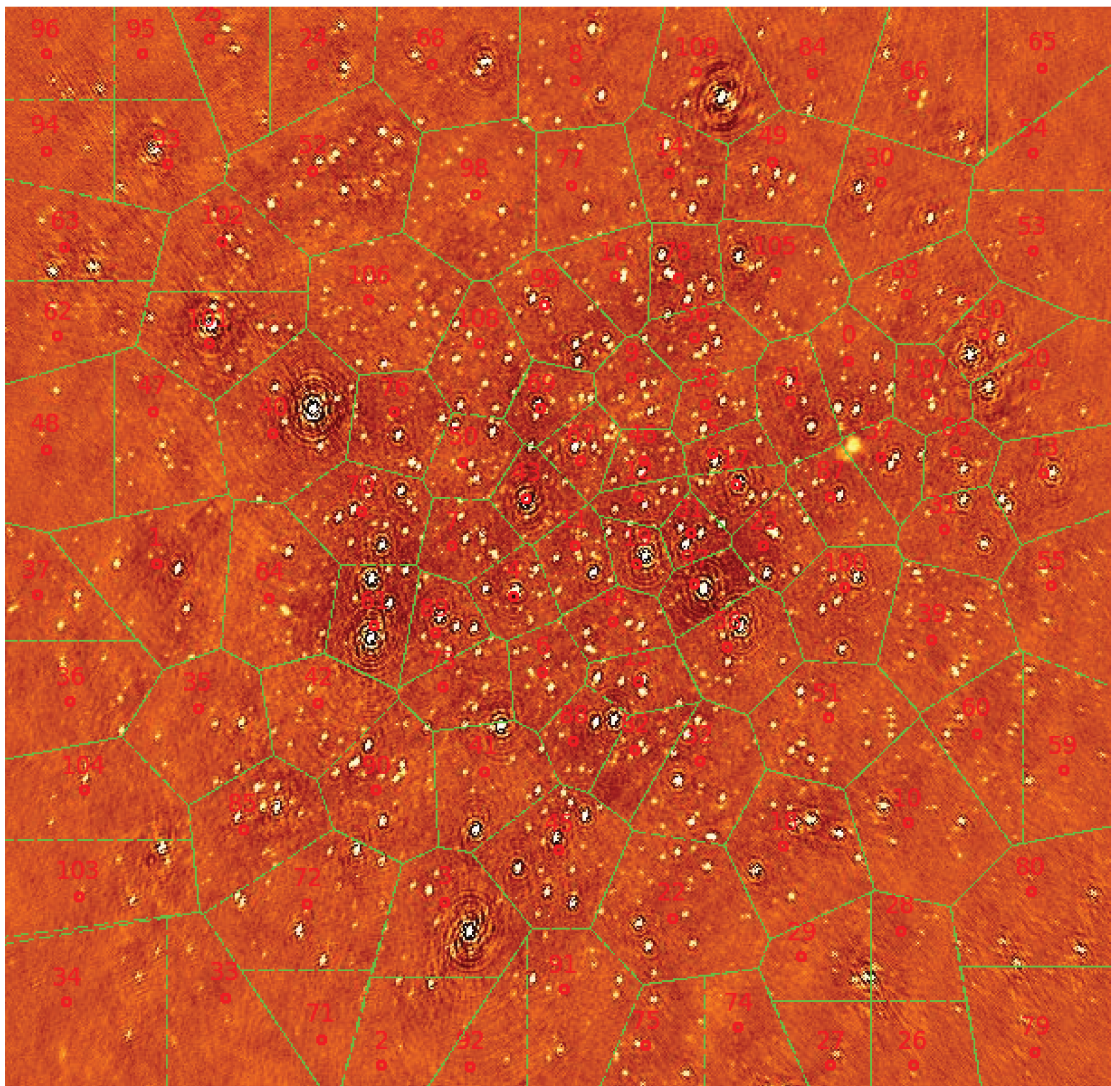
Figure 2.16. Voronoi facets, as implemented in DDFacet. Image is made before application of direction-dependent correction. This is an image of the Bootes field, made by Cyril Tasse.
