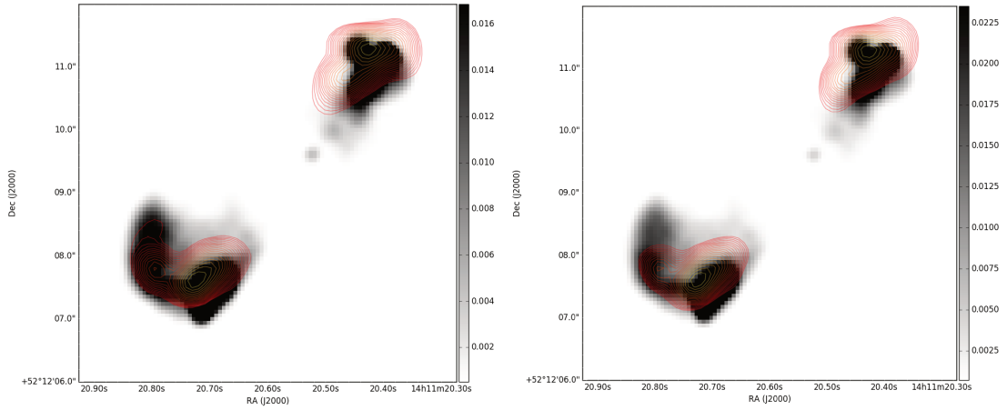
(a) Overlay of our model of 3C295 at 116.6 MHz over our initial VLA model.
