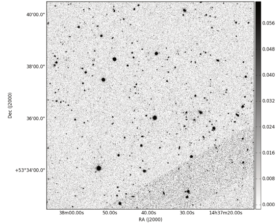
(d) Same image as Fig. 4.6b, with WISE overlay.
