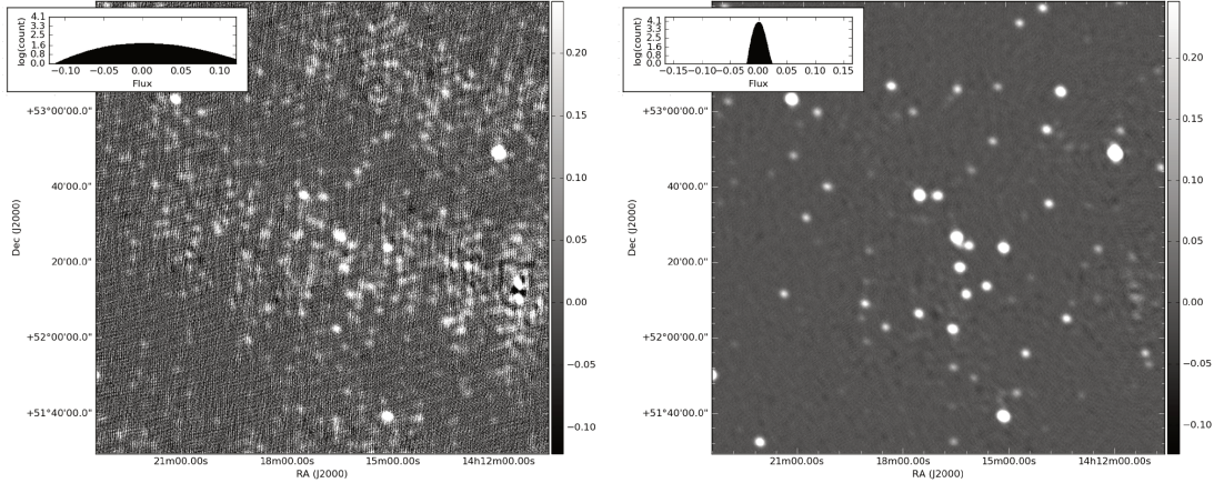
(a) Poorly-calibrated, unweighted restored image of the sky near the centre of the Extended Groth Strip. Units of colourbar are Jy/bm. rms=86.4mJy/beam
