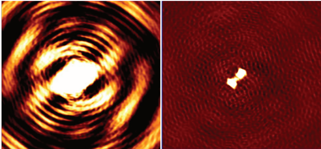
Figure 2.9. Effect of deconvolution on a dirty image of 3C295. To the left, the dirty image; to the right, the deconvolved image (same size, resolution & flux scale, made with the same data). As we can see, the latter is much more scientifically interesting.
