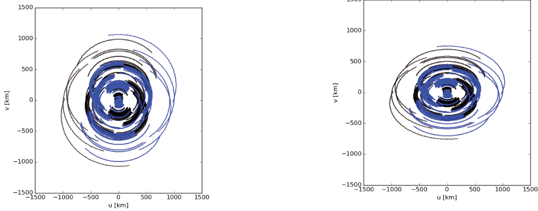
(b) uv -coverage of an 8-hour LOFAR observation when pointing 45 degrees away from zenith.
