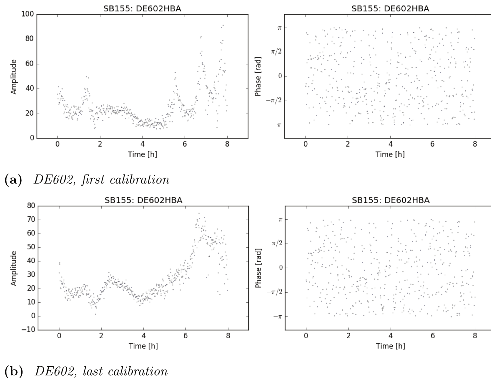
Figure 5.8. Gain amplitude & phase for DE602 of SB155
