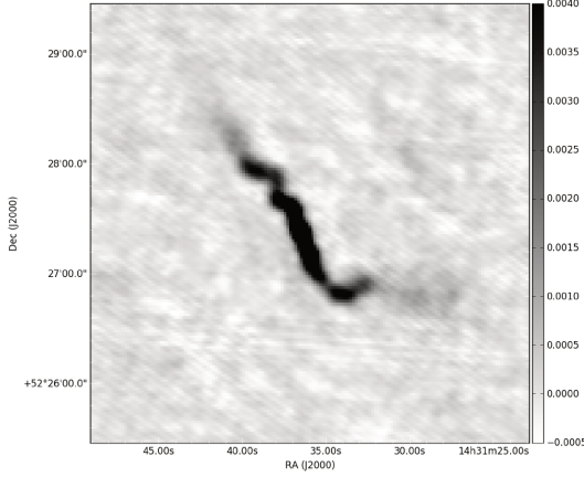
(a) Cutout of our LOFAR wide-field image centred on EGS-4.
