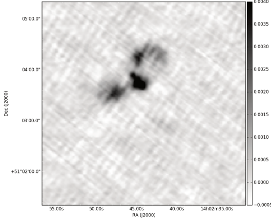
(a) Cutout of our LOFAR wide-field image centred on EGS-12.
