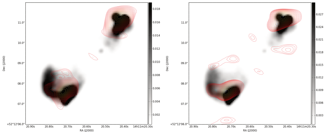
(e) Overlay of our model of 3C295 at 164.256 MHz over our initial VLA model.
