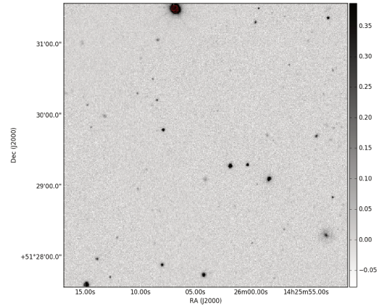
(d) Same image as Fig. 4.11b, with WISE overlay.
