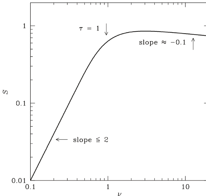
Figure 1.6. Characteristic spectrum of free-free radiation. Arbitrary unit scale. Source: NRAO online course: https://www.cv.nrao.edu/course/ast534/FreeFreeEmission.html .
