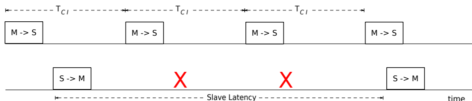
Figure 2.8: BLE Connected Mode with Slave Latency non-zero
