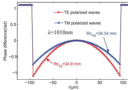
Fig. 7. Simulated resulting phase difference profile at work wavelength \lambda_0 = 1010nm using elliptical holes ( f_x = 0.6 and varying f_y ). PC thickness=280nm, Spacer thickness=142nm, a=280nm. TE / TM-polarized waves experience different radius of curvature.
