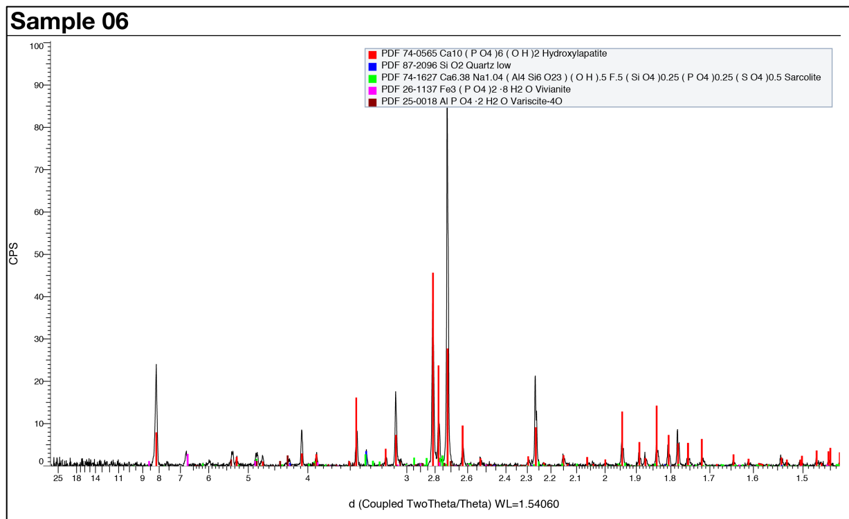
Figure 89. X-ray diffractogram of Sample 6.
