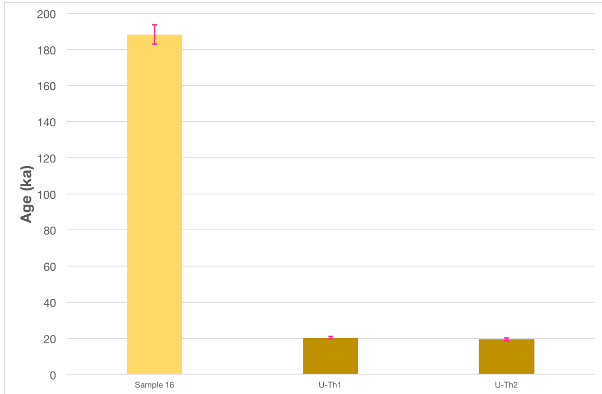
Figure 177. Calculated uranium-series ages of the gypsum sample analyzed for this study (Sample 16; in light yellow), compared with those in the gypsum samples analyzed by Lewis et al. (2008) (U-Th1 and U-Th2; in dark yellow).
