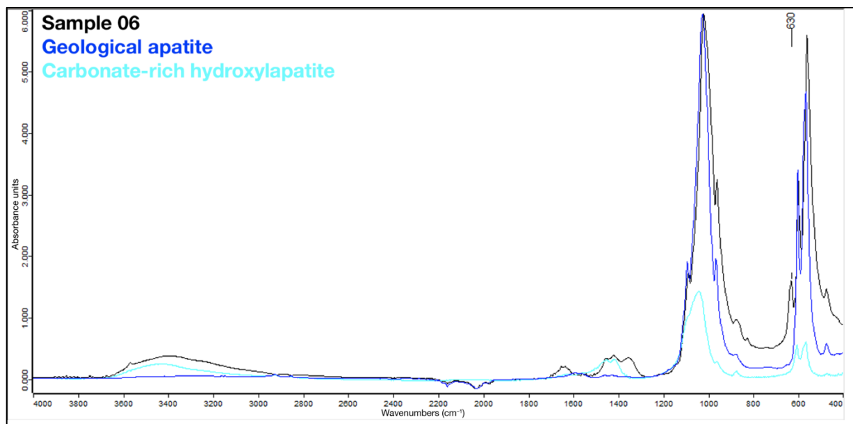
Figure 88. ATR-FTIR spectrum of Sample 6 in absorbance mode.
