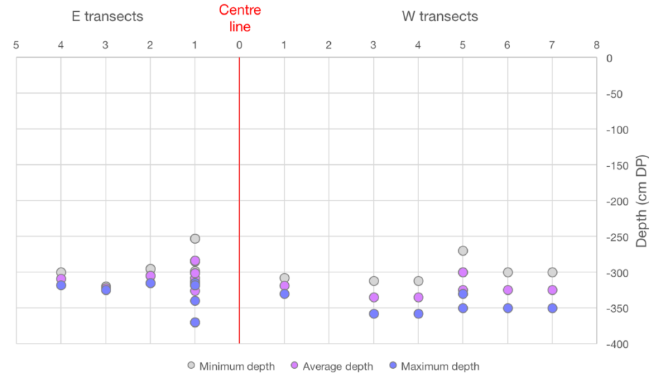
East-West view
