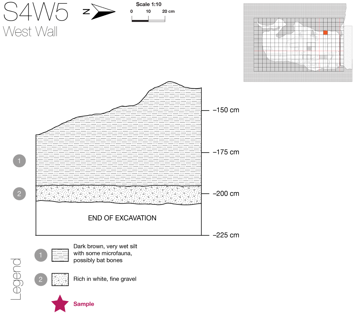
Figure 23. West Wall vertical profile for Square S4W5.
