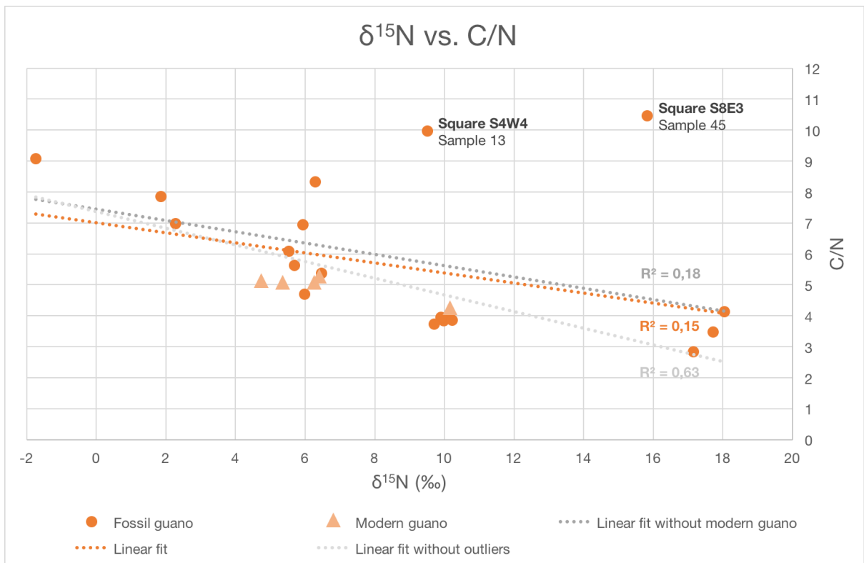
Figure 162. δ 15 N against C/N. Labelled points are considered outliers (Samples 13 and 45).
