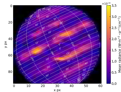
Fig. 2. Map of the mean observed radiance for the reduced spectral cube in the 1930–1943 \text{cm}^{-1} wavenumber range taken the 16 January 2016 at 11h10 UTC. The Great Red Spot can be seen around pixel [32, 70]. The longitudes are in system III and the latitudes are planetocentric. (For interpretation of the references to colour in this figure legend, the reader is referred to the web version of this article.)
