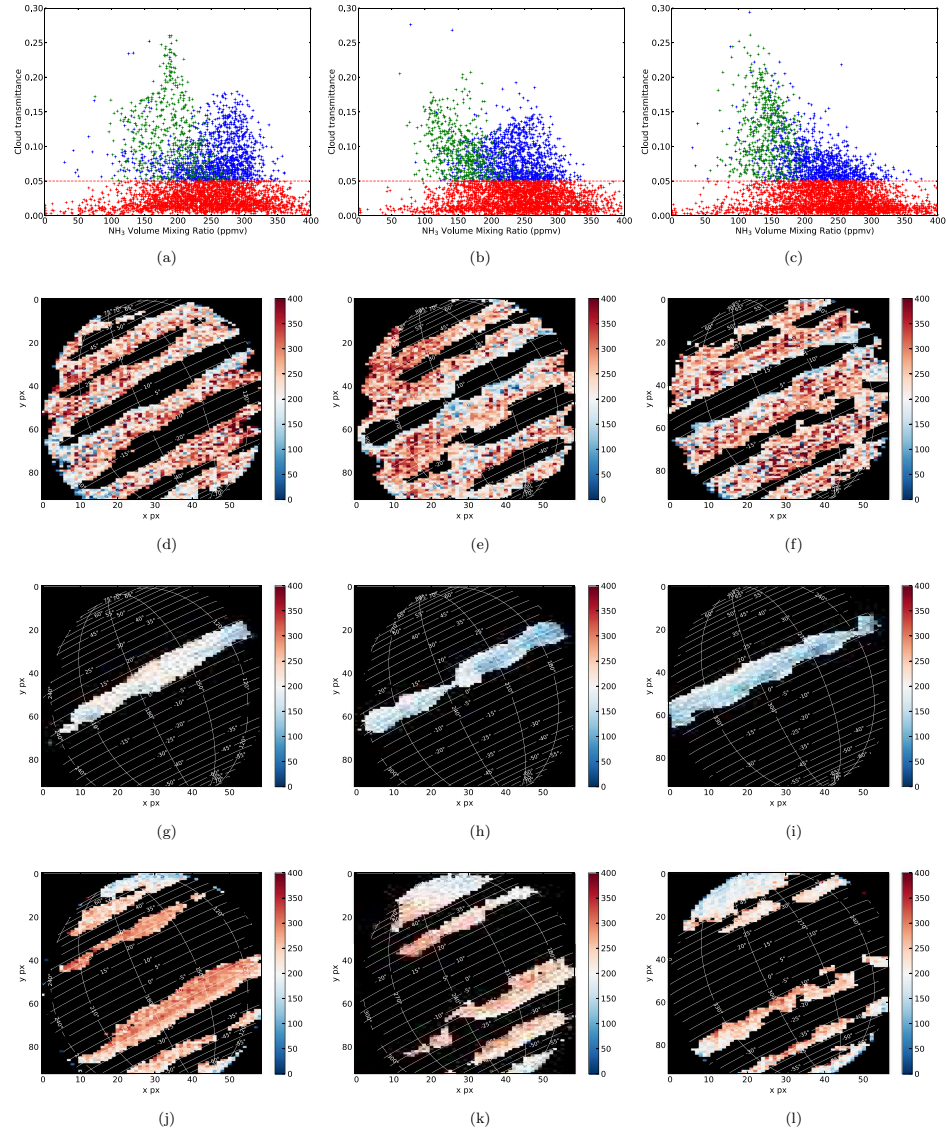
Fig. 14. Figures (a) to (c): retrieved cloud transmittance in function of our retrieved NH 3 abundance for each spectrum of the spectral cube taken at 09h36, 11h10 and 12h50 (see Table 1) in this order from left to right. Red: spectra with a retrieved cloud transmittance lower than 0.05, corresponding to the zones. Green: spectra with a retrieved cloud transmittance greater than 0.05 and located between latitudes 0 and 17°N, corresponding to the NEB. Blue: spectra located outside the NEB with a cloud transmittance greater than 0.05. Figures (d) to (l): retrieved NH 3 abundance and location of each spectra of each of our spectral cube, for each of the filters used in figure (a) to (c). From top to bottom: spectra corresponding to respectively the red, green and blue points of figures (a) to (c). From left to right: spectra corresponding to respectively the figure (a), (b) and (c). Latitudes are planetocentric and longitudes are in system III. (For interpretation of the references to colour in this figure legend, the reader is referred to the web version of this article.)
