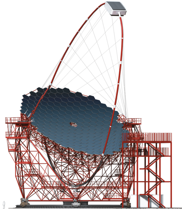
FIGURE 2.2 – Grand télescope de CTA (Large Size Telescope, LST).
