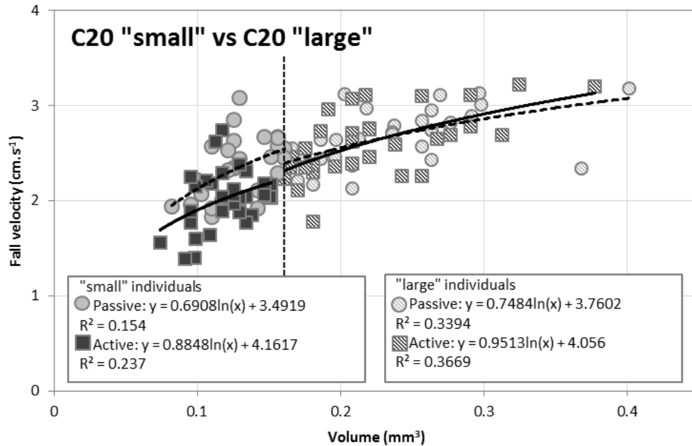
Figure 21: Relationship between fall velocity and recruit's volume for passive recruits and active recruits of two size classes ("small" and "large") of C20 condition. Dotted and continuous curves correspond respectively to regressions of passives and for recruits and vertical dotted line correspond to med the median size of C20 ( 0.16 \text{ mm}^3 ).
