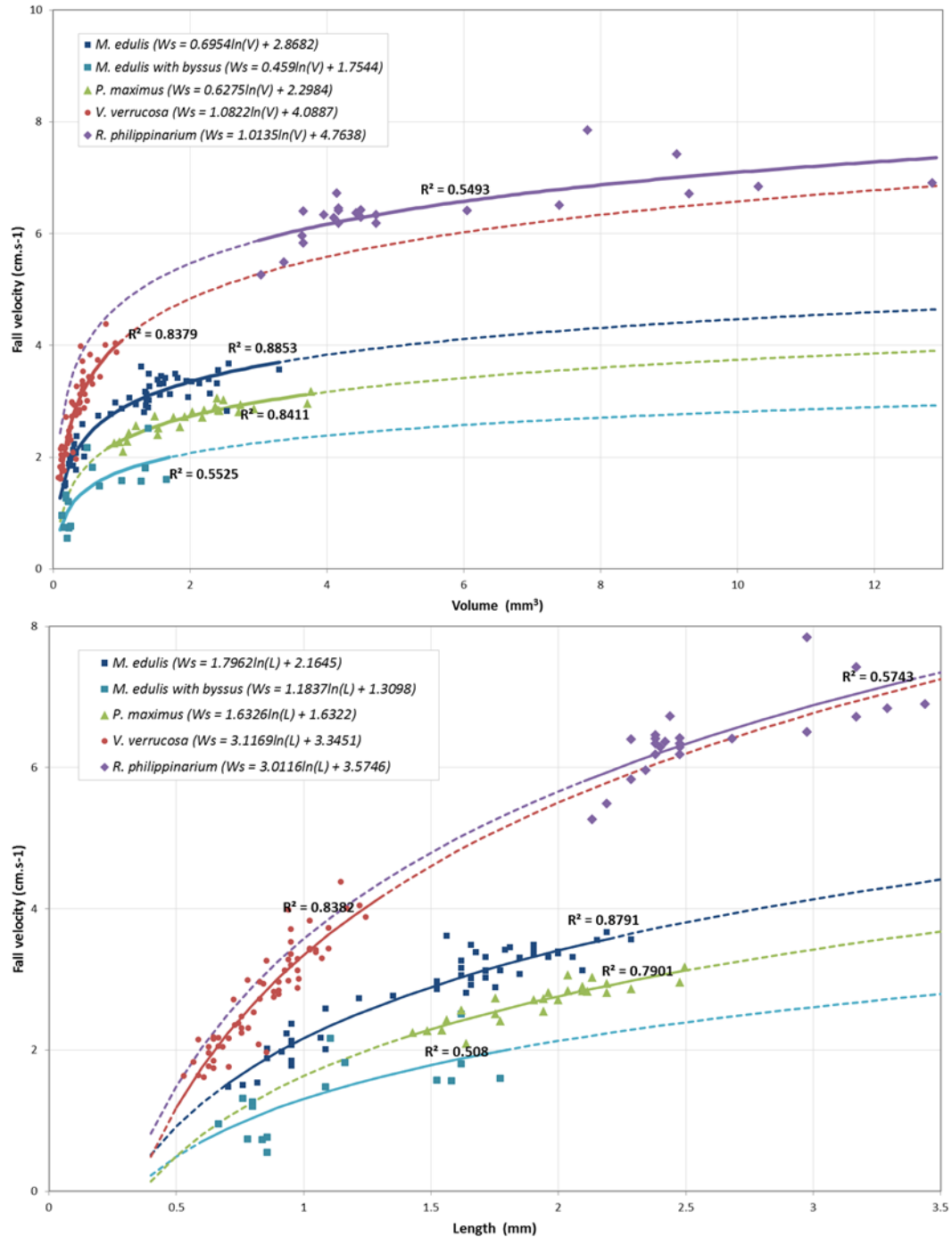
Figure 12: Relationships between fall velocity and volume or shell length for active recruits of the four species and mussel recruits producing byssus thread. Lines are logarithmic regression curves ( Ws = a \times \ln(\text{Size}) + b ) with their respective coefficients of determination ( R^2 ), the solid lines relate to the size range of the individuals studied for each species and the dashed lines correspond to an extension of the regression outside this range.
