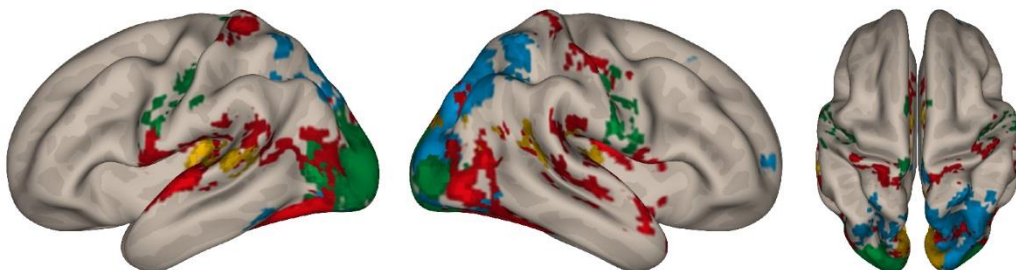
Figure 2.2.1 – Unique functional connectivity in neonates and adults
