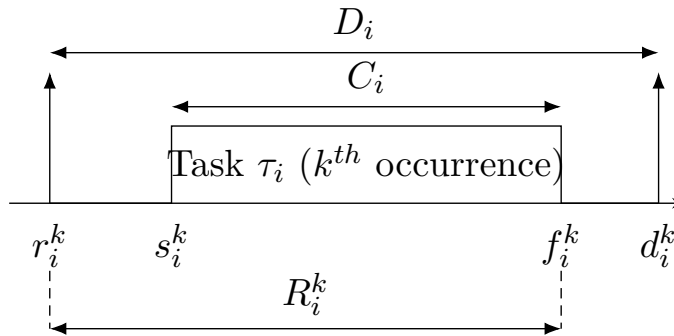
Figure 2.13: Parameters of a real-time task.
