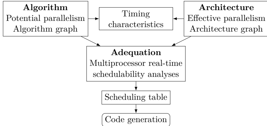
Figure 2.14: The Algorithm-Architecture-Adequation methodology.
