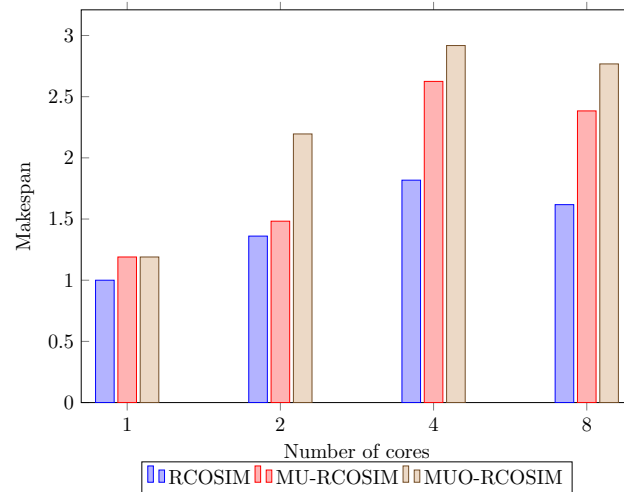
Figure 6.16: Speedup results.
