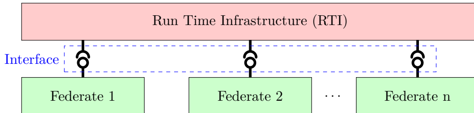
Figure 2.9: HLA federation.
