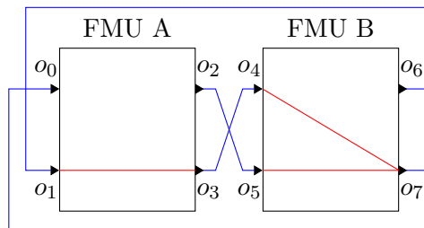
FMU-level view
