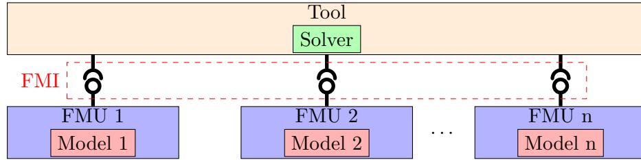
Figure 2.7: FMI for Model Exchange.
