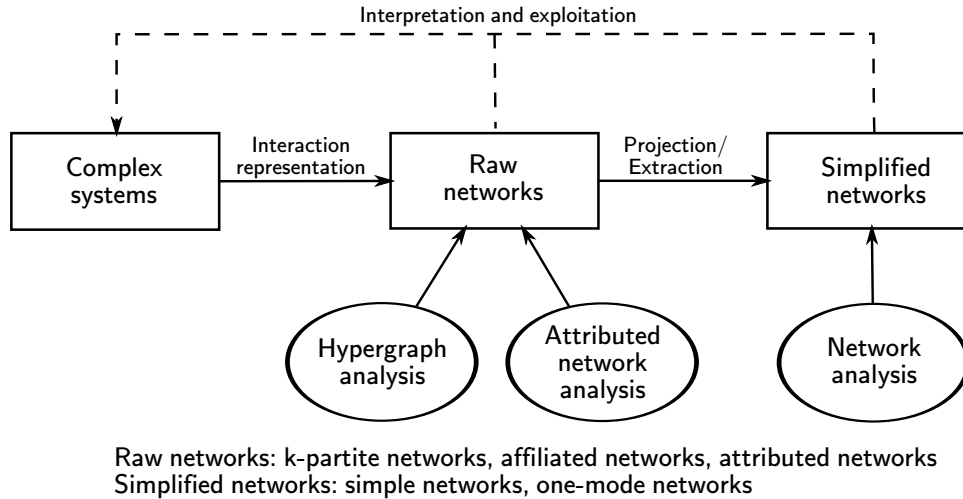
FIGURE 2.1: A summarized learning cycle using network analysis tools to extract and comprehend complex system information. The process is illustrated in a network science viewpoint.
