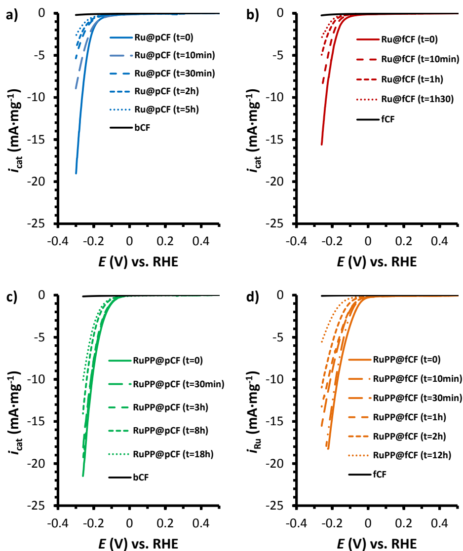
Figure 17. LSV curves of A) Ru@pCF, B) Ru@fCF, C) RuPP@pCF and D) RuPP@fCF, along a bulk electrolysis experiment at 1M \text{H}_2\text{SO}_4 pH=0. An E_{\text{app}}=250 mV was used for Ru@xCF systems to reach i_{\text{cat}}\approx 10 \text{mA}\cdot\text{mg} during the electrolysis, and E_{\text{app}}=150 mV for RuPP-based systems.
