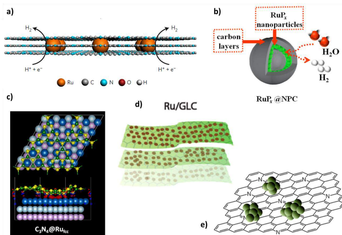
Figure 19. Ru-based nanosystems as HECs: a) Baek's Ru@C 2 N, 119 b) Liu's Ru P x @NPC, 127 c) Qiao's Ru/C 3 N 4 /C, 131 d) Adschiri's Ru/GLC 125 and e) Tour's Ru-NG750. 130
