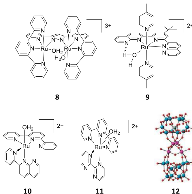
Figure 12. Structure of Llobet's dinuclear [\text{Ru}^{\text{II}}_2(\text{bpp})(\text{trpy})_2(\text{H}_2\text{O})_2]^{3+} ( 8 ), Thummel's [\text{Ru}^{\text{II}}(\text{tnp})(\text{Mepy})_2(\text{H}_2\text{O})]^{2+} ( 9 ) and [\text{Ru}^{\text{II}}(\text{trpy})(\text{pynap})(\text{H}_2\text{O})]^{2+} ( 10 ), Meyer's [\text{Ru}(\text{trpy})(\text{bpm})(\text{OH}_2)]^{2+} ( 11 ), and Bonchio's \text{Ru}_4\text{-POM} ( 12 ).
