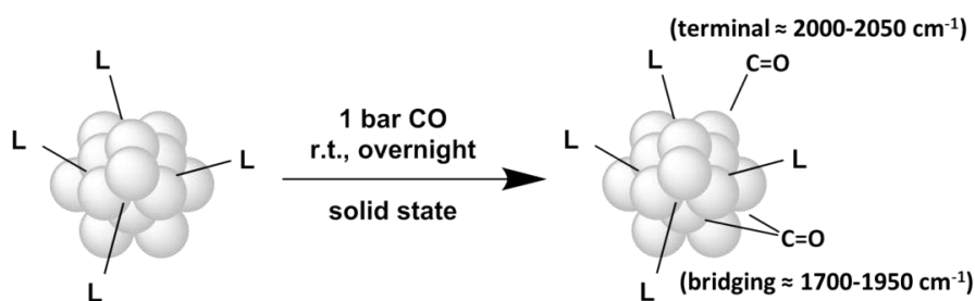
Scheme 2. Conditions for the reaction of CO at Ru nanoparticles' surface.
