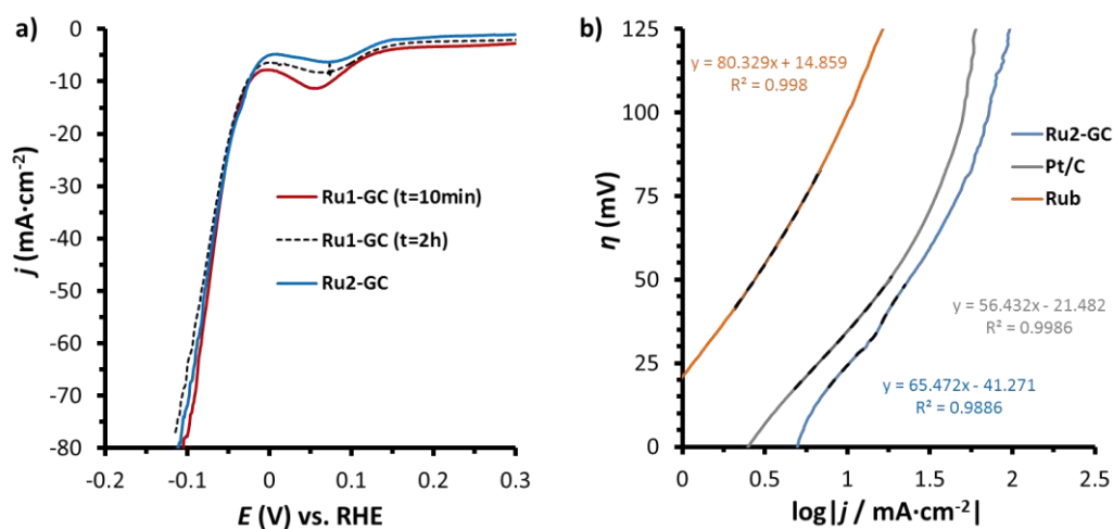
Figure 11. a) Polarization curves of Ru1-GC (dark red, after 10 minutes, electrode and electrochemical set-up preparation time) and at t=2\text{h} (dashed black), and Ru2-GC (blue) in 1 M NaOH. b) Tafel plot of Ru2-GC (blue), Pt/C (grey) and Rub (orange) in 1 M NaOH.
