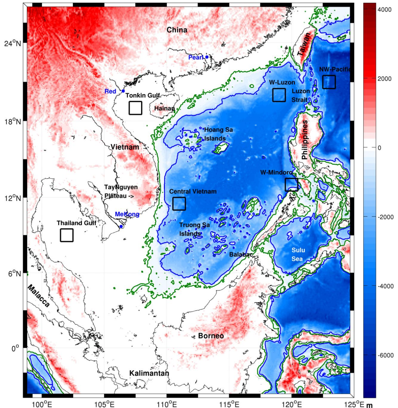
Figure 1.1 Geography and bathymetry of the South China Sea. The green and blue contours represent isobaths of 100 and 1000 m (data from GEBCO). The black rectangles represent locations and area (1°x1°) for calculation of mean temperature-salinity profiles in Figure 1.15.
