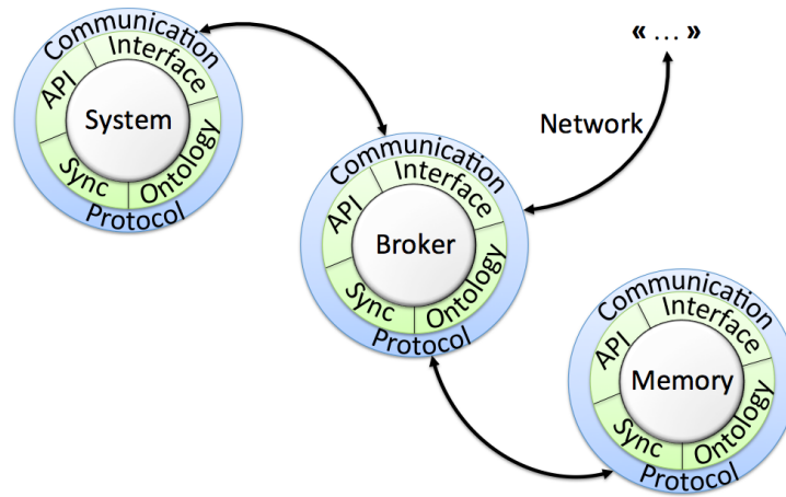
Figure 4.1: The MBA architecture proposed by this research.
