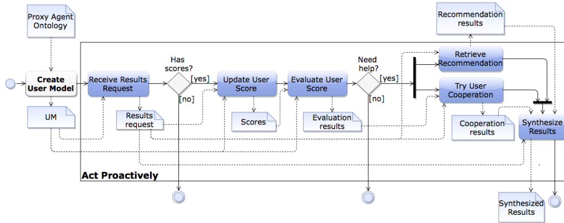
Figure 5.9: The steps of the “Act Proactively” activity of the ProPA method.
