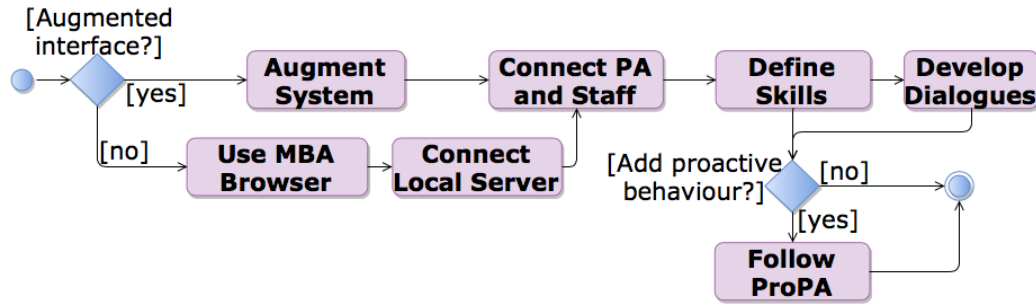
Figure 8.3: The steps of the Integrate Proactive Interfaces of the GAMBAD method.
