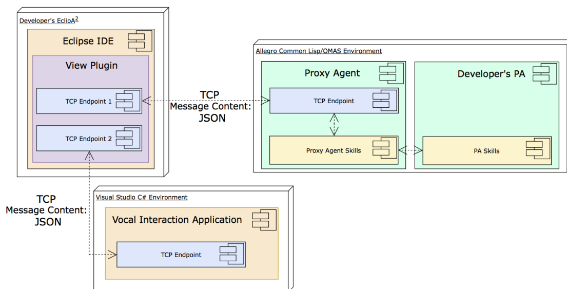
Figure 6.8: Integrating a natural language interface in the EclipA 2 through an augmented approach.
