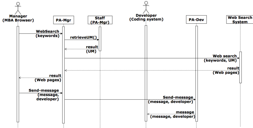
Figure 6.4: A sequence diagram showing a request made by a manager for code quality information, and interaction with other team members in the ACE4SD SoS.
