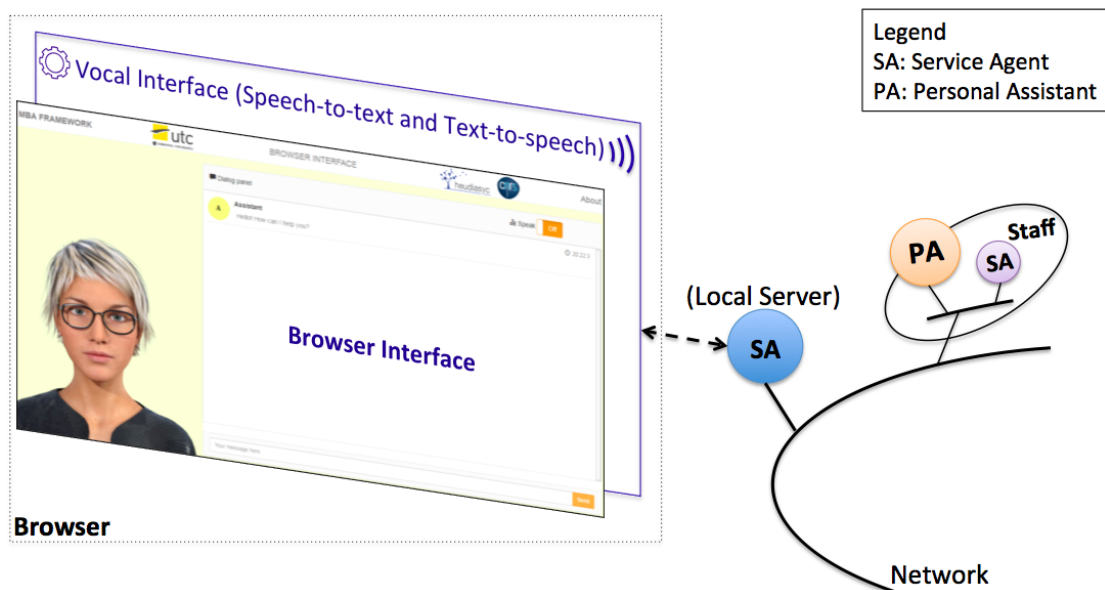
Figure F.1: The MBA Browser system and its components.
