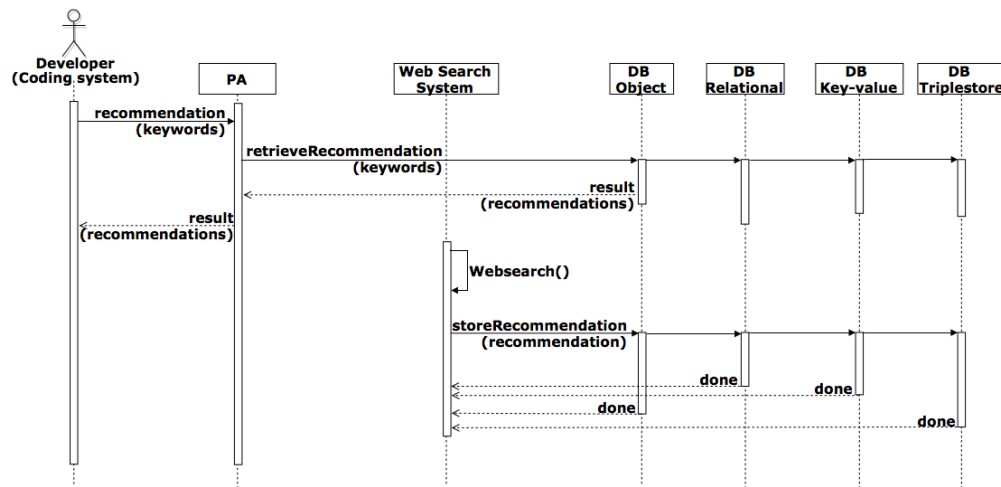
Figure 6.2: A sequence diagram showing a request made by a developer for receiving quality recommendations in the ACE4SD SoS.
