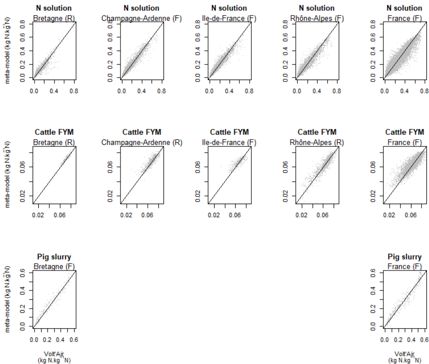
Figure 13: Scatter plot of metamodels selected by year-by-year cross-validation versus Volt'Air simulated emission rates (in \text{kg N.kg}^{-1} \text{N} ). The letters R and F stand for regional and France metamodel, respectively, for each fertilizer type.
