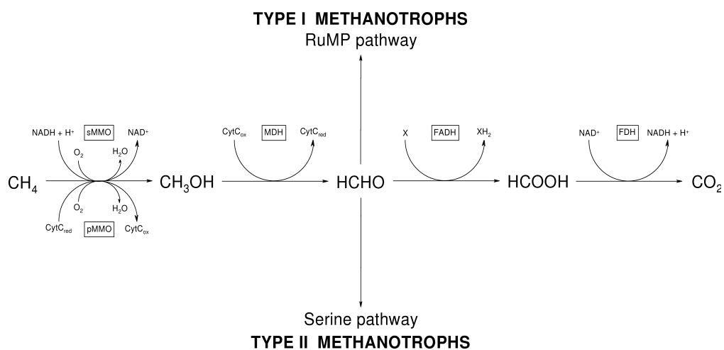
Figure 6. Oxidation pathway of methane to methanol and formaldehyde. SMMO – soluble methane monooxygenase; pMMO – particulate methane monooxygenase; MDH – methanol dehydrogenase, FADH – formaldehyde dehydrogenase, FDH – formate dehydrogenase (Hanson and Hanson, 1996).
