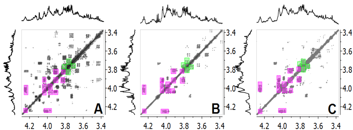
Figure 4. EPSs spectral patterns in COSY spectra of IM media of Bacillus sp. 3B6 on: A – glucose after 48 h; B – glucose after 63 h and C – cellulose after 63 h. Cross-peaks marked by: pink colour – due to dextran type of polysaccharide with \alpha -1,6-linked galactose in the backbone; green colour – non identified isolated -O-CH_2- group.
