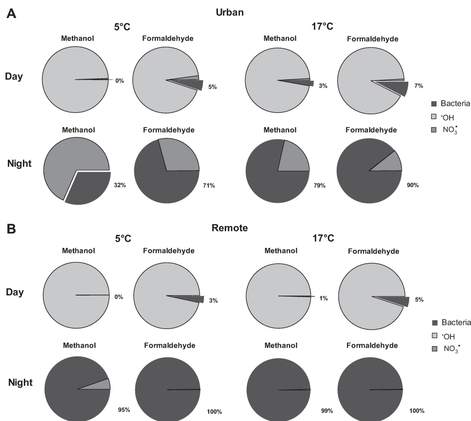
Fig. 4. Estimated relative influence of bacterial activity and free radicals ( \cdot\text{OH} and \text{NO}_3^- ) on the degradation of methanol and formaldehyde in cloud water at 5 °C and 17 °C during the day and the night for both cloud air mass types: urban (A) and remote (B) cases. During nighttime (i.e. in the absence of photochemical reactivity), \cdot\text{OH} radicals are considered not present. The rates of degradation for cloud conditions are those reported in Table 2.
