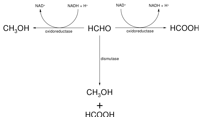
Figure 8. Disproportionation pathways of formaldehyde to formate and methanol, catalysed by \text{NAD}^+ -dependent oxidoreductase or formaldehyde dismutase.
