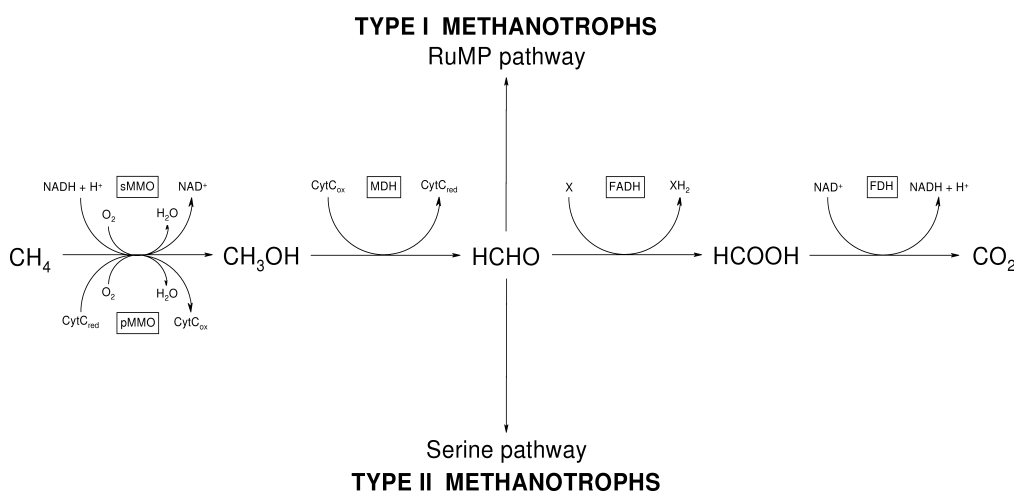
Figure 6. Oxidation pathway of methane to methanol and formaldehyde. SMMO – soluble methane monooxygenase; pMMO – particulate methane monooxygenase; MDH – methanol dehydrogenase, FADH – formaldehyde dehydrogenase, FDH – formate dehydrogenase (Hanson and Hanson, 1996).
