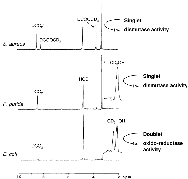
Figure 15. In vivo ^2\text{H} NMR spectra of incubations of Staphylococcus aureus , Pseudomonas putida , and E. coli cells with deuterated formaldehyde (Mason and Sanders, 1989).
