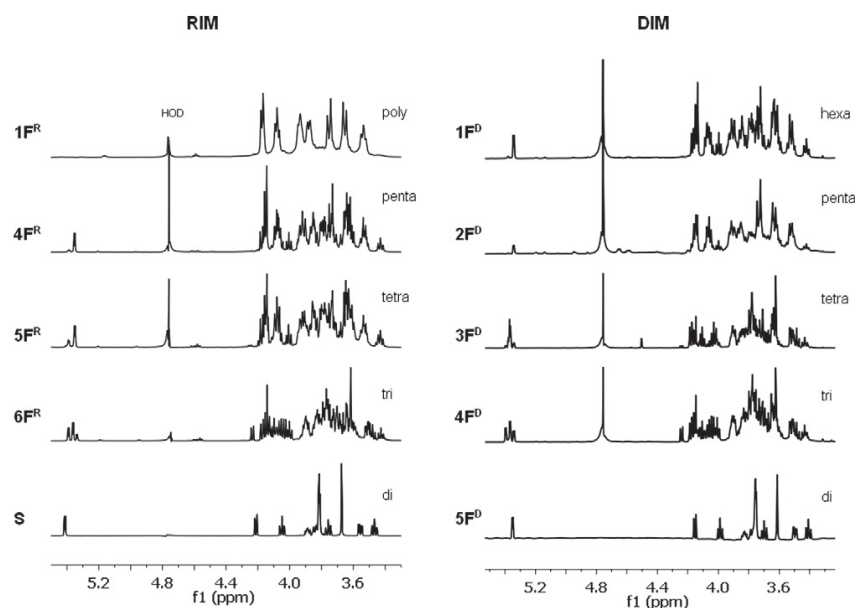
Figure 3. Series of ^1\text{H} NMR spectra of fractions obtained by separation on Bio-Gel P2 of retentate (RIM) and dialyzate (DIM). Fractions 1\text{F}^{\text{R}} and 4\text{--}6\text{F}^{\text{R}} from RIM, fractions 1\text{--}5\text{F}^{\text{D}} from DIM, di—disaccharide, tri—trisaccharide, tetra—tetrasaccharide, penta—pentasaccharide, hexa—hexasaccharide, poly—polymer, HOD—residual signal of water.
