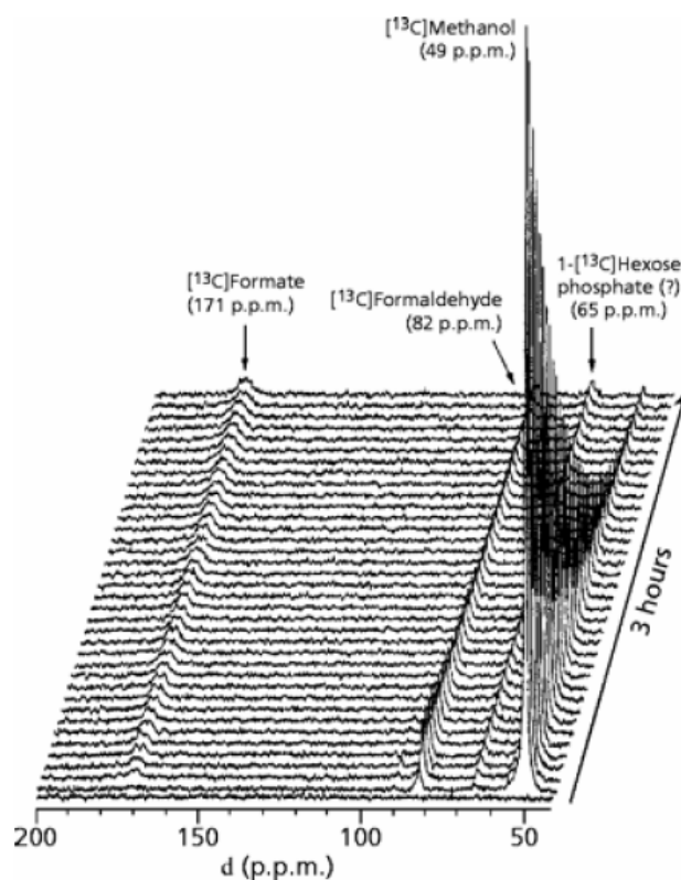
Figure 13. ^{13}\text{C} NMR analysis of the kinetics of ^{13}\text{C} -methanol degradation in a cell suspension of B. methanolicus (Pluschkell and Flickinger, 2002).
