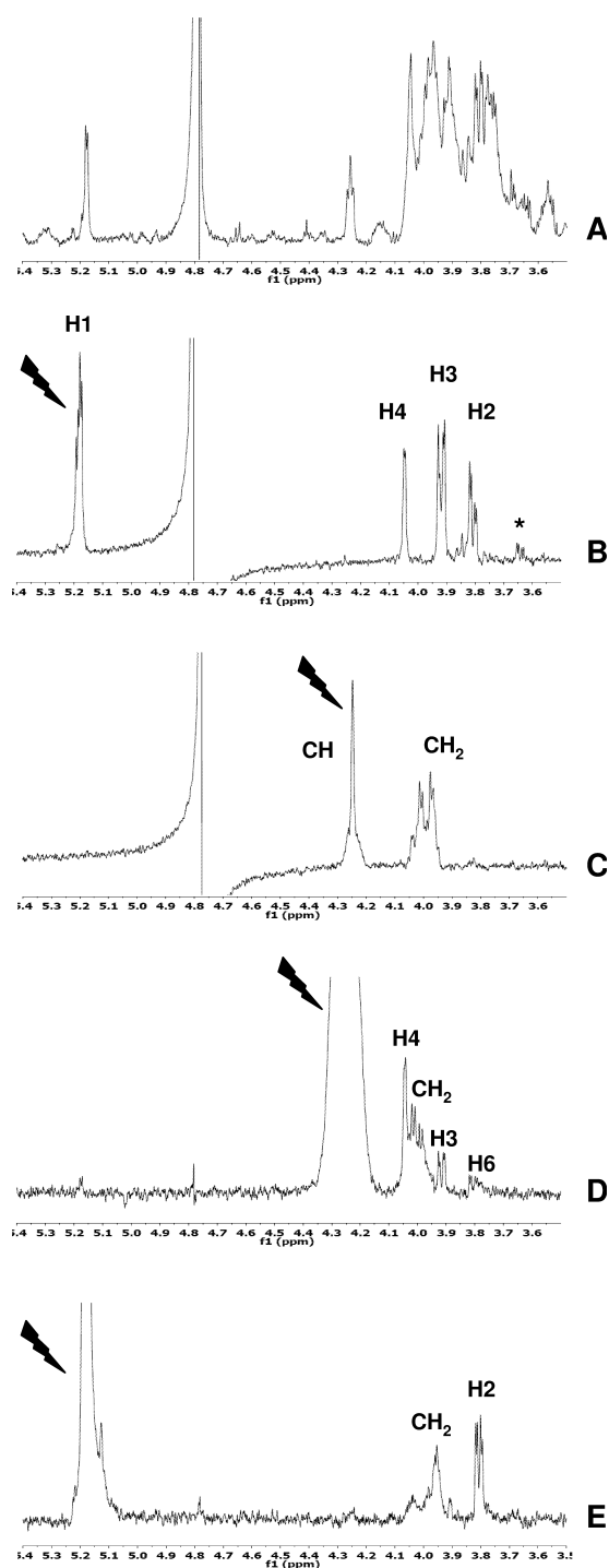
Figure 3. Selective 1D NMR spectra of the incubation medium of Bacillus sp. 3B6 on turanose: ^1\text{H} NMR spectrum of turanose t = 72 h (A); selective 1D TOCSY with mixing time 150 ms spectra with irradiation at \delta 5.176 ppm (B) and \delta 4.245 ppm (C); selective 1D NOESY spectra with mixing time 200 ms with irradiation of the signal at \delta 4.245 (D) and \delta 5.176 (E); * unknown.
