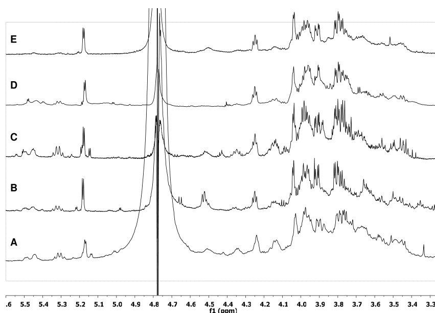
Figure 1. ^1\text{H} NMR spectra of incubation media (IM) of Bacillus sp. 3B6, in which the carbohydrate substrate was already depleted: A ( t = 63 h) on glucose; B ( t = 43 h) on cellotetraose; C ( t = 63 h) on cellulose; D ( t = 72 h) on turanose; and E ( t = 63 h) on starch. In B ( t = 43 h) on cellotetraose still some substrate was present. Similar spectral pattern was observed also in the case of fructose and sucrose at the end of the incubation.
