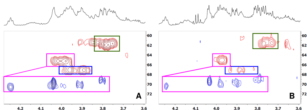
Figure 2. EPSs spectral patterns in HSQC spectra of IM media of Bacillus sp. 3B6 on: A – turanose after 72 h and B – cellulose after 63h. Attribution of colours: i) spectrum cross-peak: red – CH 2 ; blue – CH; ii) marks: pink 1,6-linked \alpha -galactan; green and blue – non identified –O–CH 2 – due to PHA.
