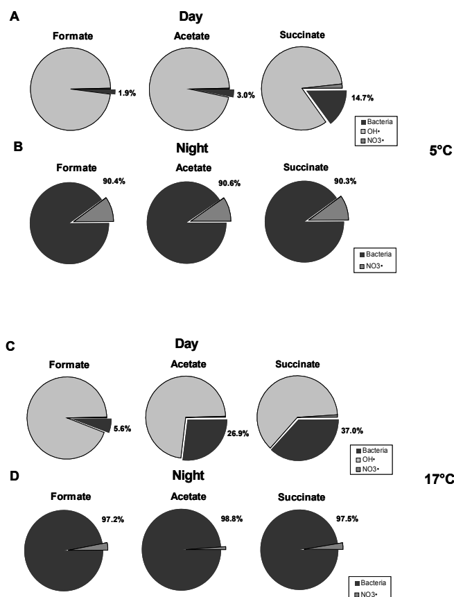
Figure 5. Estimated relative influence of bacterial activity (in black) and free radicals (hydroxyl \cdot\text{OH} and nitrate \text{NO}_3\cdot ) on the degradation of formate, acetate, and succinate in cloud water at 5 °C (A) during the day and (B) during the night and at 17 °C (C) during the day and (D) during the night. During night-time ( i.e. in the absence of photochemical reactivity), \cdot\text{OH} radicals are not present and were not considered. The following values of concentrations have been used for calculations: [bacteria] = 8.4 \times 10^4 cell \text{mL}^{-1} ; [ \cdot\text{OH} ] = 1.2 \times 10^{-13} mol \text{L}^{-1} (day-time); [ \text{NO}_3\cdot ] = 1.5 \times 10^{-14} mol \text{L}^{-1} ; [formate] = 14.5 \times 10^{-6} mol \text{L}^{-1} ; [acetate] = 20 \times 10^{-6} mol \text{L}^{-1} ; [succinate] = 1.5 \times 10^{-6} mol \text{L}^{-1} . (From Väitilingom et al. , 2010).
