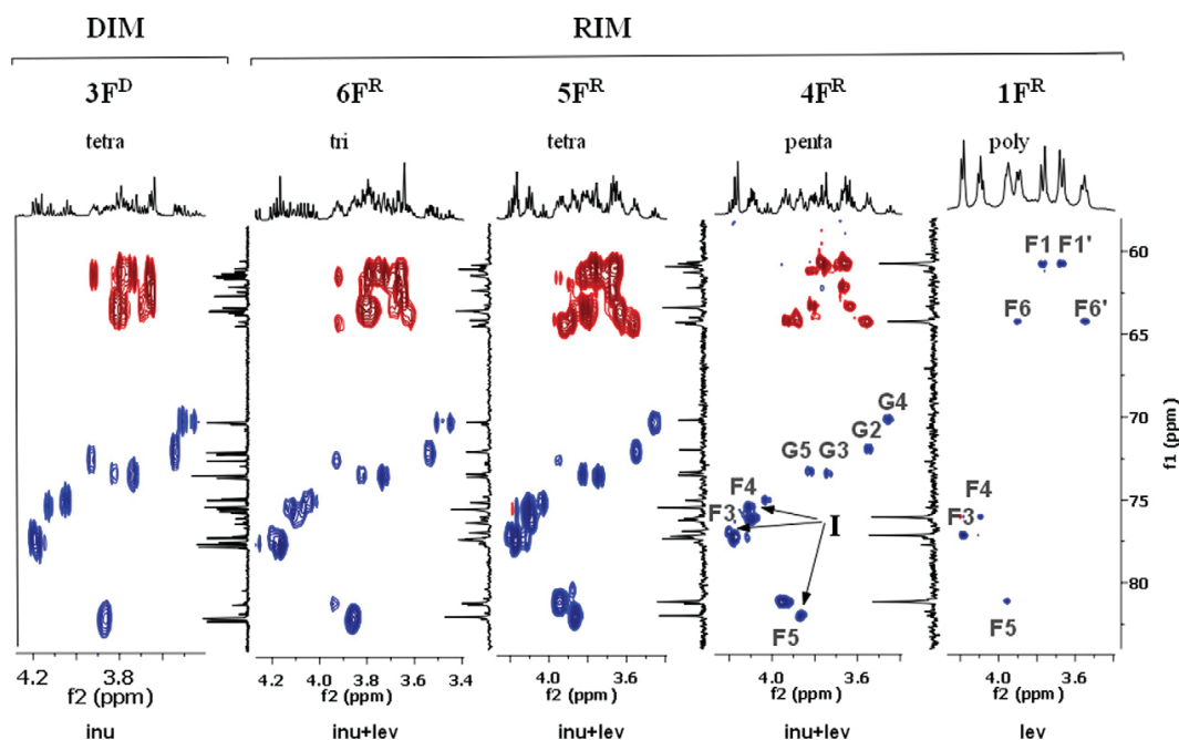
Figure 4. Part of HSQC NMR spectra (cross peaks of skeletal protons and carbons) of chosen fractions obtained by separation on Bio-Gel P2 of retentate (RIM) and dialyrate (DIM). 3F^D tetrasaccharide DIM fraction, 1F^R and 4-6F^R —polymer and tri-, tetra-, and pentasaccharides of RIM, inu—inulin type 1, 2- \beta FOSs, lev—levan type 2,6- \beta FOSs, S—sucrose, G—glucose, F— \beta -fructofuranose, I—cross peaks due to inulin type 1,2- \beta FOSs.
