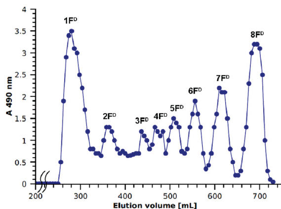
Figure 2. Elution profile on Bio-Gel P2 of the retentate (RIM) obtained after a dialysis of a complex incubation medium (incubation procedure No. 2) retained after 3 days dialysis against water (8 days of incubation of Bacillus sp. 3B6 on sucrose).
