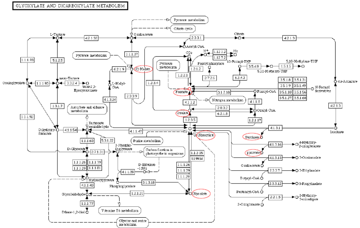
Scheme 3. Metabolic pathways involved in bacterial metabolism. Glyoxalate and dicarboxylate metabolism.
