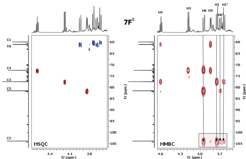
Figure 6. HSQC and HMBC spectra of the disaccharide difructose anhydride DFA IV present in the 7F R fraction obtained after the separation of the dialyzed complex incubation medium RIM (incubation procedure No. 2) on Bio-Gel P2.
