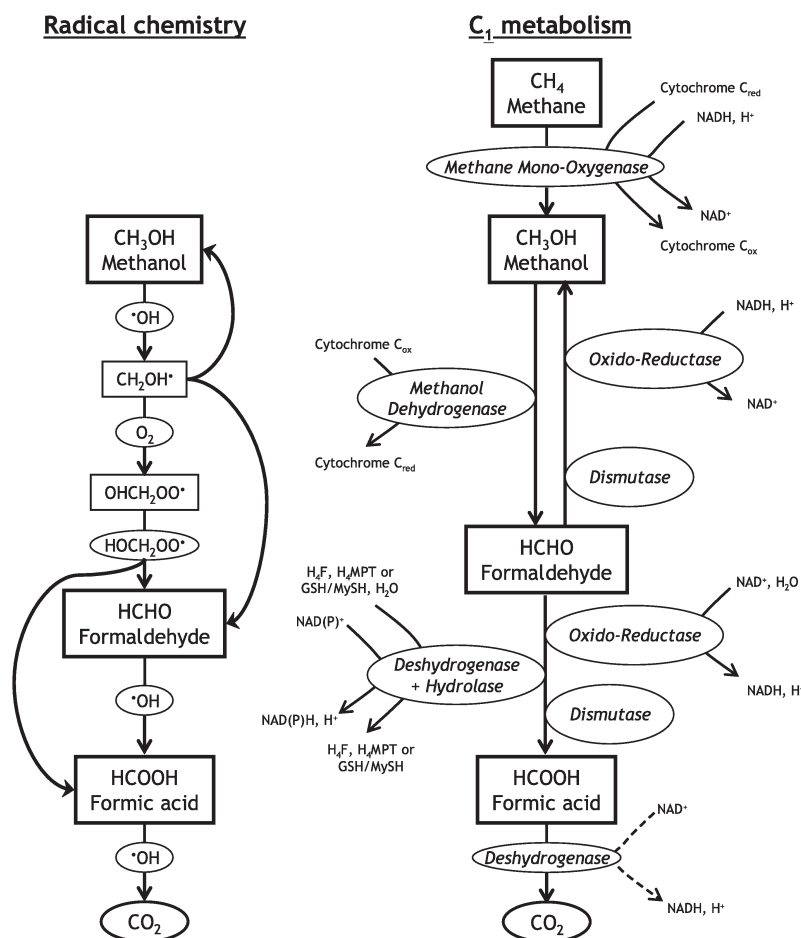
Fig. 1. Non-exhaustive schemes of the ways of degradation of C_1 compounds by radical chemistry and by metabolism. The scheme corresponding to radical chemistry has been drawn from reactions given in Monod et al. (2000) and references therein. C_1 metabolism scheme was reconstructed from Hanson and Hanson (1996), and Delort (2006) and references therein. Known enzymes are described for each reaction in which they can be involved, as well as cofactors when required (the dot line in the case of Formate, dehydrogenase signifies the existence of several types of this enzyme, with and without a cofactor). NAD: Nicotinamide adenine dinucleotide; H_4F : Tetrahydrofolate; H_4MPT : Dephospho-tetrahydro-methanopterin; GSH: Glutathione; MySH: Mycothiol.
