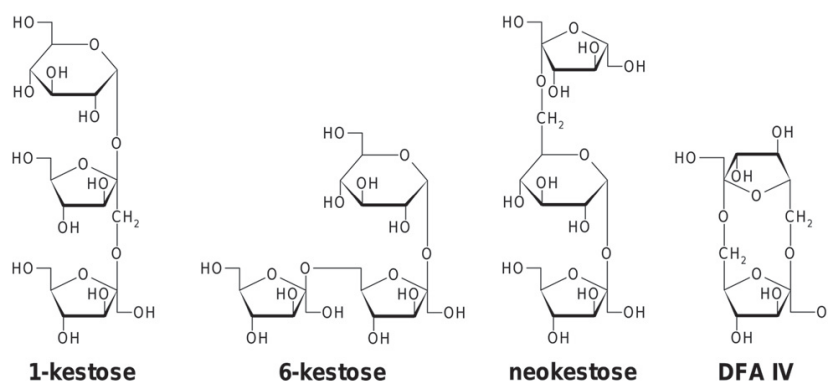
Figure 5. Structures of 1-kestose, 6-kestose, neokestose, and DFA IV.
