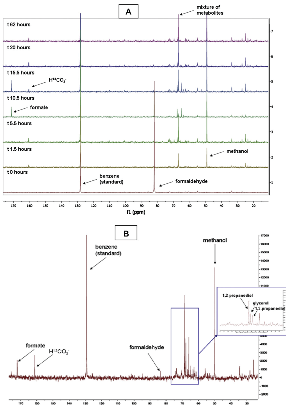
Fig. 2. A) in vivo ^{13}C NMR spectra collected during the incubation of Bacillus sp 3B6 with ^{13}C formaldehyde; B) Example of in vivo ^{13}C NMR spectrum collected after 4 h. Cell concentration was 10^9 cells mL^{-1} and substrate concentration was 20 mM.
