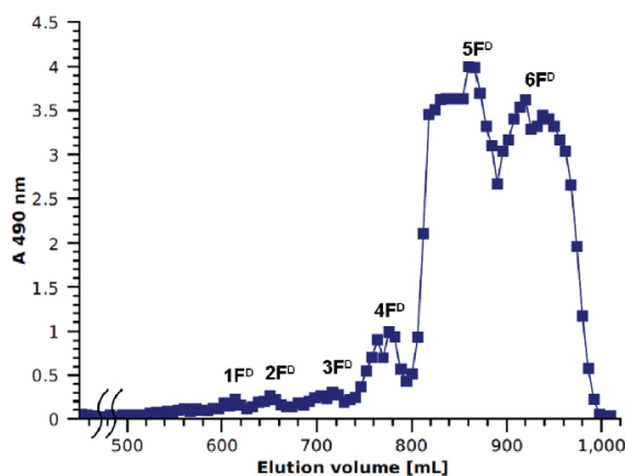
Figure 1. Elution profile on Bio-Gel P2 of the dialyzate (DIM) obtained after a dialysis of a complex incubation medium (incubation procedure No. 2) after 3 days dialysis against water (8 days of incubation of Bacillus sp. 3B6 on sucrose).
