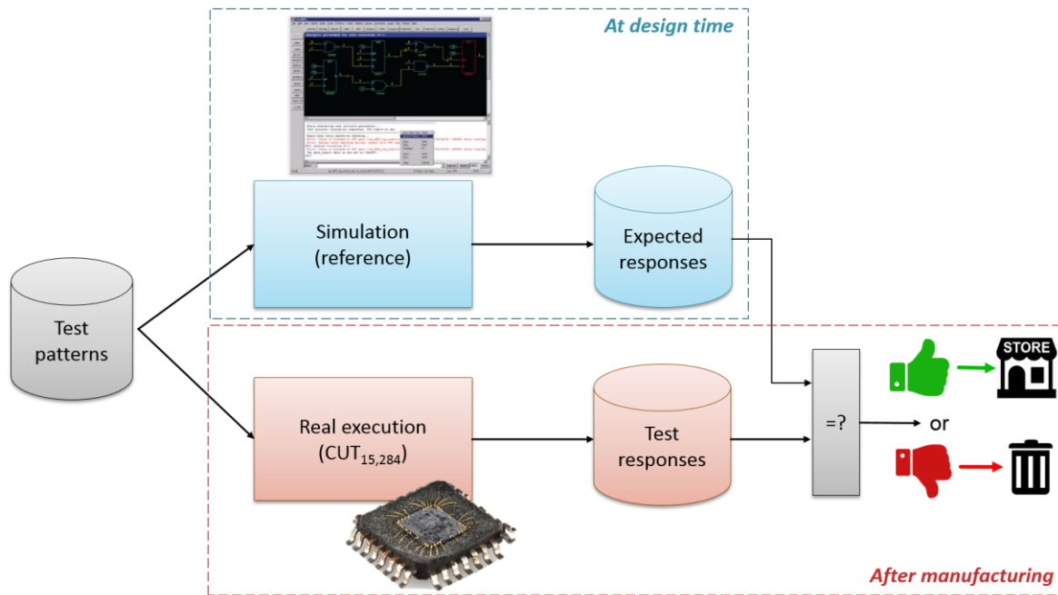
Figure 4: Testing principle.
