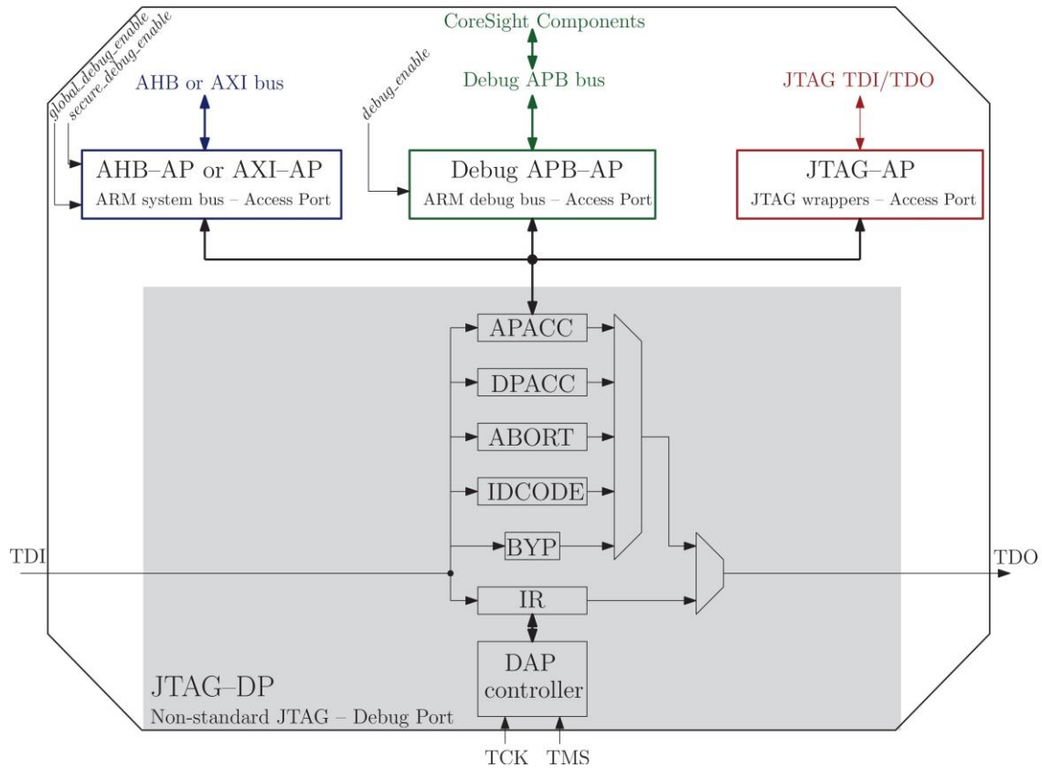
Figure 12: Overview of the non-standard JTAG-Debug Port (JTAG-DP) giving 3 accesses to (1) the ARM system bus (AHB or AXI); (2) the ARM debug bus (Debug APB); and (3) the standard JTAG wrappers.
