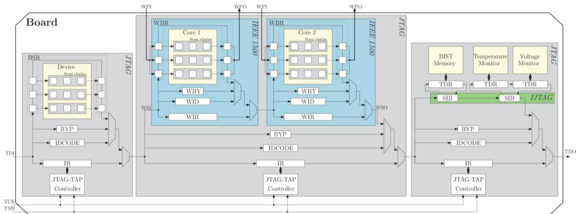
Figure 11: JTAG daisy-chained components and integration with IEEE 1500 (blue area) and IJTAG (green area) standards.
