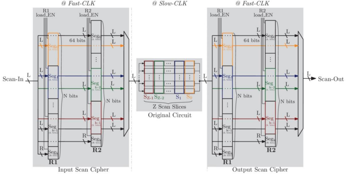
Figure 26: Proposed CBC solution applied on L multiple scan chains.
