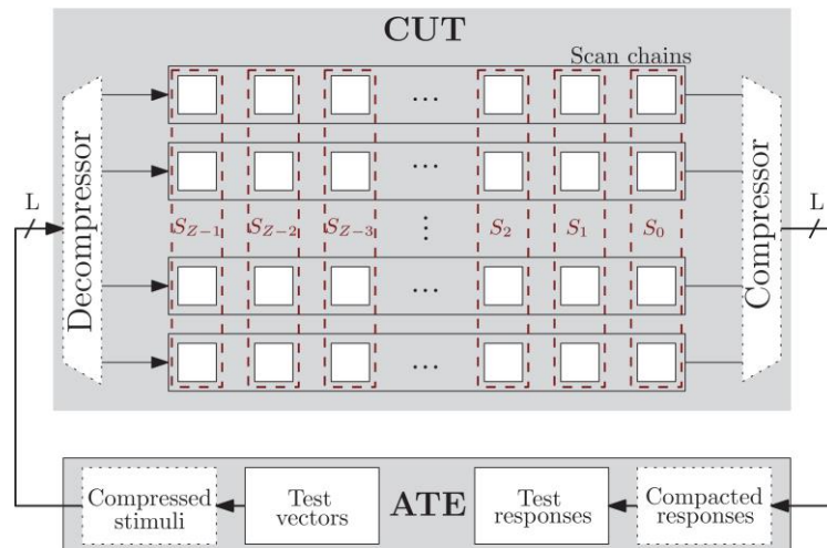
Figure 10: Multiple scan design with the possible integration of test compression techniques.
