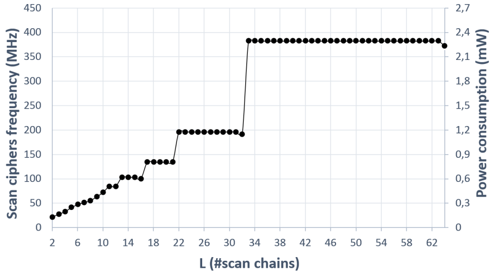
Figure 28: Scan ciphers frequency and power consumption according to the number L of scan chains (in the case of SKINNY block cipher).
