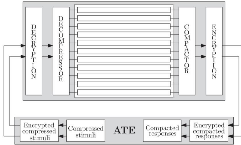
Figure 29: CBC applied when a test compression method is used.
