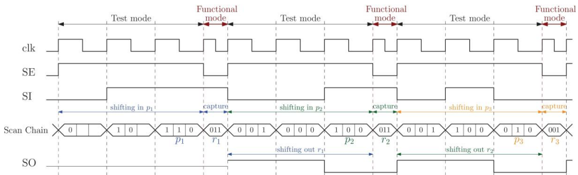
Figure 6: Example of scan procedure for testing stuck-at faults.
