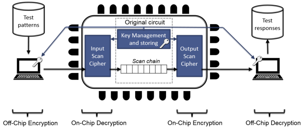
Figure 21: Principle of proposed scan chain encryption.
