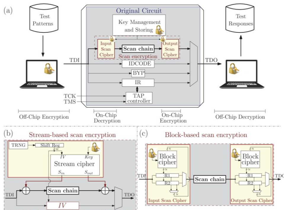
Figure 36: (a) Global architecture of the scan encryption countermeasures. (b) CSC implementation. (c) CBC implementation.
