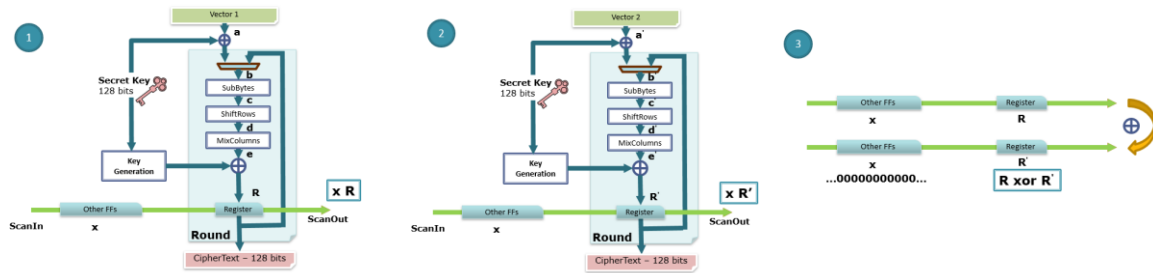
Figure 14: Differential scan attack on AES.
