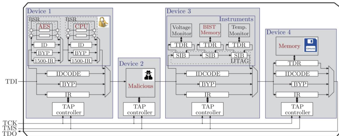
Figure 13: JTAG daisy-chained components (Device 1) a SoC containing an AES crypto-core and a CPU, (Device 2) a malicious core, (Device 3) a device with embedded instruments accessible through an RSN, and (Device 4) a memory contained a firmware.
