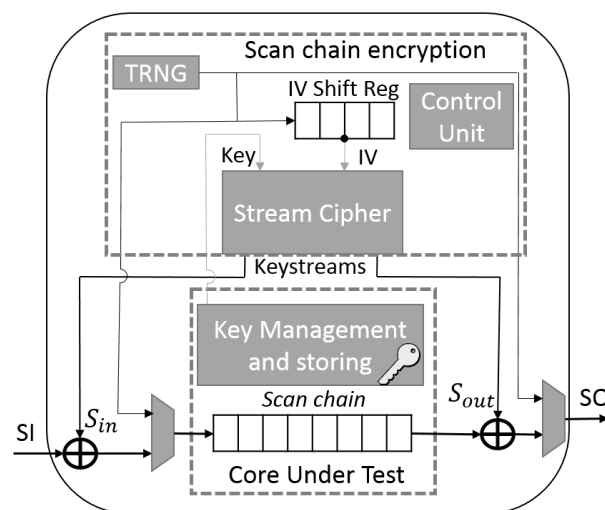
Figure 31: Architecture of the first proposed CSC using a random IV.
