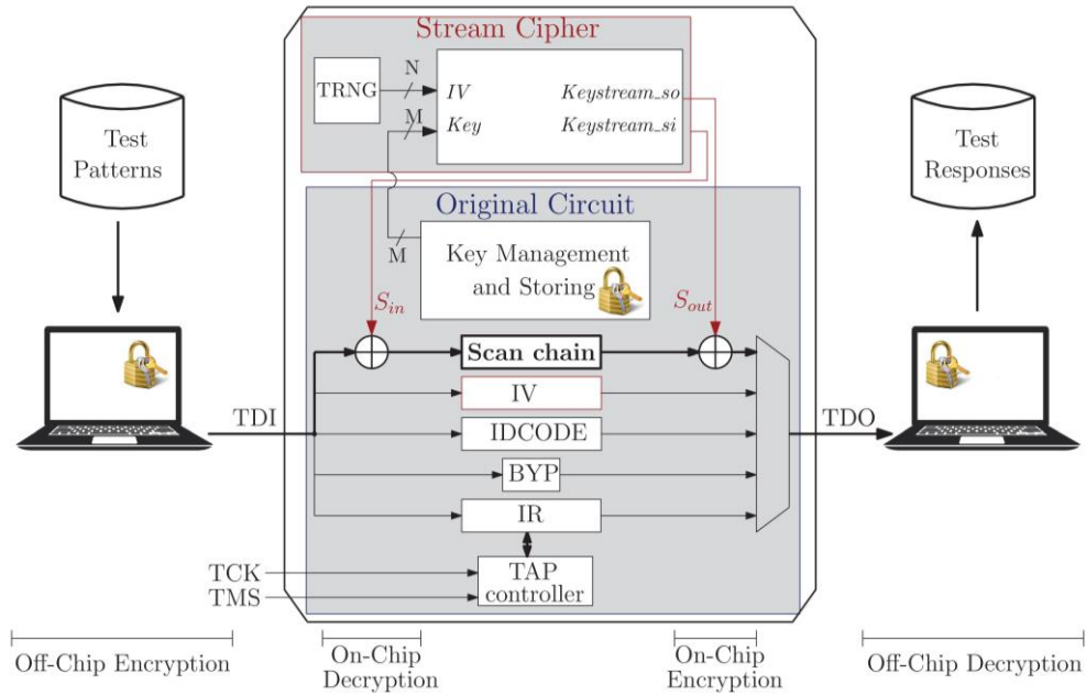
Figure 32: Basic scheme of CSC on single scan chain integrated in JTAG infrastructure.
