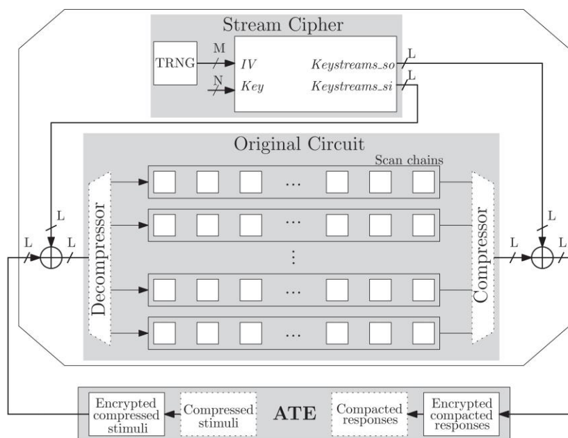
Figure 35: CSC solution applied on L multiple scan chains regardless of test compression.
