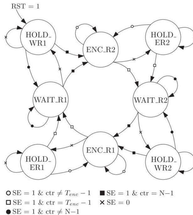
Figure 24: Finite State Machine controlling both scan ciphers in CBC.
