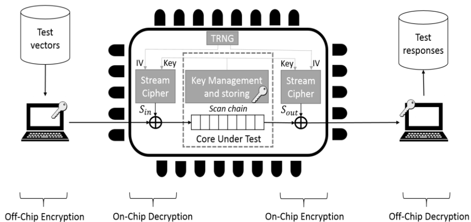
Figure 30: Principle of the proposed CSC using a random IV.
