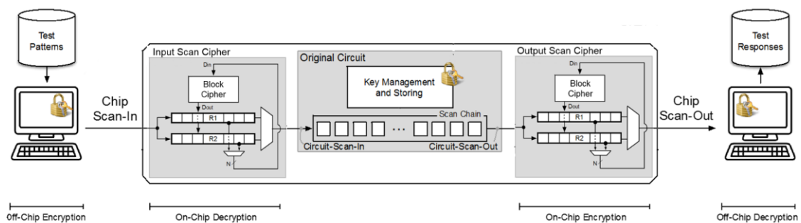
Figure 22: Basic scheme of CBC on a single scan chain configuration.
