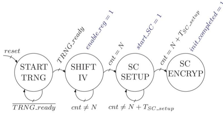
Figure 34: Finite State Machine controlling the initialization procedure of the CSC solution.
