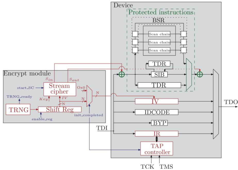
Figure 33: Detailed architecture of the CSC solution.
