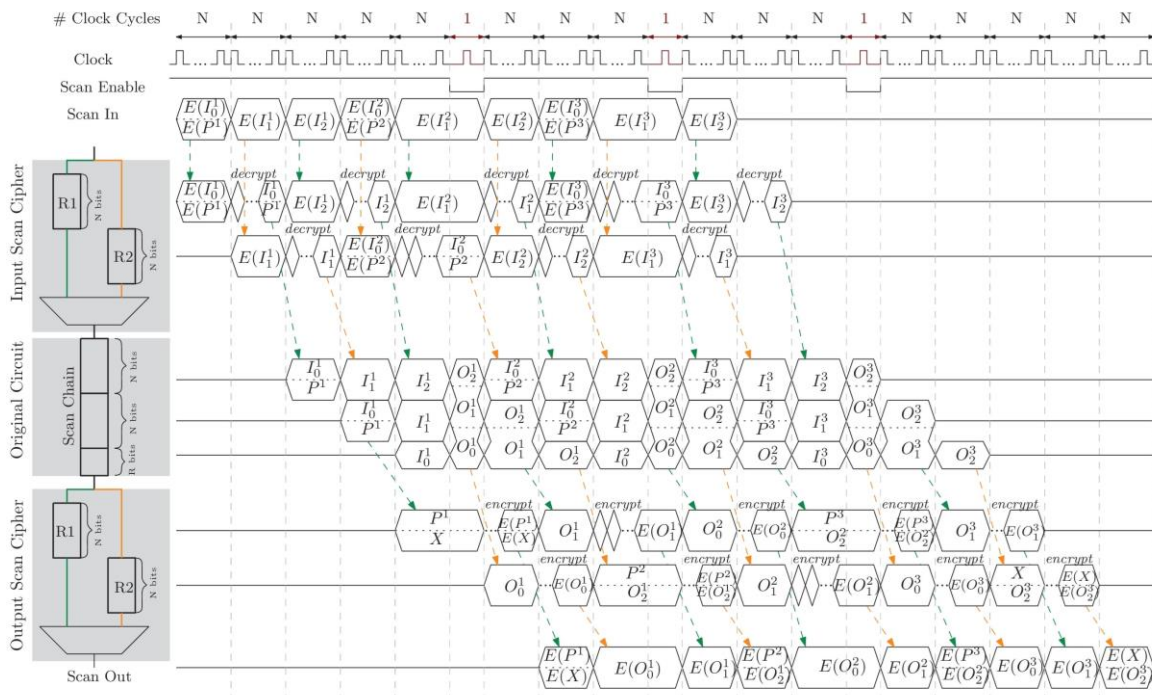
Figure 25: Time diagram of shift operations in the case of CBC applied on single scan chain.
