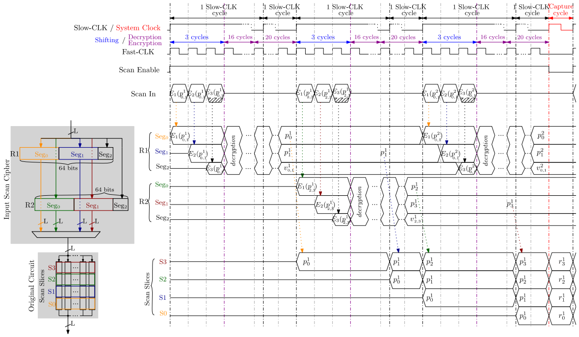
Figure 27: Time diagram of shift operations for the Input Scan Cipher in the case of CBC applied on L multiple scan chains.
