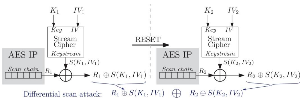
Figure 20: Differential scan attack on test data encrypted with stream cipher.
