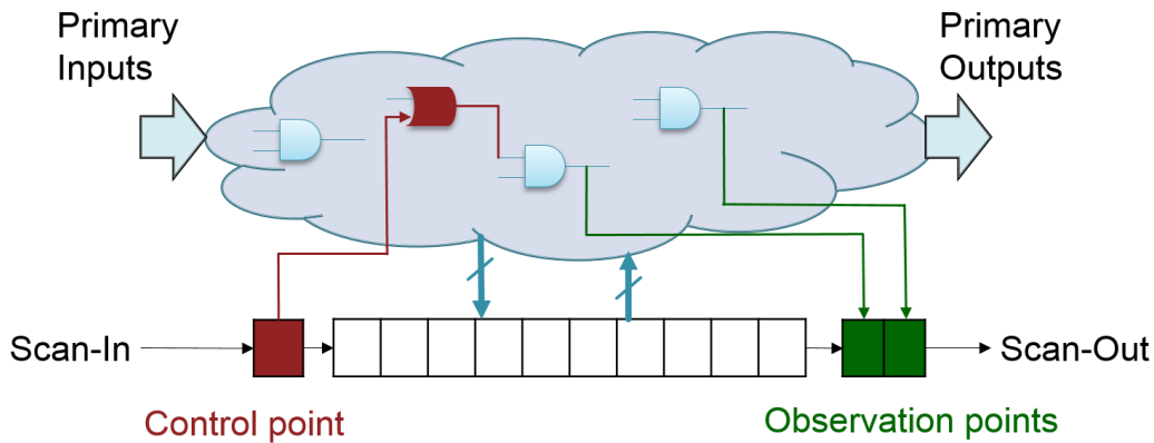
Figure 9: Insertion of control points and observation points on a circuit.
