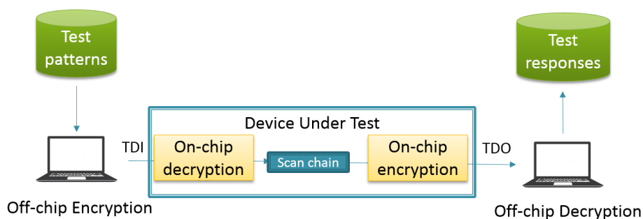
Figure 19: Scheme of test communication encryption.
