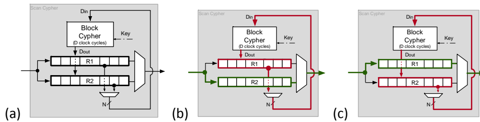
Figure 23: (a) generic scheme of scan cipher; (b) R1 is used for encryption while R2 shifts test data; (c) R2 is used for encryption while R1 shifts test data.
