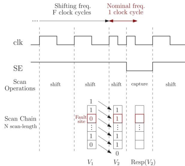
Figure 8: Launch-On Extra-Shift (LOES) scheme.
