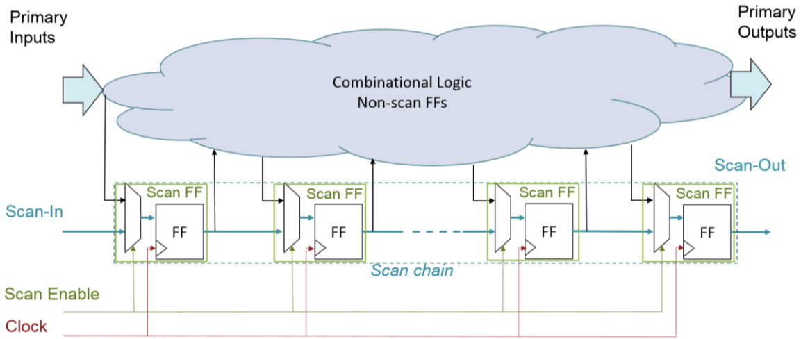
Figure 5: Single scan chain.
