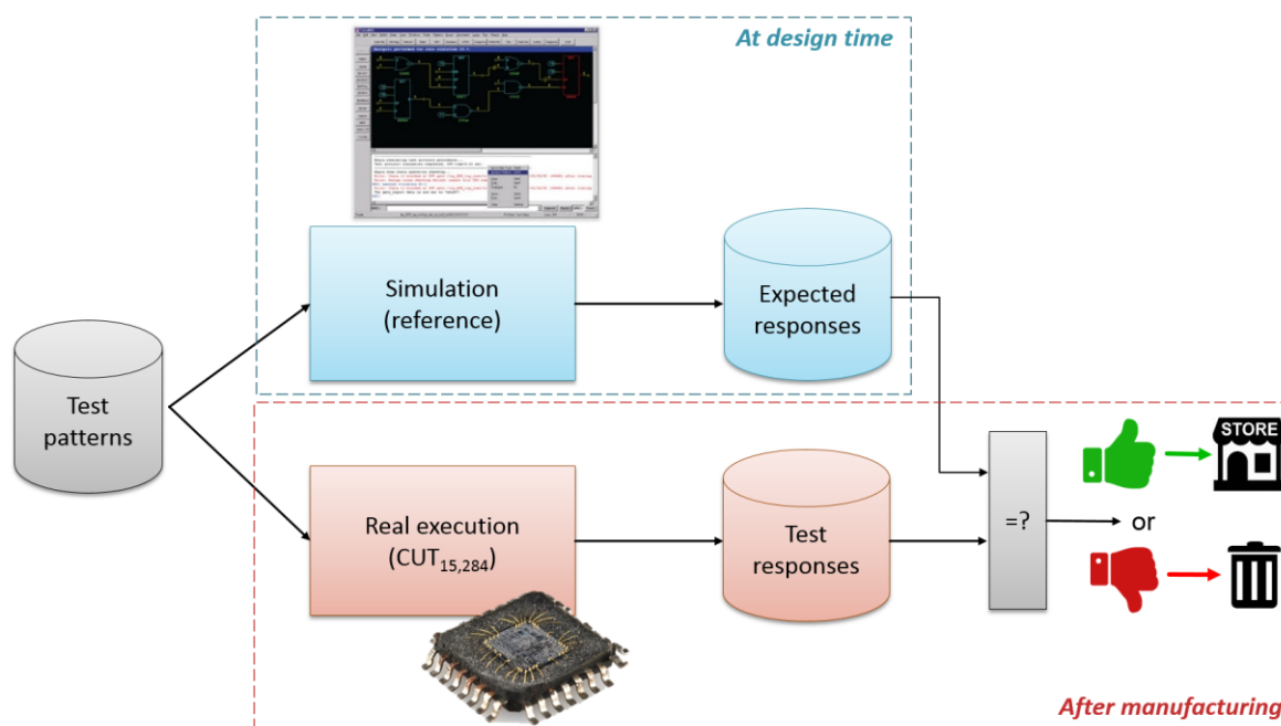
Figure 4: Testing principle.
