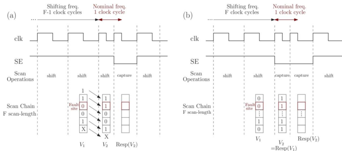
Figure 7: (a) Launch-On-Shift (LOS) scheme. (b) Launch-On-Capture (LOC) scheme.
