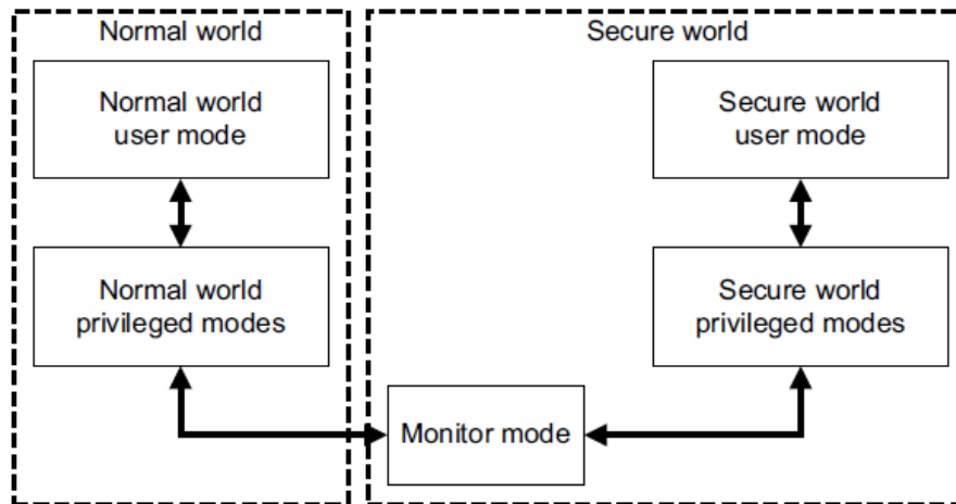
Figure 2: Modes in an ARM processor implementing TrustZone [1] technology.
