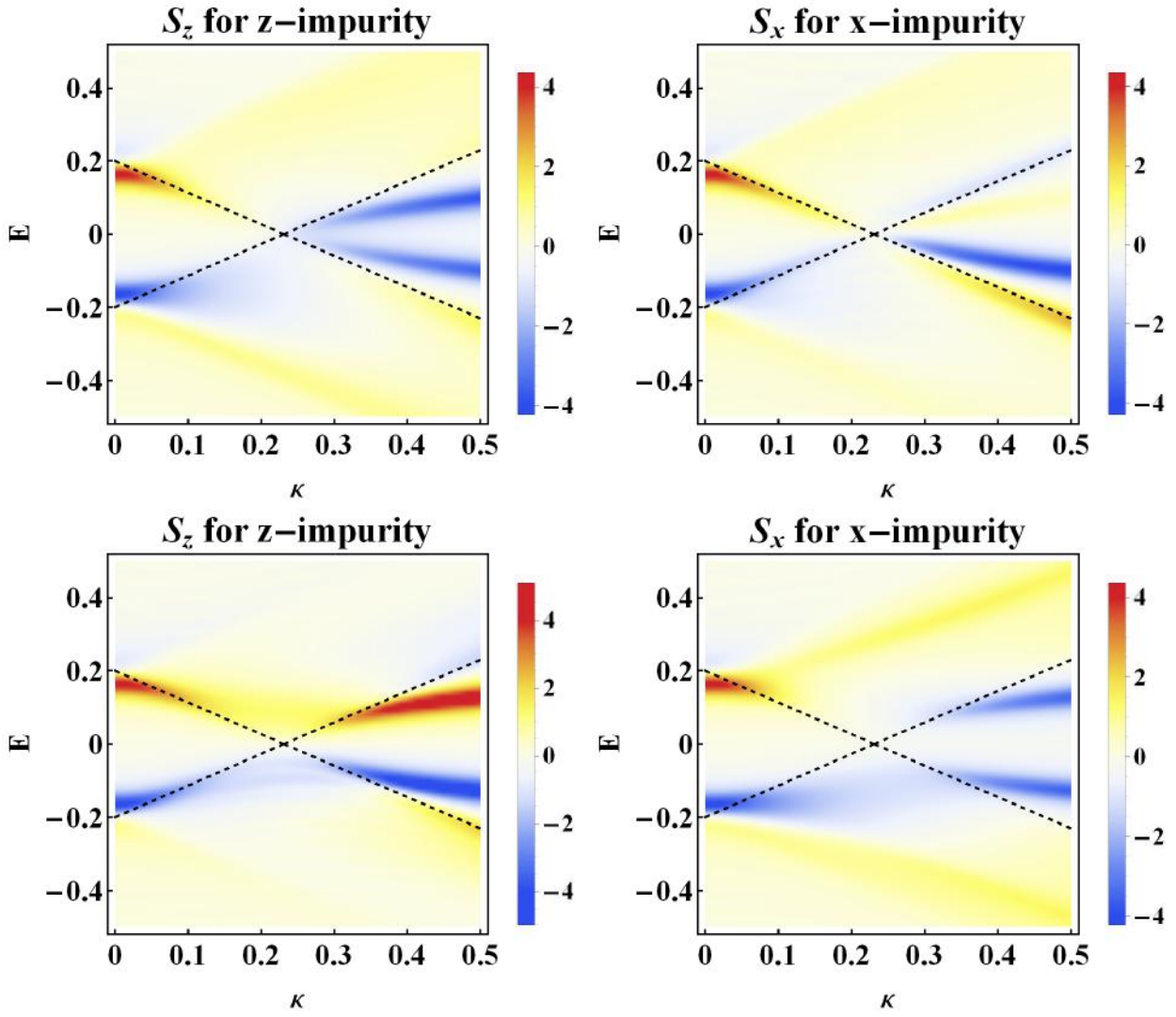
Figure A.4: SPDOS as a function of energy and the p-wave order parameter \varkappa . The \mathbf{d} vector is in-plane in the first row and perpendicular to the plane in the second row. We consider magnetic impurities with an impurity strength of J_z = 6 (left column), and with J_x = 6 (right column). We set \Delta_s = 0.2 , and an inverse quasiparticle lifetime of \delta = 0.03 .
