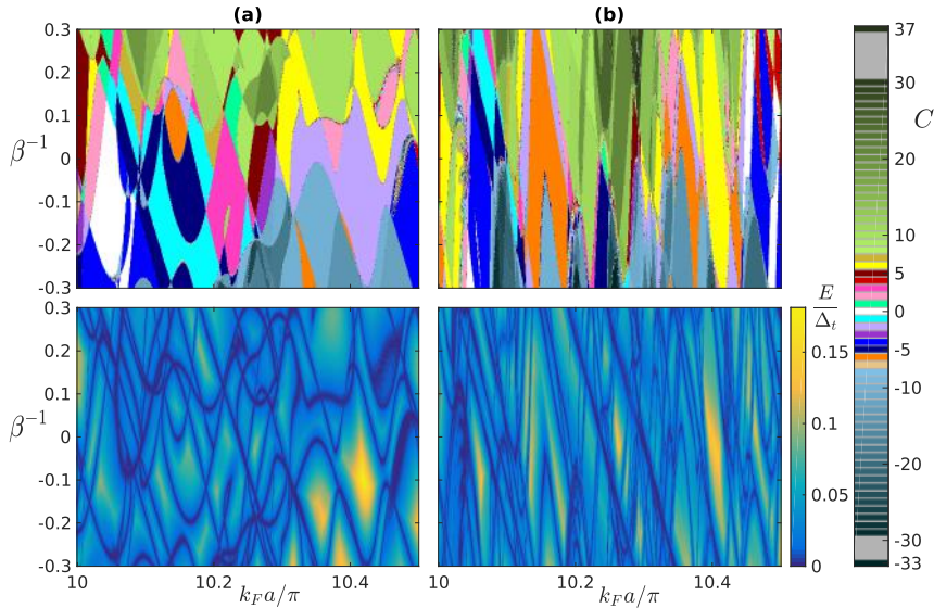
Figure 7.2: (a): Chern number (above) and energy gap (below) diagrams for a square lattice of impurities with lattice constant a and coherence length \xi/a = 5 . The quantity \beta^{-1} in the vertical axis controls the strengths of the impurity. The \beta^{-1} = 0 line, corresponding to infinite impurity potential |U| = \infty , divides the repulsive and attractive impurity regions. The horizontal axis k_F a controls the hybridisation between the bound states centred at different impurity sites. (b): Same as (a) but for coherence length \xi/a = 10 .
