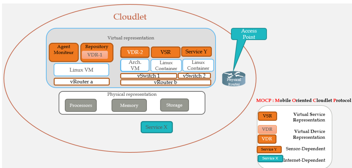
Figure 2.2 Architecture locale d'une Cloudlet
