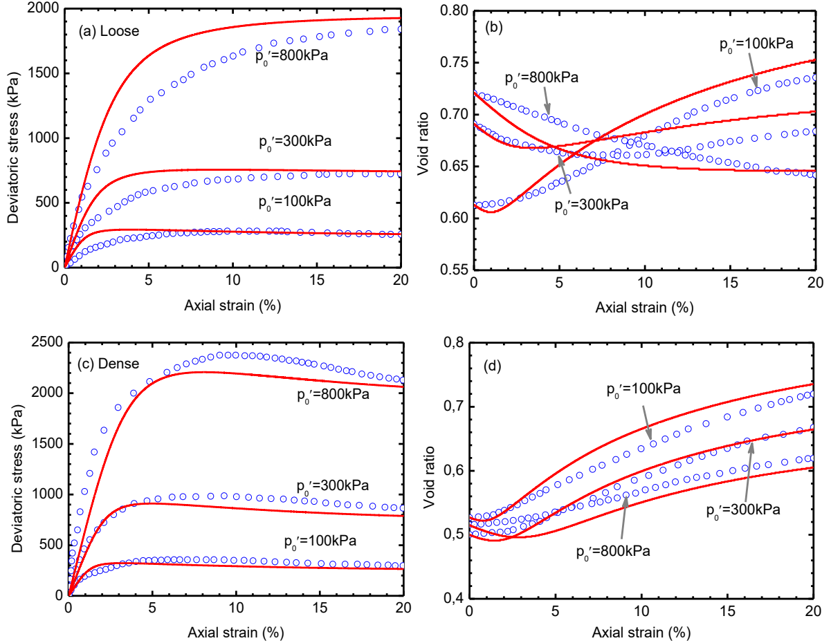
Figure 2.2 Experimental data and simulations for Hostun sand: triaxial drained tests (a) deviatoric stress versus axial strain for loose sand, (b) void ratio versus axial strain for loose sand, (c) deviatoric stress versus axial strain for dense sand, (d) void ratio versus axial strain for dense sand. (experimental data from Biarez and Hicher, 1994)
