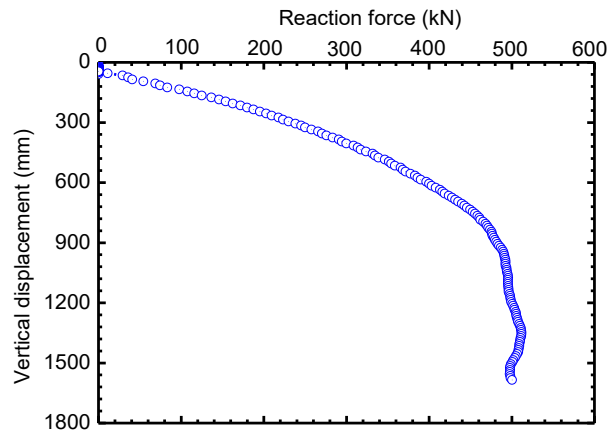
Figure 6.6 Force-displacement relation of the square footing
