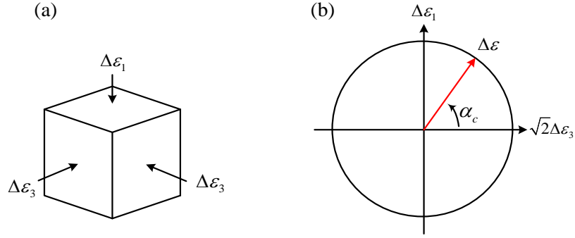
Figure 5.1 Rendulic plane: (a) triaxial probe, (b) strain probe circle
