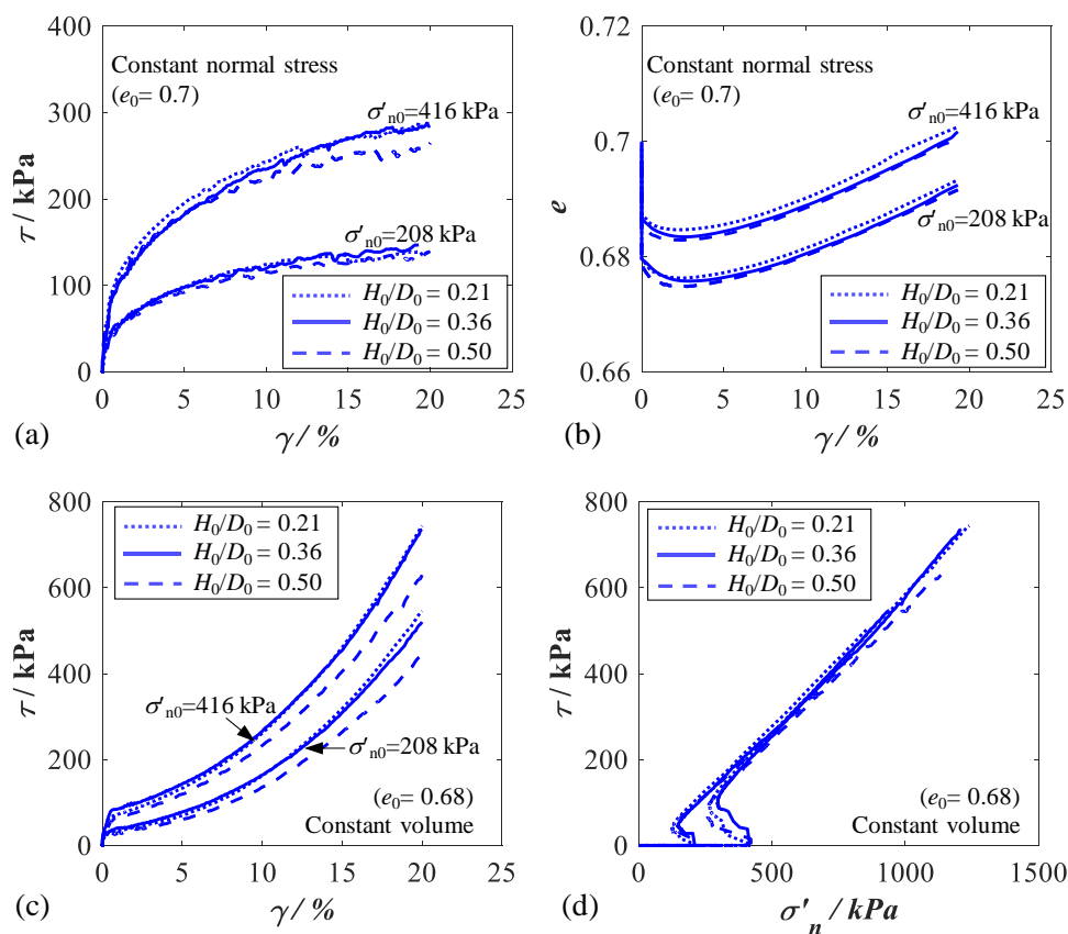
Figure 3.17 Comparison results between different aspect ratios of specimens: (a) constant normal stress simple shear in \gamma - \tau space; (b) constant normal simple shear in \gamma - e space; (c) constant volume simple shear in \gamma - \tau space; (d) constant volume simple shear in \sigma'_n - \tau space.
