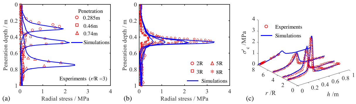
Figure 6.20 Comparison of radial stress between test and simulation considering (a) different penetration depth, (b) different radial distance, and (c) combined 3D plot
