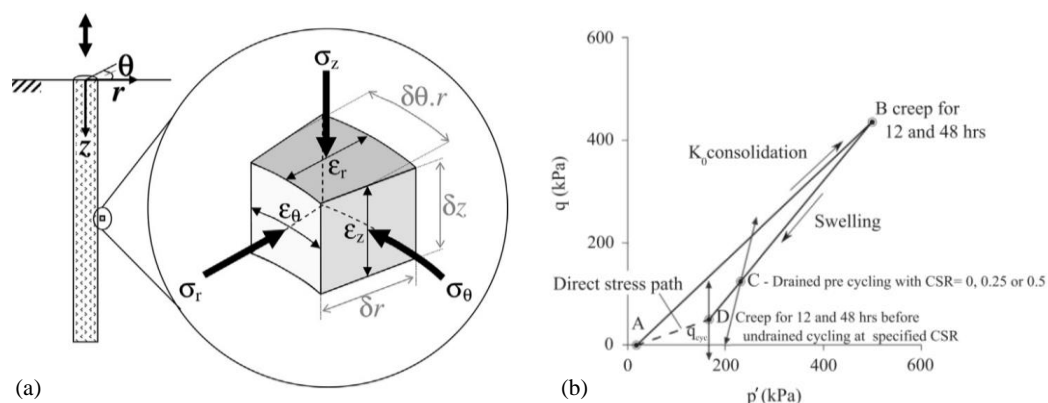
Figure 1.1 Schematic diagram (a) soil element around pile, (b) specimen loading path after (Sim et al. 2013a; Aghakouchak et al. 2015)
