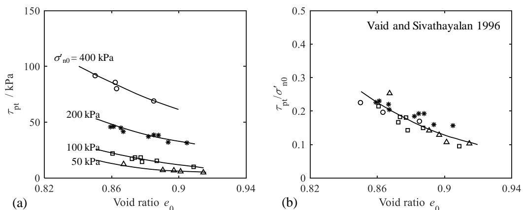
Figure 1.12 Variation of undrained strength at stress with void ratio and initial effect normal stress in simple shear (a) \tau_{pt} versus e ; (a) \tau_{pt}/\sigma'_{n0} versus e (Vaid and Sivathayalan 1996)
