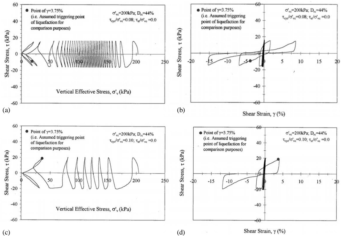
Figure 1.15 Undrained cyclic simple shear tests with different CSRs (a) \sigma'_{n0} versus \tau on CSR=0.08; (b) \gamma versus \tau on CSR=0.08; (c) \sigma'_{n0} versus \tau on CSR=0.1; (d) \gamma versus \tau on CSR=0.1
