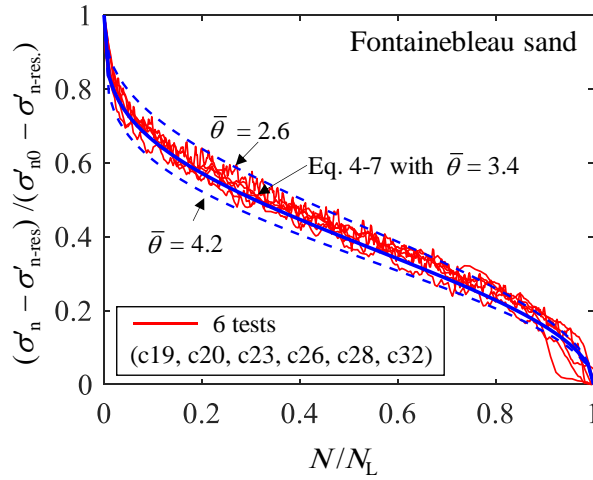
Figure 4.13 Normalized effective normal stress against normalized number of cycles to liquefaction
