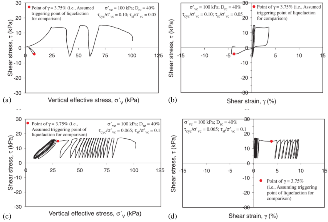
Figure 1.16 Undrained non-symmetrical cyclic simple shear tests with different average shear stress, (a-b) with stress reversal cyclic loading; (c-d) non-stress reversal cyclic loading
