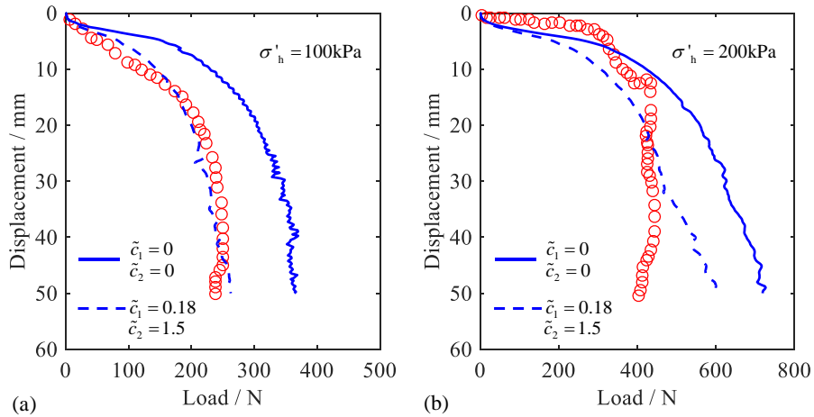
Figure 6.14 Comparison between experiment and simulation of 3SR mini model pile test with confining pressure of (a) 100kPa and (b) 200kPa
