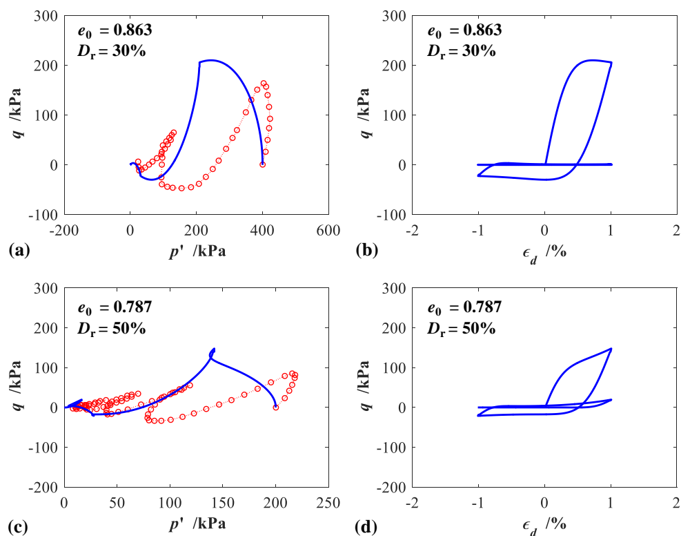
Figure 6.4 Comparison between the experimental and numerical results of undrained triaxial tests under cyclic loading on Toyoura sand with different initial void ratios: in (a) and (c) stress path in mean effective stress versus deviatoric stress; (b) and (d) deviatoric stress versus deviatoric strain
