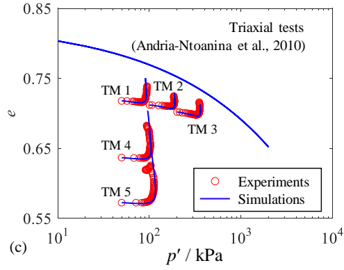
Figure 3.1 Parameters determination from isotropic compression and triaxial drained tests on Fontainebleau NE34 sand: (a) isotropic compression line, (b) deviatoric stress versus axial strain, and (c) void ratio versus mean effective stress
