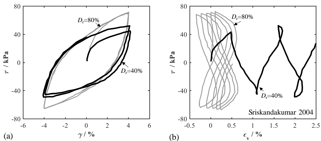
Figure 1.14 Cyclic drained simple shear test on Fraser River sand by Sriskandakumar (2004)
