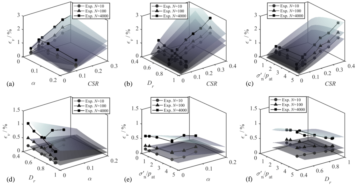
Figure 5.9 Volumetric strain accumulation evolution with 10, 100 and 4000 cycles for different effects of (a) \alpha and CSR , (b) D_r and CSR , (c) \sigma'_n/p_{at} and CSR , (d) D_r and \alpha , (e) \sigma'_n/p_{at} and \alpha and (f) \sigma'_n/p_{at} and D_r
