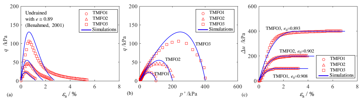
Figure 3.3 Simulation results of triaxial undrained tests on very loose Fontainebleau sand: (a) deviatoric stress versus axial strain; (b) deviatoric stress versus mean effective stress for undrained tests; (c) pore pressure versus axial strain for undrained
