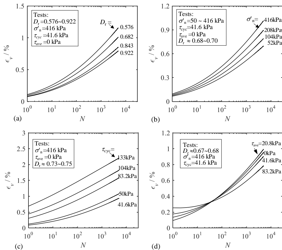
Figure 5.7 Performance of analytical model: (a) calibration with different relative densities; (b) calibration with different effective normal stresses; (c) calibration with different cyclic shear stress; (d) calibration with different average shear stress
