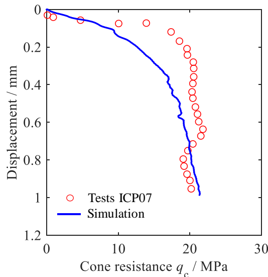
Figure 6.19 Comparison between experiment and simulation of model pile test in Fontainebleau sand for the pile resistance against the penetration depth
