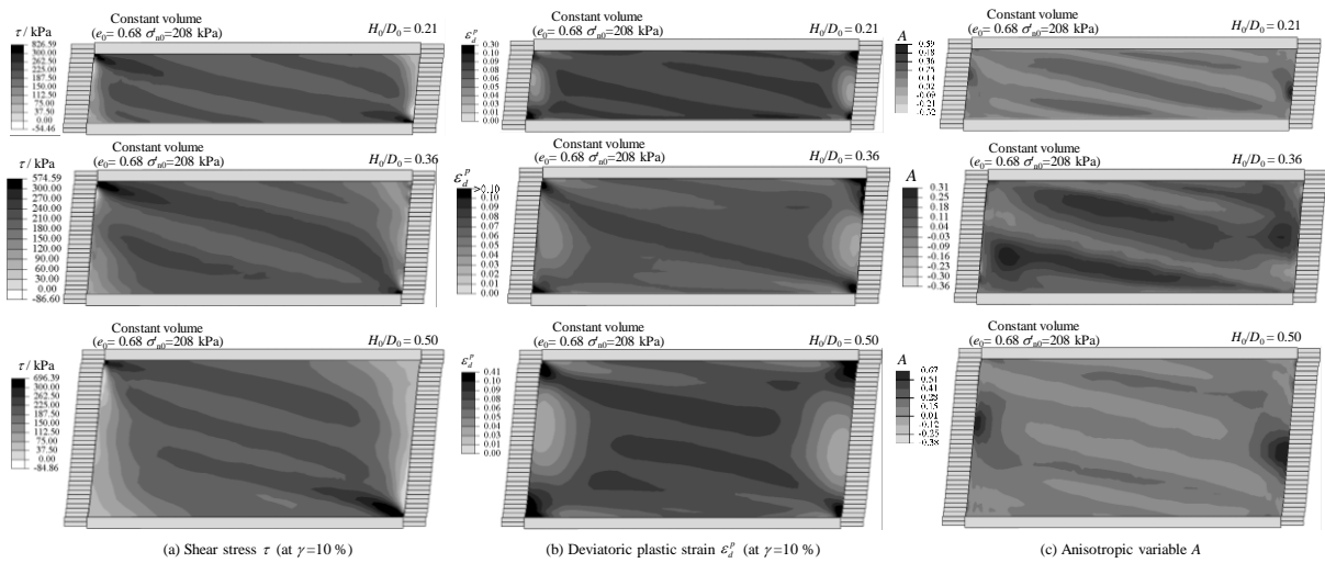
Figure 3.20 Comparisons of different aspect ratios of specimens for the constant volume condition (test S-4): (a) contour of shear stress at \gamma = 10\% , (b) contour of deviatoric plastic strain \varepsilon_d^p at \gamma = 10\% , (c) contour of Anisotropic variable A at \gamma = 10\%
