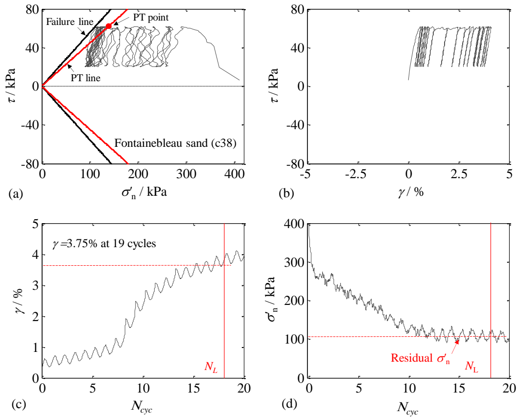
Figure 4.8 Non-symmetrical cyclic response of Fontainebleau sand with no-stress reversal loading: (a) shear stress versus effective normal stress; (b) shear stress versus shear strain, (c) shear strain versus number of cycles; (d) effective normal stress versus number of cycles
