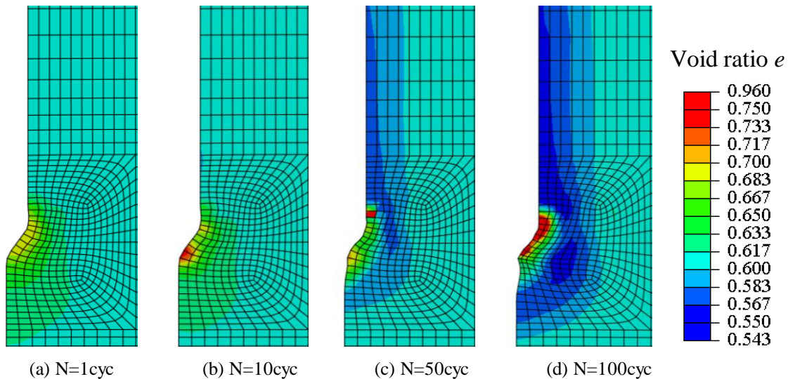
Figure 6.26 Cyclic densification behaviour surrounding the pile with different number of cycles (a) N=1 cycle, (b) N=10 cycles, (c) N=50 cycles and (c) N=100 cycles
