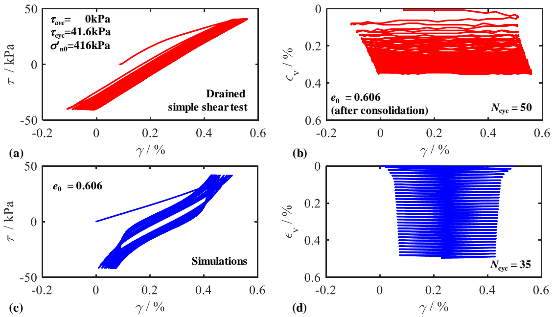
Figure 6.11 Comparison of experimental and numerical results of stress-controlled drained cyclic simple shear tests on medium dense Fontainebleau sand: (a-b) experiment and (c-d) simulation
