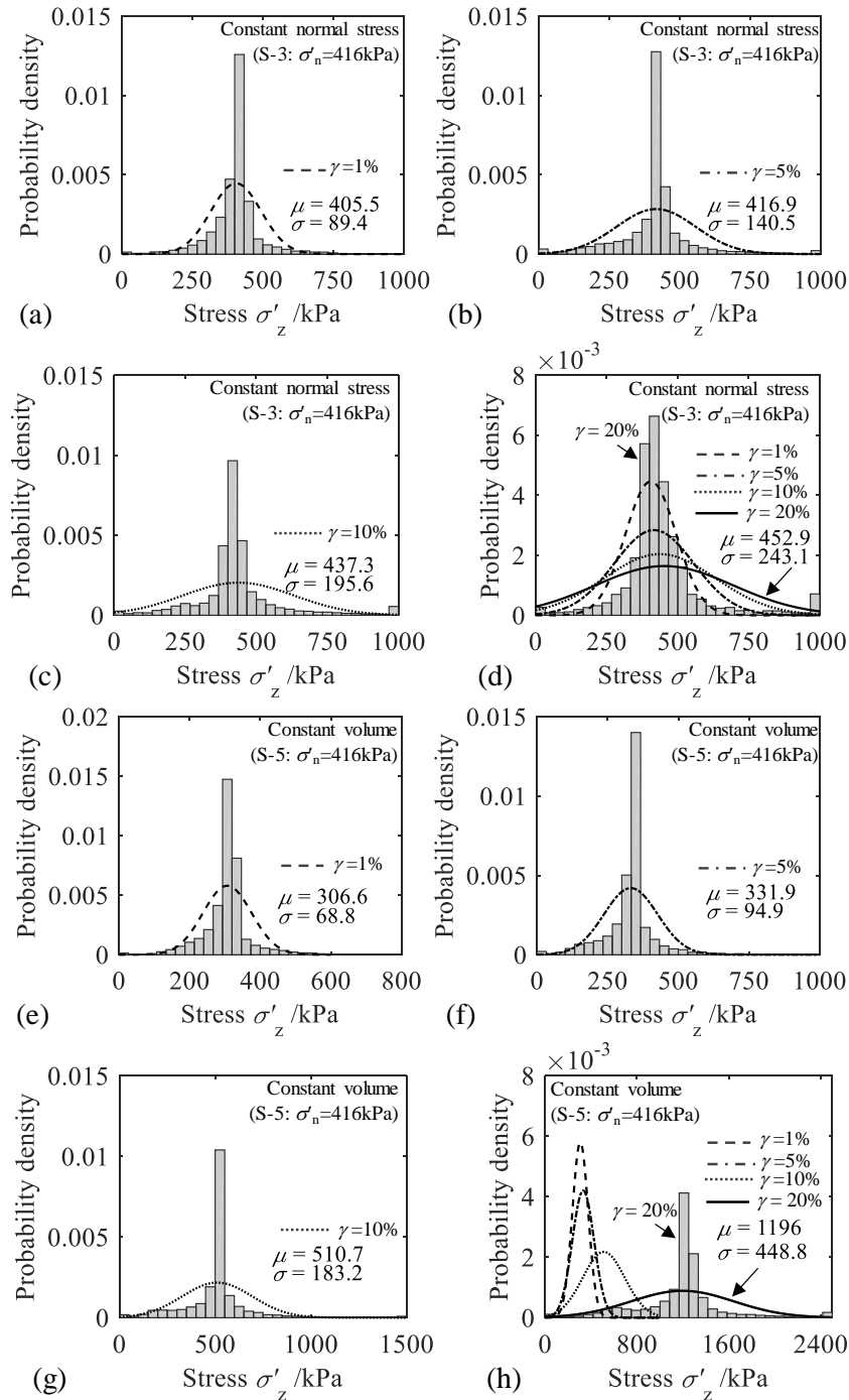
Figure 3.12 Normal distribution of vertical stress \sigma'_z with constant normal stress condition (a) \gamma=1\% , (b) \gamma=5\% , (c) \gamma=10\% and (d) \gamma=20\% ; and with constant volume condition (e) \gamma=1\% , (f) \gamma=5\% , (g) \gamma=10\% and (h) \gamma=20\% .
