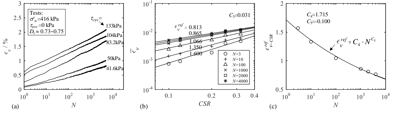
Figure 5.5 volumetric strain accumulation with different cyclic stress ratio: (a) volumetric strain versus number of cycles; (b) normalized volumetric strain versus cyclic shear stress ratio; (c) reference volumetric strain versus number of cycles
