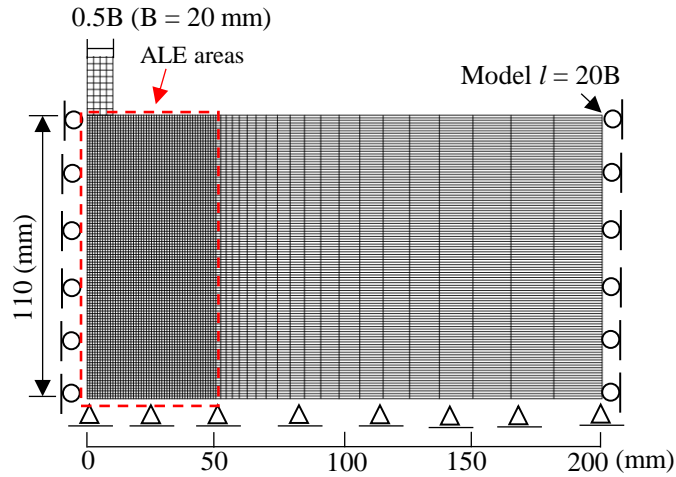
Figure 2.17 Finite element model for footing tests by ABAQUS
