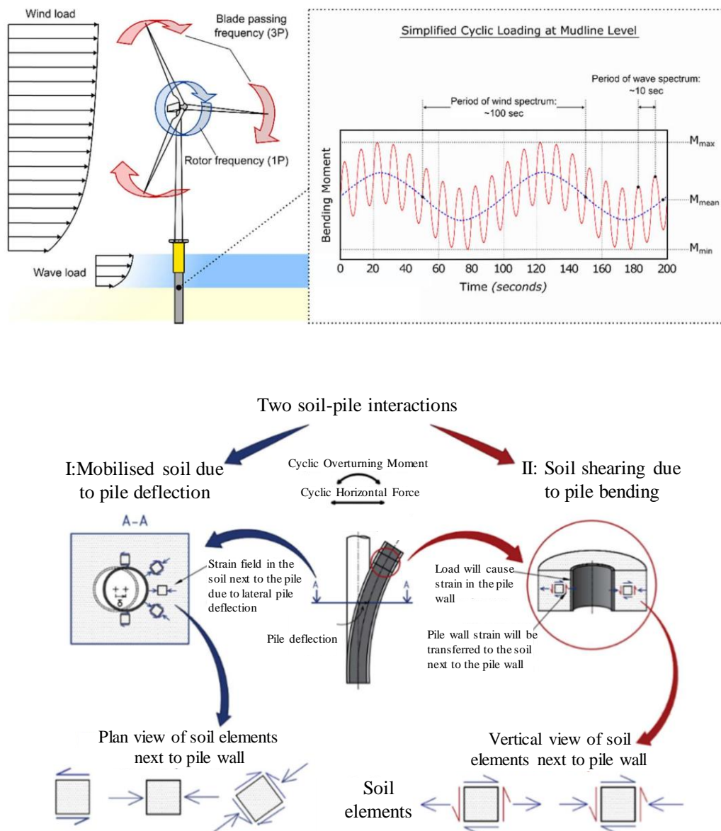
Figure 1.6 Offshore wind foundation and its schematic diagram of loads (Nikitas et al. 2017)
