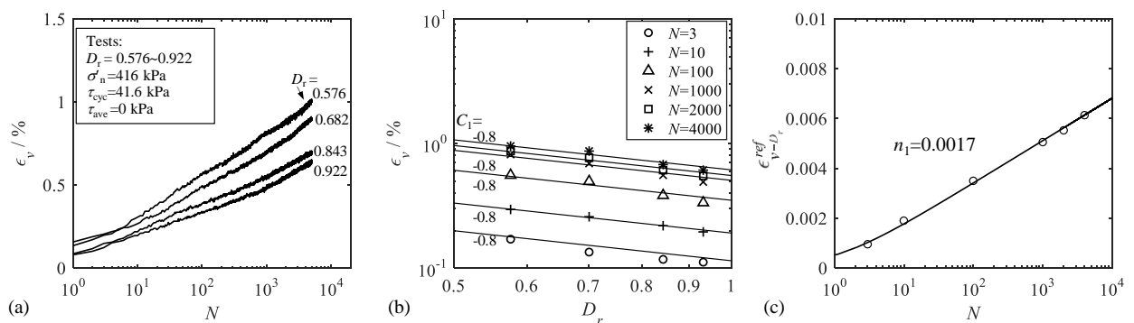
Figure 5.3 volumetric strain accumulation with different relative densities: (a) volumetric strain versus number of cycles; (b) volumetric strain versus relative density; (c) reference volumetric strain versus number of cycles
