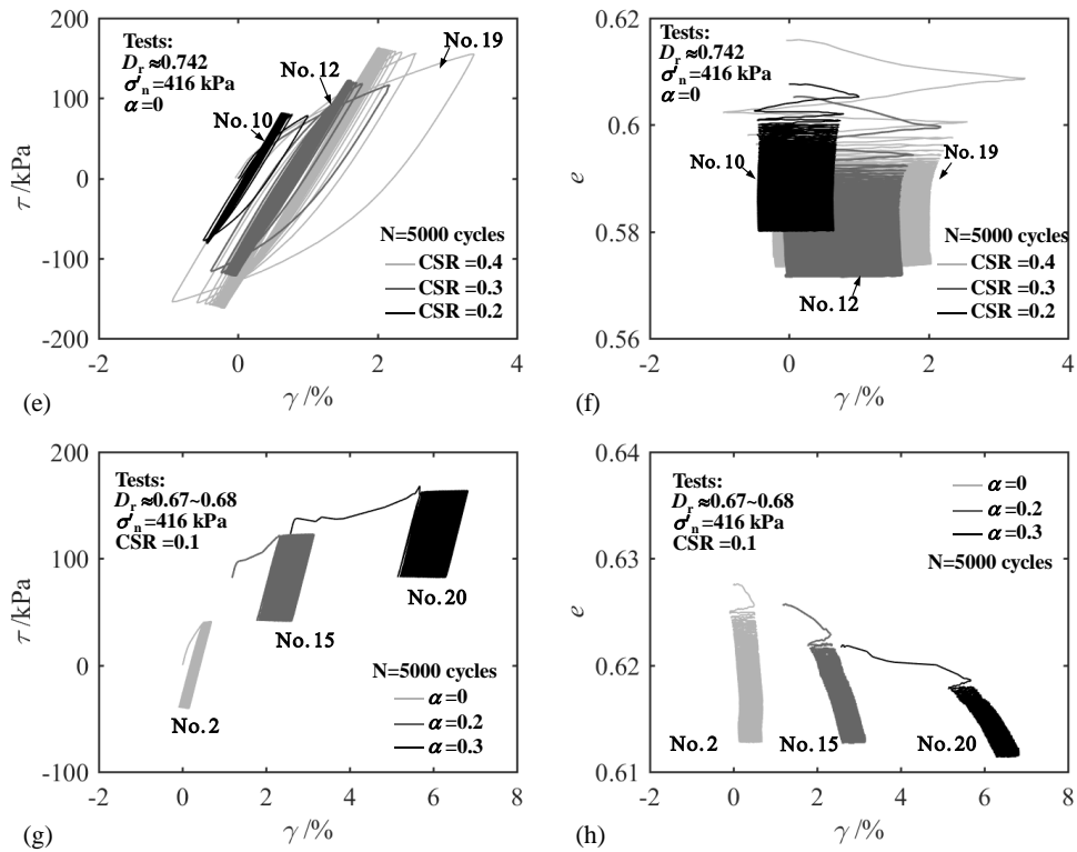
Figure 5.1 Summary of drained cyclic simple shear results: (a)-(b) comparisons by different initial relative densities; (c)-(d) comparisons by different effective normal stresses; (e)-(f) comparisons by different cyclic shear stress ratios and (g)-(h) comparisons by different average shear stress ratios.
