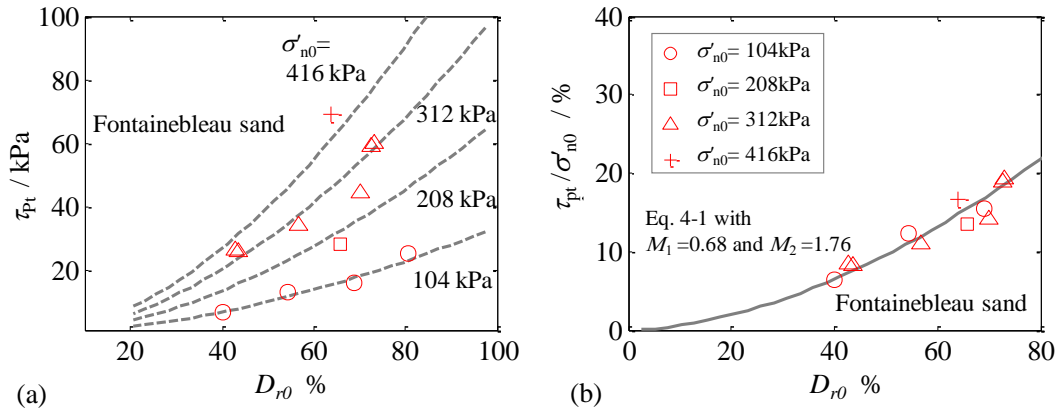
Figure 4.3 Shear stress at phase transformation as a function of experimental variables initial effective normal stress and relative density: (a) shear stress at phase transformation versus initial relative density; (b) normalized shear stress at phase transformation versus initial relative density
