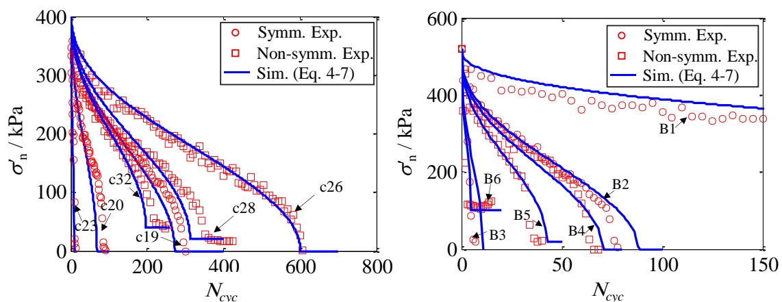
Figure 4.17 Comparisons between simulations and experiments on Fontainebleau sand: (a) training tests; (b) additional tests
