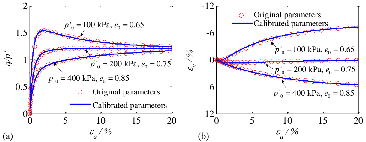
Figure 2.7 Comparison between synthetic results and simulated results by calibrated parameters: (a) stress ratio versus axial strain; (b) volumetric strain versus axial strain
