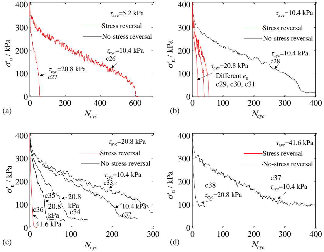
Figure 4.9 Degradation of effective normal stress under different average shear stresses: (a) 5.2 kPa; (b) 10.4 kPa; (c) 20.8 kPa; (d) 41.6 kPa
