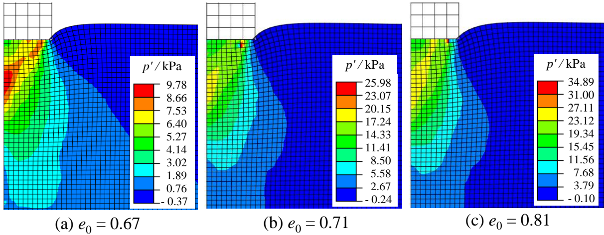
Figure 2.19 Simulated mean effective stress field of three footings at the settlement of 2.8 mm for the initial void ratio of: (a) e_0=0.67 ; (b) e_0=0.71 ; (c) e_0=0.81
