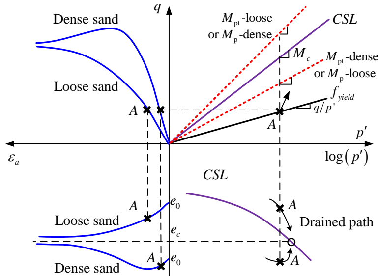
Figure 2.1 Principle of SIMSAND model
