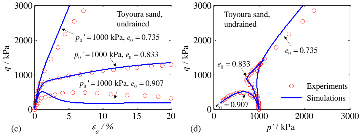
Figure 2.13 Comparison between experiments and simulations of undrained triaxial tests on Toyoura sand under confining stresses of 100 kPa and 1000 kPa plotted in (a) and (c) deviatoric stress versus axial strain, (b) and (d) stress path in mean effective stress and deviatoric stress
