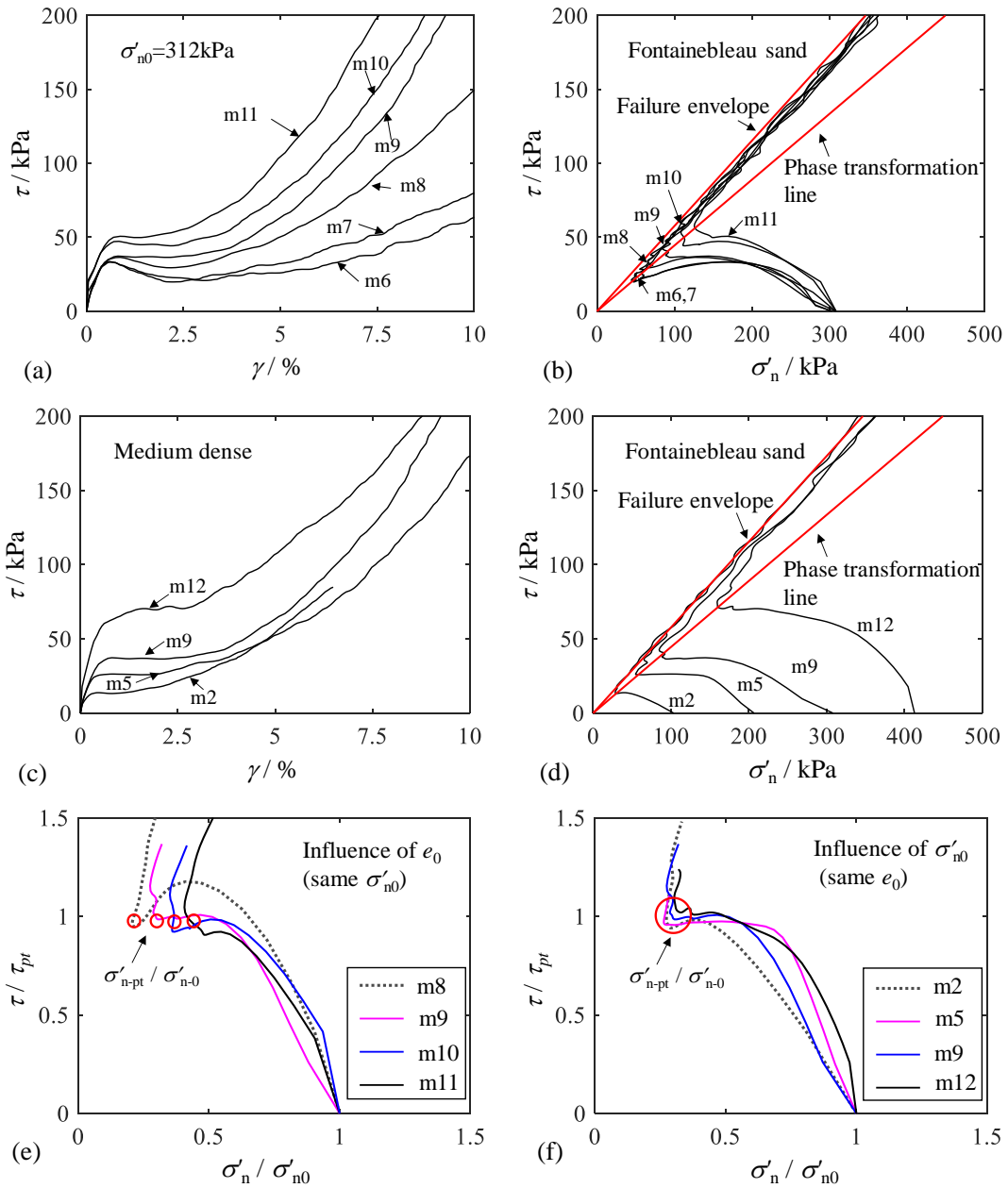
Figure 4.2 Undrained monotonic test results on Fontainebleau sand: (a-b) comparison results with different initial void ratios; (c-d) comparison results with different initial effective normal stresses; (e-f) normalized monotonic behaviour with different initial void ratios and effective normal stresses
