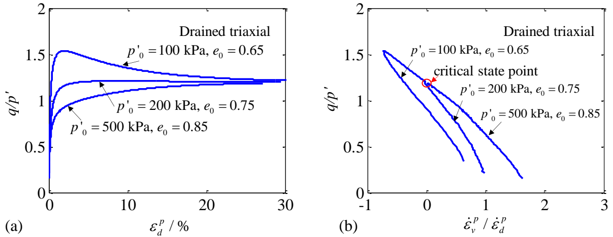
Figure 2.5 Increments of plastic strain of drained triaxial tests: (a) stress ratio versus deviatoric plastic strain; (b) stress ratio versus ratio of plastic strain increment
