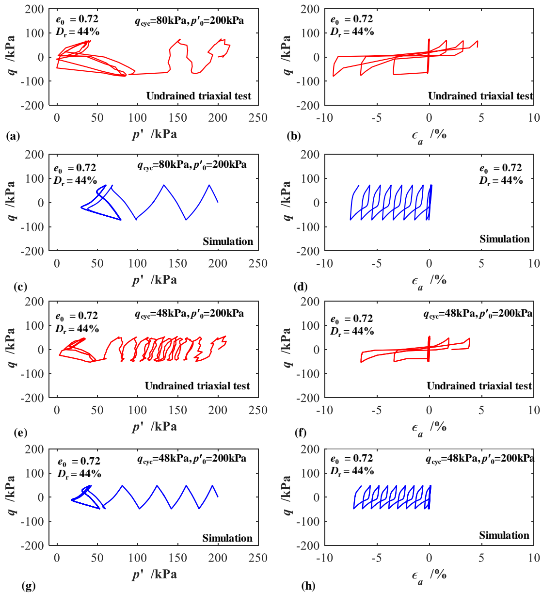
Figure 6.8 Comparison between experimental and numerical results of undrained cyclic tests on loose Fontainebleau sand: (a)-(b) experiment with q_{cyc}=80\text{kPa} , (c)-(d) simulation with q_{cyc}=80\text{kPa} (e)-(f) experiment with q_{cyc}=48\text{kPa} and (g)-(h) simulation with q_{cyc}=48\text{kPa}
