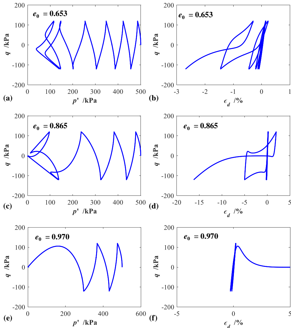
Figure 6.5 Comparison between the experimental and numerical results of undrained triaxial tests under cyclic loading on Toyoura sand with different initial void ratios: in (a), (c) and (e) stress path in mean effective stress versus deviatoric stress; (b), (d) and (f) deviatoric stress versus deviatoric strain
