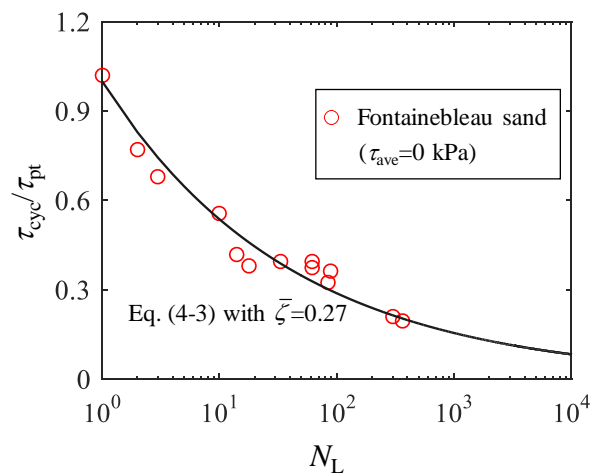
Figure 4.6 Normalized cyclic shear stress versus number of cycles to liquefaction
