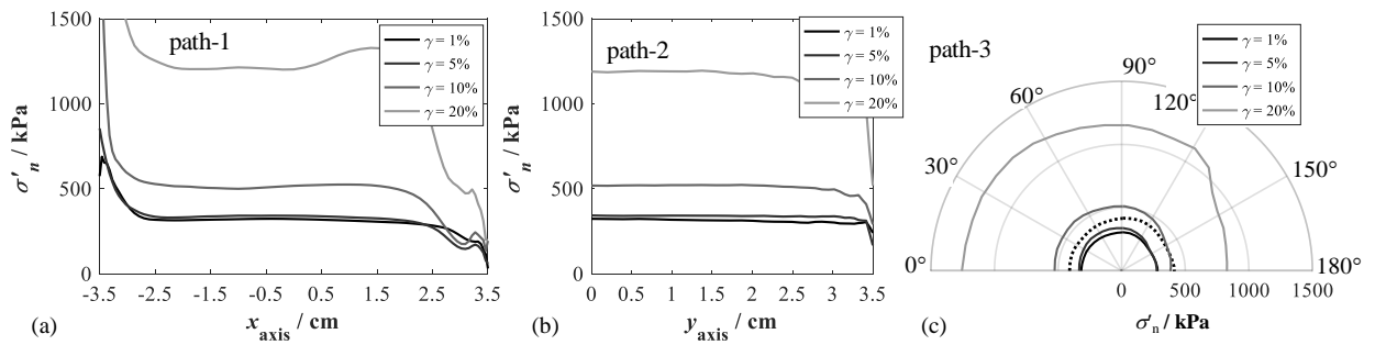
Figure 3.11 The distribution of vertical effective stress for constant volume test S-5 (a) along with path-1, (b) along with path-2 and (c) along with path-3
