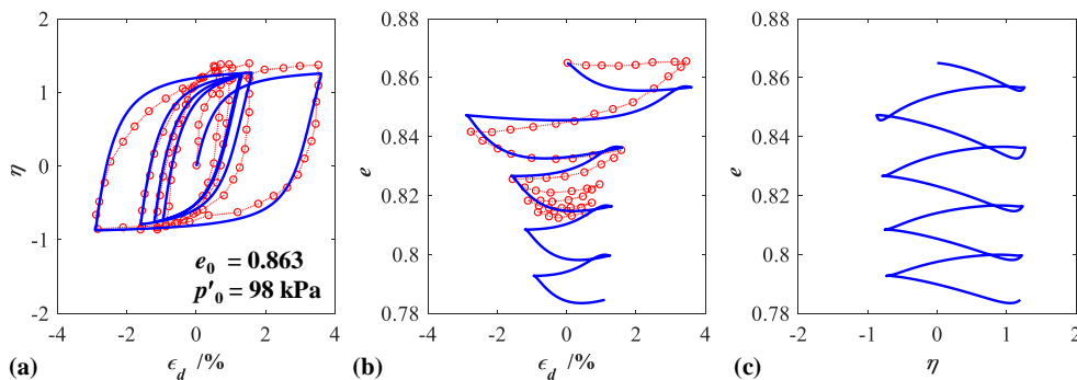
Figure 6.3 Comparison between experimental and numerical results for drained cyclic triaxial tests on Toyoura sand: in (a) stress ratio versus deviatoric strain, (b) void ratio versus deviatoric strain and (c) void ratio versus stress ratio
