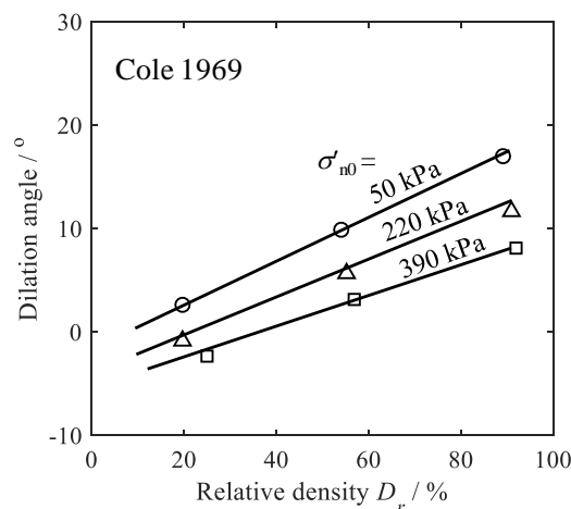
Figure 1.11 Dependence of dilation angle on relative density and stress level (Cole 1969)
