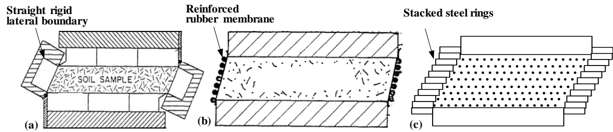
Figure 1.8 Simple shear apparatus: (a) Cambridge type (Budhu and Britto 1987), (b) NGI type (Budhu and Britto 1987) and (c) GDS type
