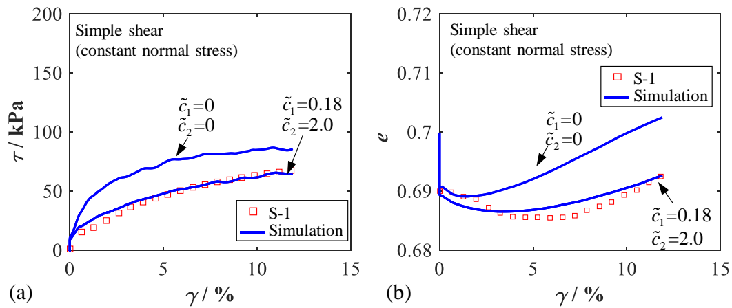
Figure 3.8 Calibration of anisotropic parameters: (a) shear strain versus shear stress (b) shear strain versus void ratio
