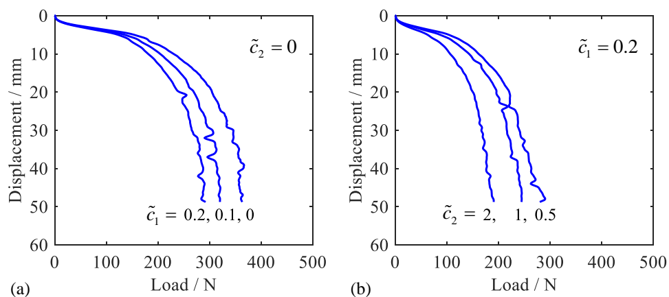
Figure 6.16 Influence of inherent anisotropy related parameters on pile resistance to investigate: (a) the effect of parameter \tilde{c}_1 , and (b) the effect of sensitivity of parameter \tilde{c}_2
