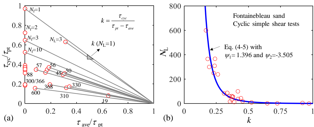
Figure 4.12 Cyclic resistance diagram for cyclic simple shear tests on Fontainebleau sand: (a) relationship between normalized cyclic shear stress and normalized average shear stress; (b) empirical curves for number of cyclic to liquefaction
