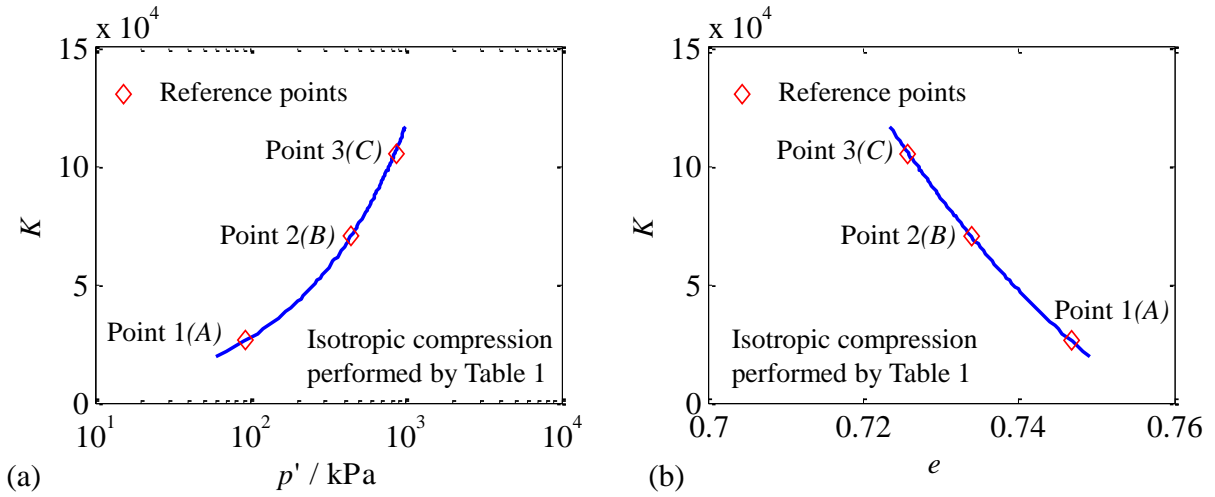
Figure 2.4 New interpreted curves from isotropic compression curve in (a) Elastic bulk moduli versus mean effective stress and (b) Elastic bulk moduli versus void ratio
