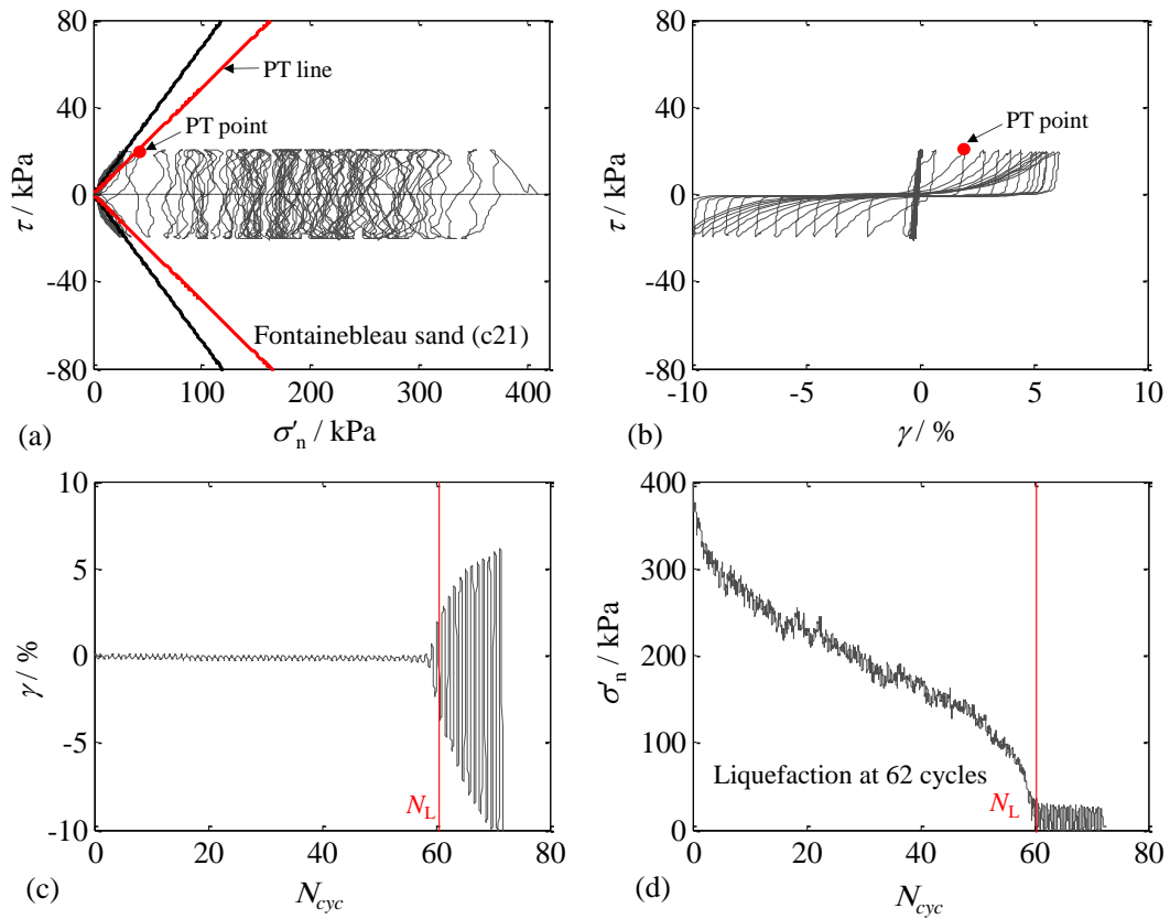
Figure 4.4 Symmetrical cyclic response of Fontainebleau sand: (a) shear stress versus effective normal stress; (b) shear stress versus shear strain, (c) shear strain versus number of cycles; (d) effective normal stress versus number of cycles
