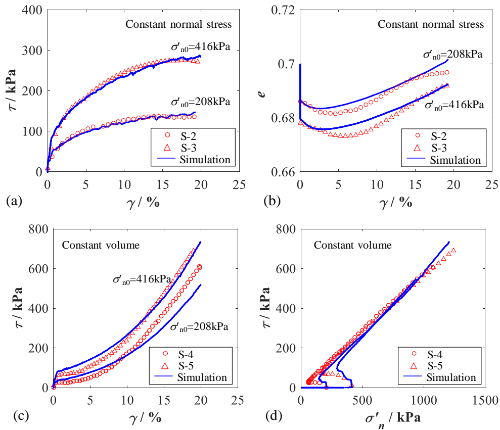
Figure 3.9 Simulation results by ideal and full three-dimensional simple shear tests (a) constant normal stress simple shear in \gamma - \tau space; (b) constant normal simple shear in \gamma - e space; (c) constant volume simple shear in \gamma - \tau space; (d) constant volume simple shear in \sigma'_n - \tau space.
