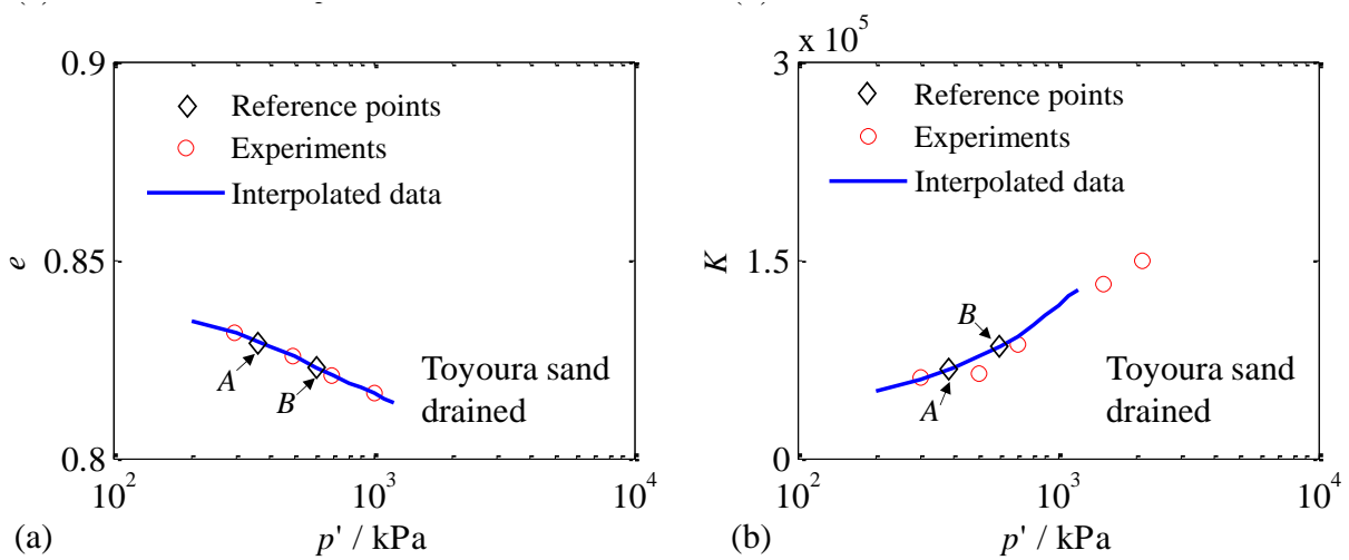
Figure 2.9 Interpreted results from isotropic compression curves of Toyoura sand for calibrating parameters: (a) void ratio versus mean effective stress and (b) Elastic bulk moduli versus mean effective stress
