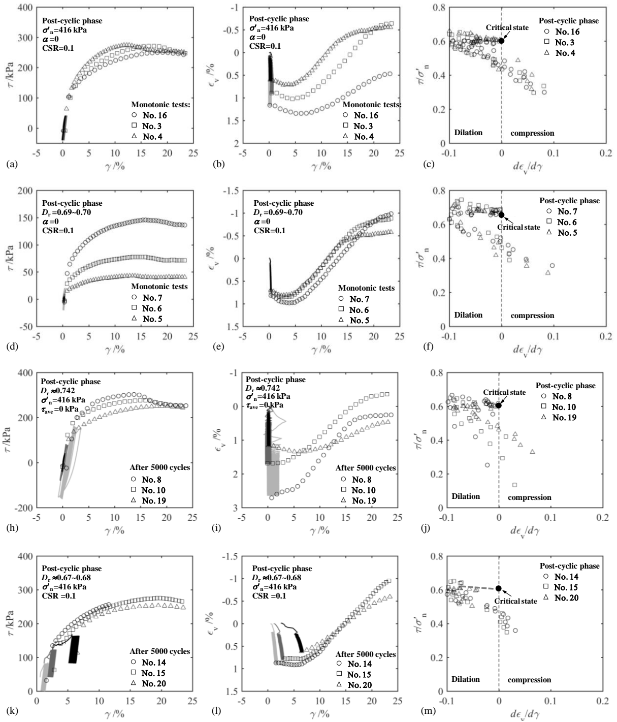
Figure 5.2 Summary of drained monotonic simple shear after 5000 cycles: (a)-(c) comparisons by different initial relative densities; (d)-(f) comparisons by different effective normal stresses; (h)-(j) comparisons by different cyclic shear stress ratios; (k)-(m) comparisons by different average shear stress ratios
