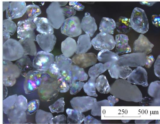
Figure 3.5 Particle shape of Fontainebleau sand
