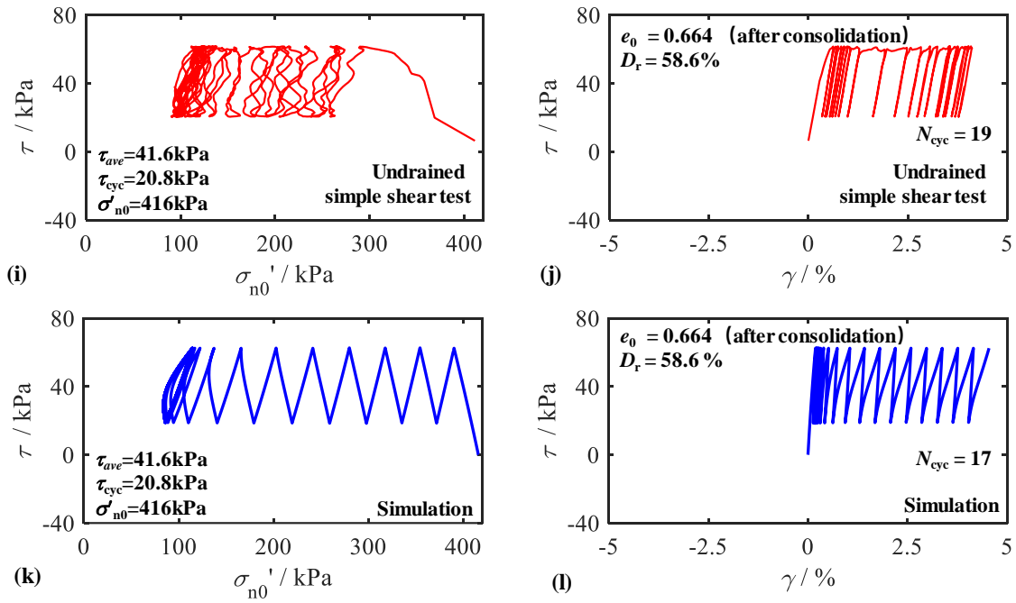
Figure 6.9 Experimental and numerical results of undrained cyclic tests on medium dense Fontainebleau sand on 416kPa initial normal stress: (a)-(d) comparison on condition ( \tau_{ave} = 0 kPa, \tau_{cyc} = 20.8 kPa), (e)-(h) comparison on condition ( \tau_{ave} = 10.4 kPa, \tau_{cyc} = 20.8 kPa) and (i)-(l) comparison on condition ( \tau_{ave} = 41.6 kPa, \tau_{cyc} = 20.8 kPa)
