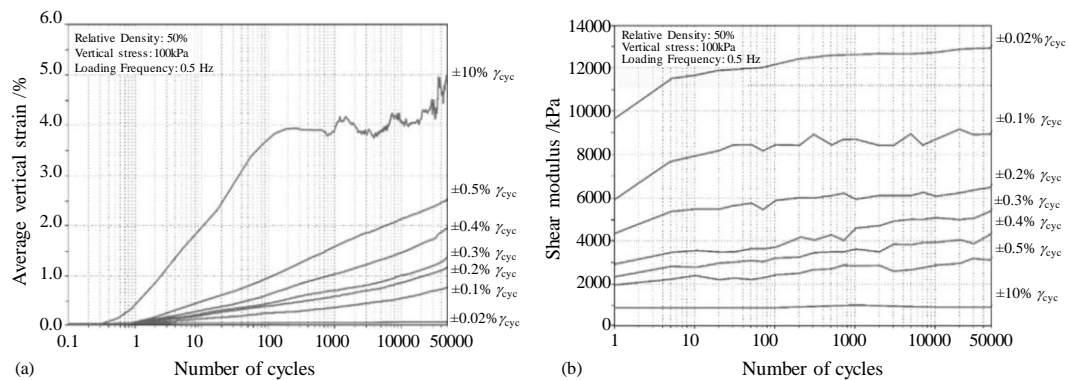
Figure 1.7 Cyclic drained simple shear tests with 100kPa normal stress: (a) vertical strain with cyclic number, (b) shear modulus with cyclic number (Nikitas et al. 2017)
