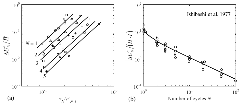
Figure 1.18 Parameters calibration of Ishibashi et al model: (a) calibration parameter \chi , (b) calibration parameter C_{1-3} (after Ishibashi et al. 1977)
