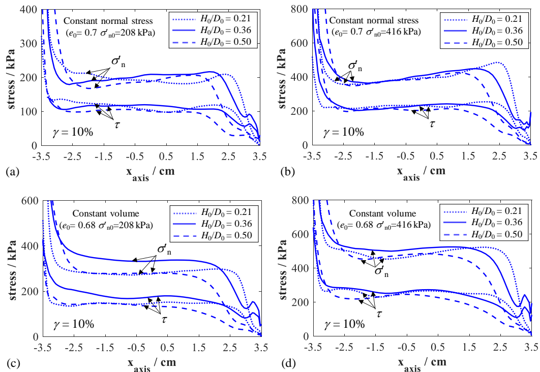
Figure 3.18 Results for different aspect ratios of specimens about distribution of normal stress and shear stress on the Path-1: (a) constant normal stress condition ( \sigma'_{n0} = 208\text{kPa} ); (b) constant normal stress condition ( \sigma'_{n0} = 416\text{kPa} ); (c) constant volume condition ( \sigma'_{n0} = 208\text{kPa} ); (d) constant volume condition ( \sigma'_{n0} = 416\text{kPa} )
