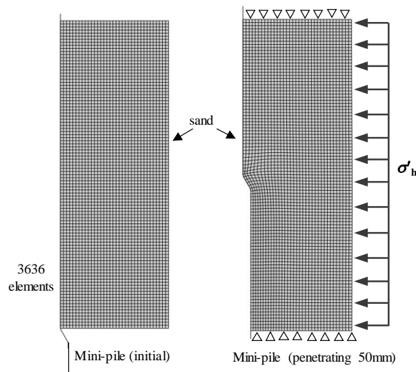
Figure 6.13 Finite element analysis of 3SR mini model pile
