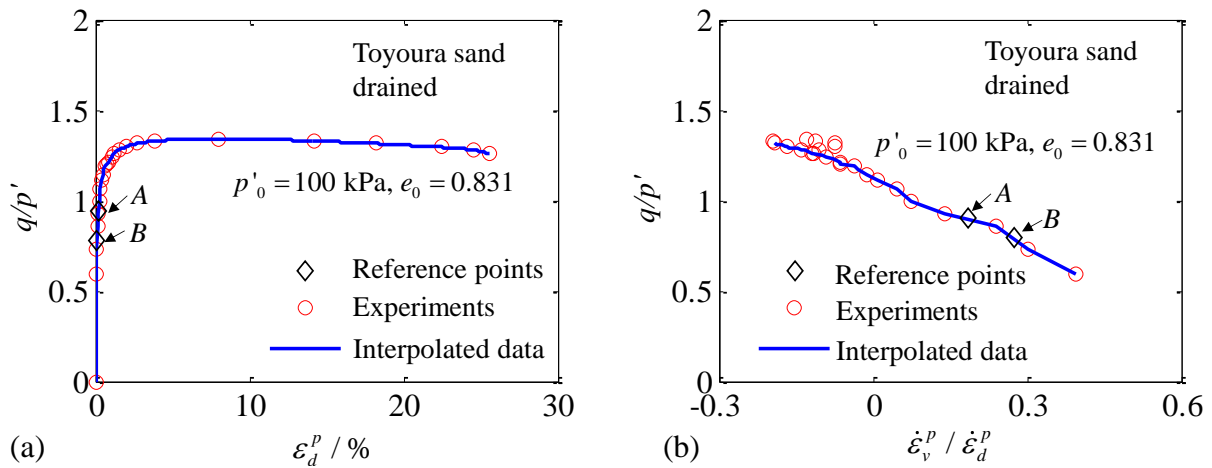
Figure 2.10 Increments of plastic strain of drained triaxial tests on Toyoura sand: (a) stress ratio versus deviatoric plastic strain; (b) stress ratio versus ratio of plastic strain increment
