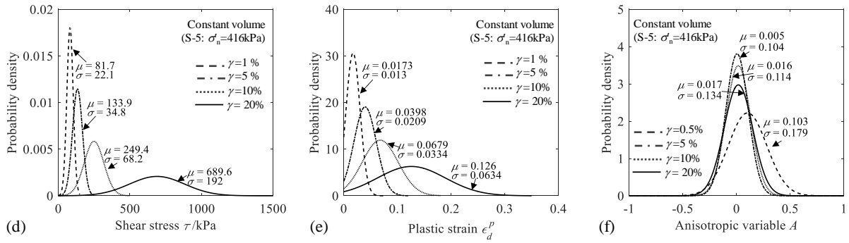
Figure 3.15 Probability distribution analysis with increasing of shear strain based on constant normal stress (a) shear stress, (b) plastic strain and (c) anisotropic variable, and constant volume (d) shear stress, (e) plastic strain and (f) anisotropic variable
