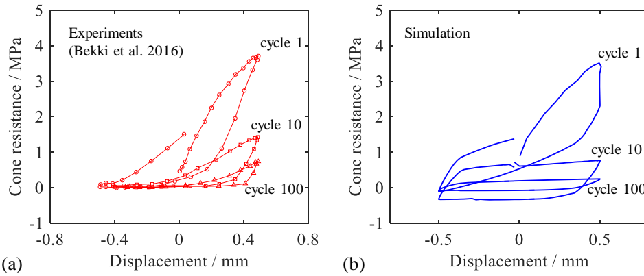
Figure 6.25 Cone resistance of cyclic model pile test (a) experiment and (b) simulation
