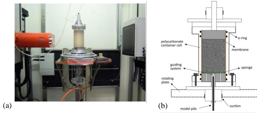
Figure 6.12 Details of 3SR mini-scale model pile tests (Silva 2014), (a) model pile with micro-CT scan apparatus and (b) geometry of model-pile penetration tests
