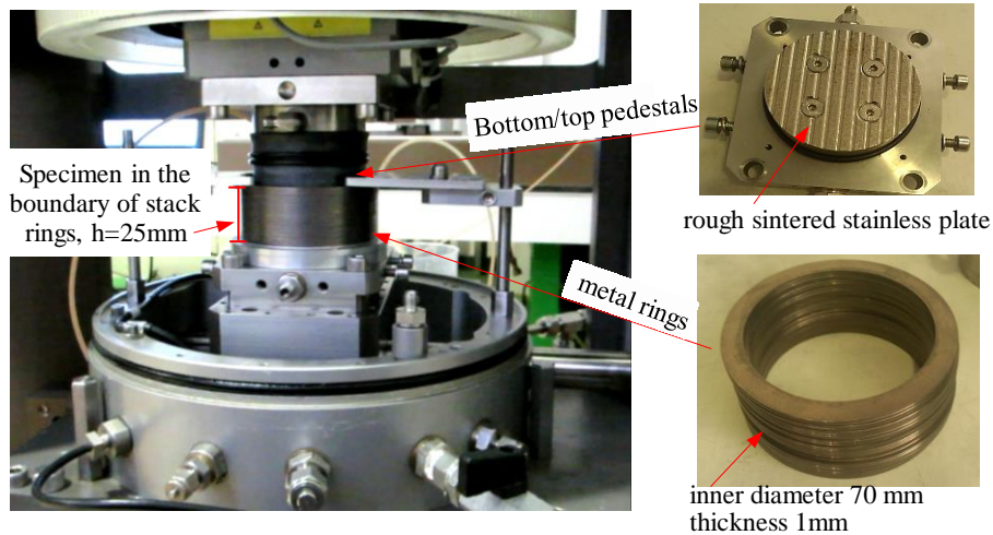
Figure 3.6 Details of cylindrical boundary for simple shear specimen
