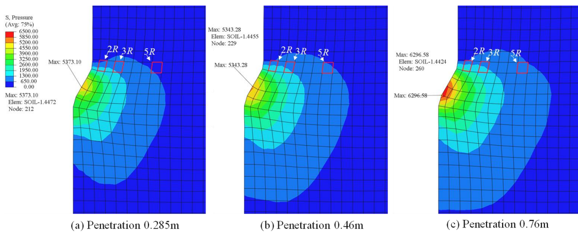
Figure 6.21 Simulation results of mean effective stress field around the cone of pile at the penetration depth of (a) 0.285m; (b) 0.46m and (c) 0.76m in Fontainebleau sand NE34
