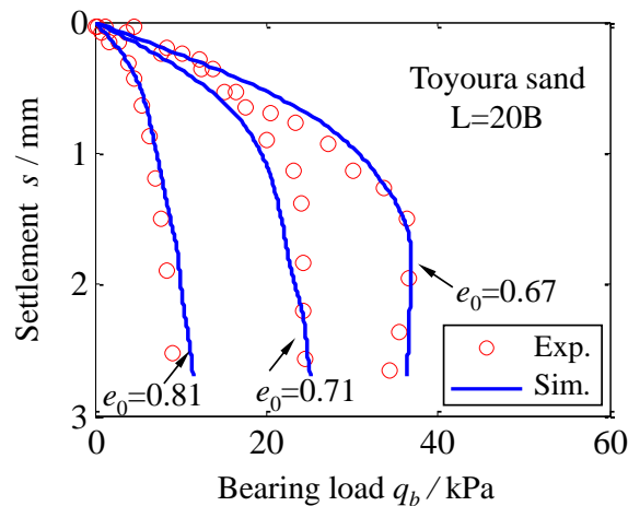
Figure 2.18 Comparison between measurements and predictions of bearing load versus settlement for three footing tests in sand with three different initial void ratios
