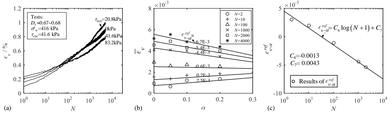
Figure 5.6 Volumetric strain accumulation with different average shear stress ratio: (a) volumetric strain versus number of cycles; (b) normalized volumetric strain versus average shear stress ratio; (c) reference volumetric strain versus number of cycles
