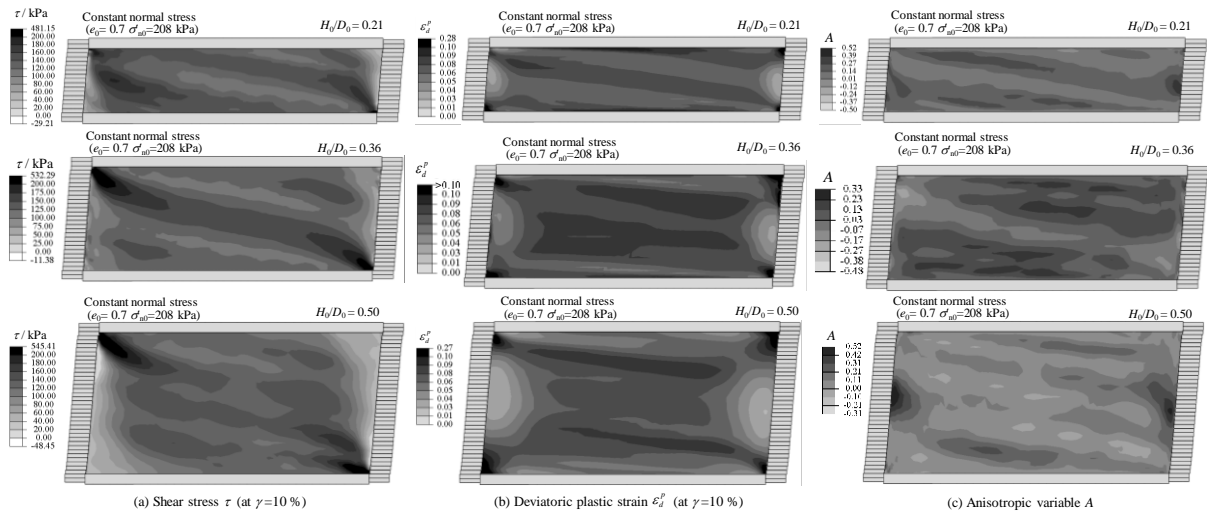
Figure 3.19 Comparisons of different aspect ratios of specimens for the constant normal stress condition (test S-2): (a) contour of shear stress at \gamma = 10\% , (b) contour of deviatoric plastic strain at \gamma = 10\% , (c) contour of Anisotropic variable A at \gamma = 10\%
