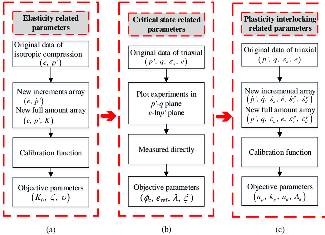
Figure 2.3 Procedure of proposed straightforward method from (a) elasticity related parameters, (b) critical state related parameters to (c) plasticity interlocking related parameters
