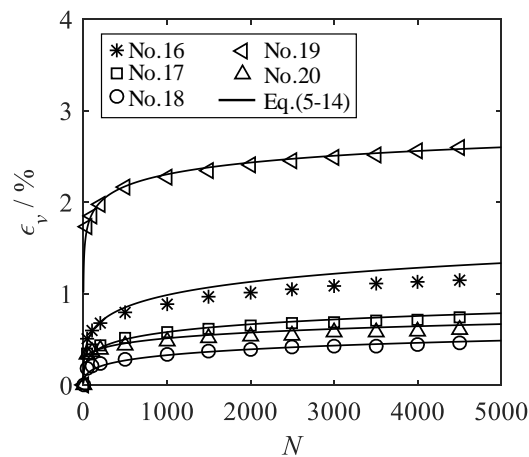
Figure 5.8 Validation of the analytical model by five additional tests No.16-20
