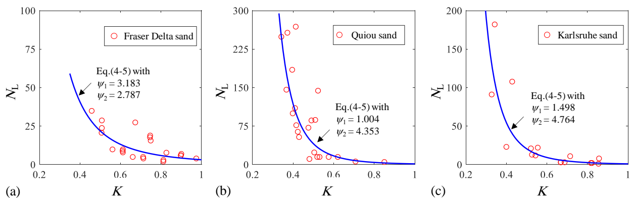
Figure 4.16 Calibration results of numbers of cycles to instability: (a) Fraser River sand; (2) Quiou sand; (3) Karlsruhe sand
