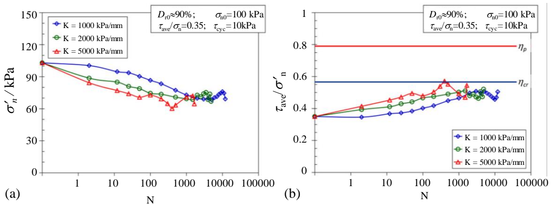
Figure 1.4 Experimental results (a) degradation of normal stress; (b) evaluation of stress ratio (Pra-ai and Boulon 2017)
