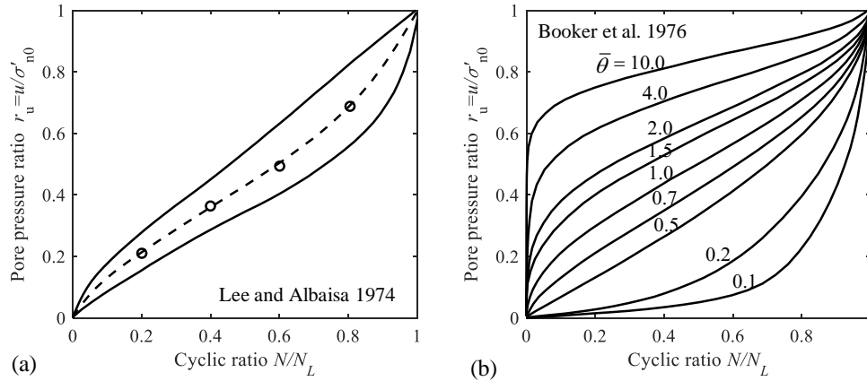
Figure 1.17 Rate of pore pressure generation: (a) Curves from Lee and Albaisa, 1974, and (b) Curves from Booker et al. (1976)
