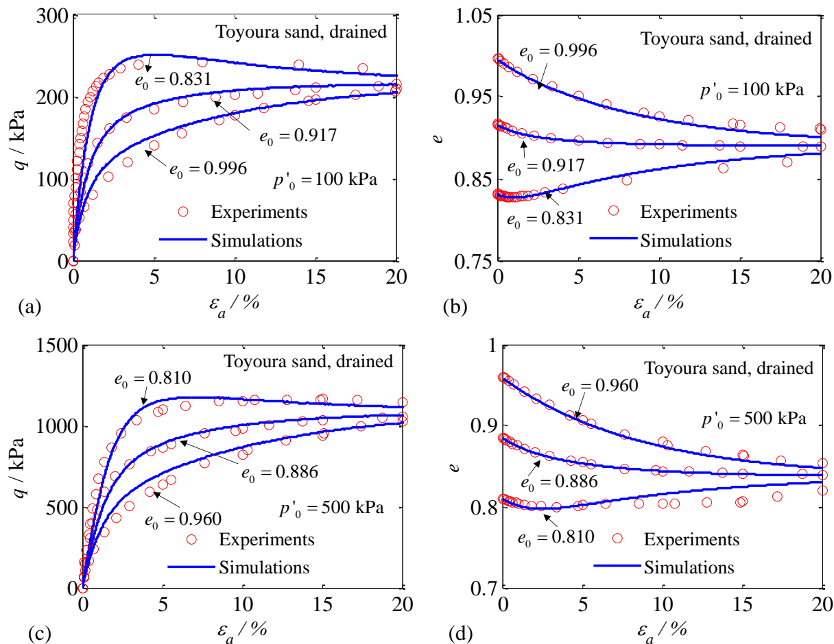
Figure 2.12 Comparison between experiments and simulations for six drained triaxial tests on Toyoura sand under confining stresses of 100 kPa and 500 kPa plotted in (a) and (c) deviatoric stress versus axial strain, (b) and (d) void ratio versus axial strain
