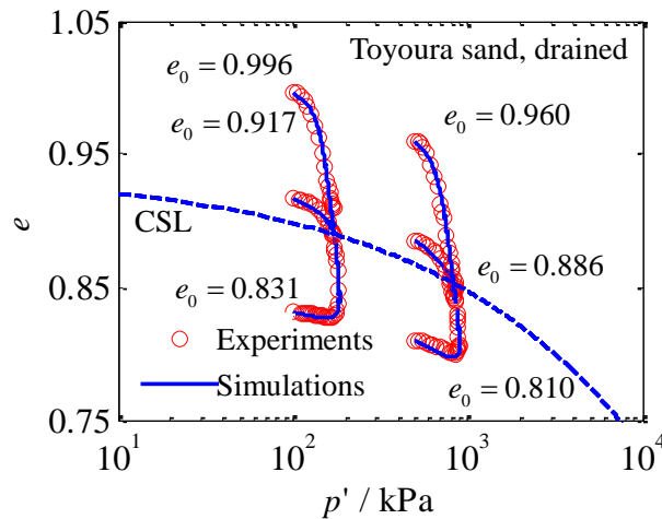
Figure 2.11 Comparison between experiments and simulations for six drained triaxial tests on Toyoura sand under confining stresses of 100 kPa and 500 kPa plotted in void ratio versus mean effective stress space
