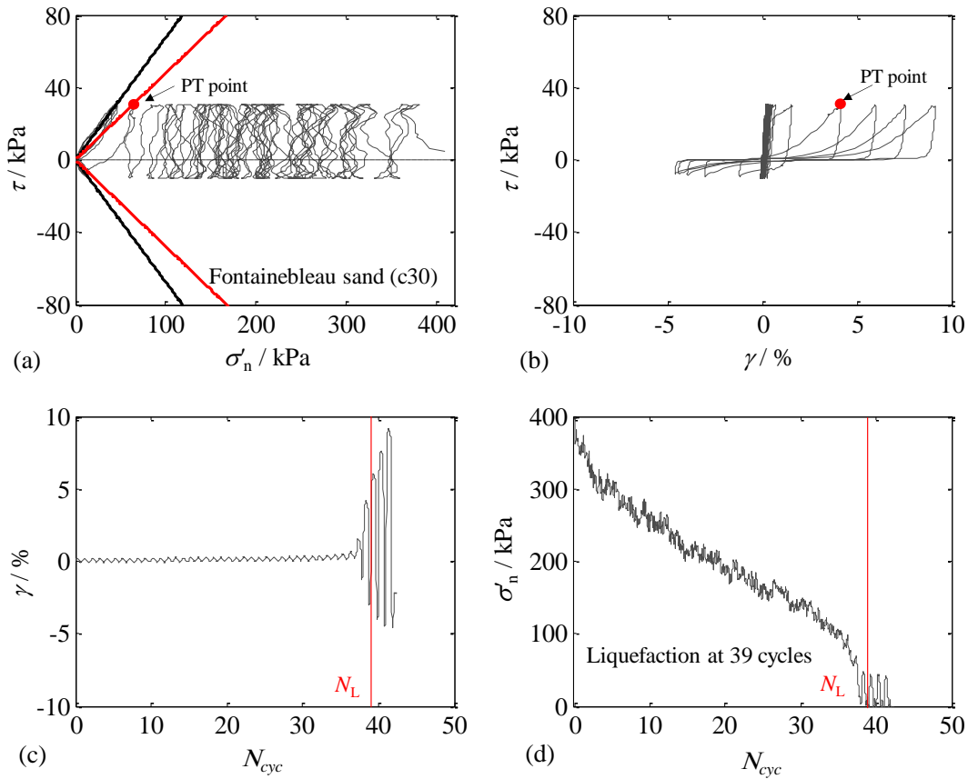
Figure 4.7 Non-symmetrical cyclic response of Fontainebleau sand with stress reversal loading: (a) shear stress versus effective normal stress; (b) shear stress versus shear strain, (c) shear strain versus number of cycles; (d) effective normal stress versus number of cycles
