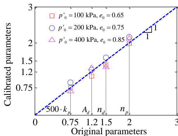
Figure 2.6 Comparison between original given and calibrated parameters
