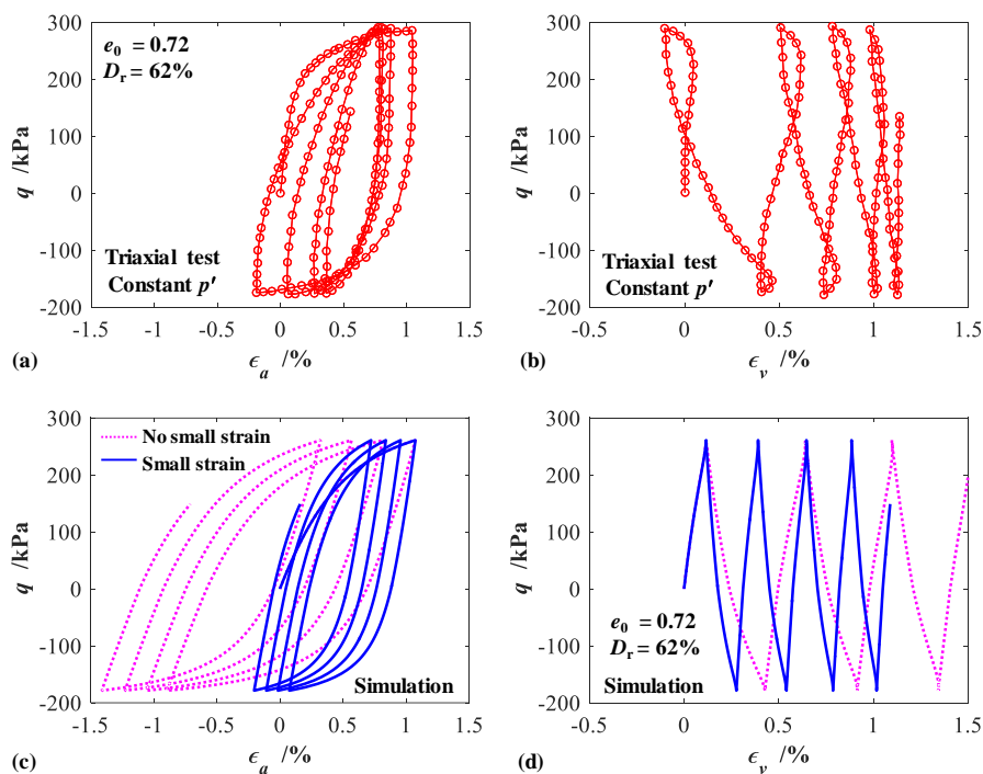
Figure 6.6 Comparison between experimental and numerical results of constant- p' drained cyclic tests on Fontainebleau sand: (a)-(b) experiment, and (c)-(d) simulation
