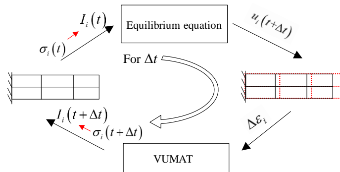
Figure 2.14 Flow chart of explicit finite element analysis based on ABAQUS/Explicit
