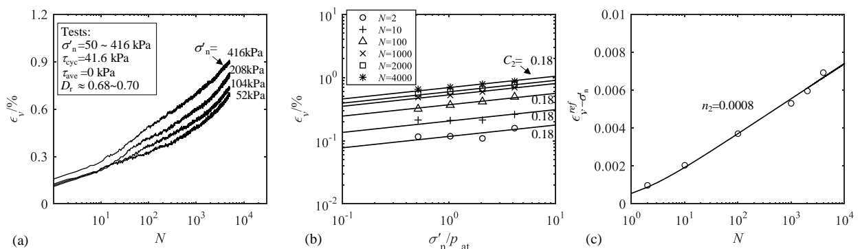
Figure 5.4 volumetric strain accumulation with different normal stress level: (a) volumetric strain versus number of cycles; (b) volumetric strain versus normal stress level; (c) reference volumetric strain versus number of cycles
