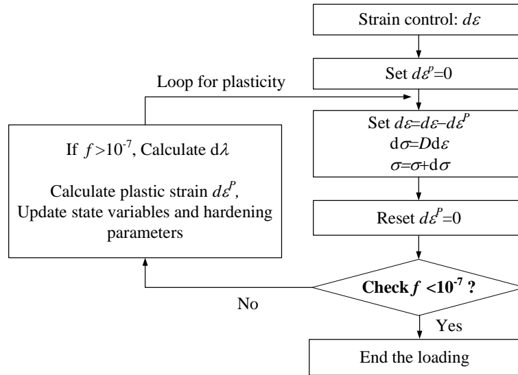
Figure 2.16 Flow chart of the cutting plane algorithm
