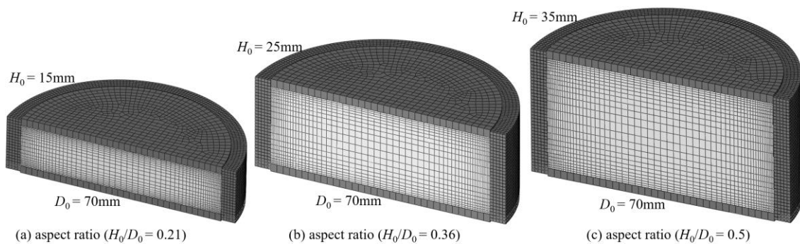
Figure 3.16 Finite element meshes for different aspect ratio of cylinder specimen: (a) H_0 = 15\text{ mm} ; (a) H_0 = 25\text{ mm} ; (c) H_0 = 35\text{ mm}
