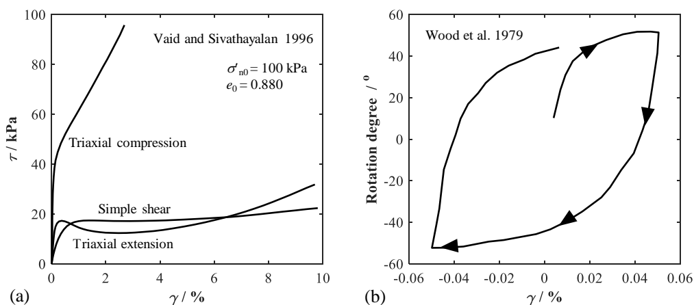
Figure 1.13 Tests of simple shear tests: (a) comparing to triaxial tests by Vaid and Sivathayalan (1996) and (b) principal stress rotation of simple shear tests by Wood et al. (1979)
