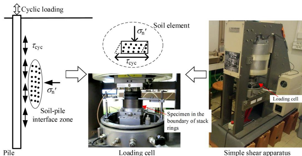
Figure 4.1 Analysis of soil element adjacent to pile based on simple shear apparatus
