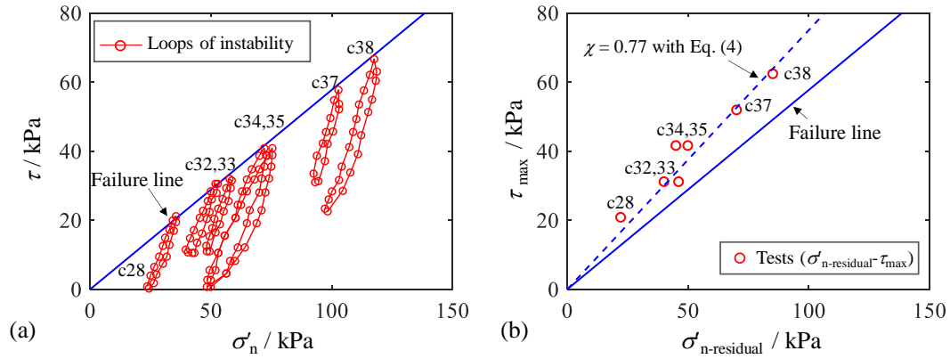
Figure 4.10 Evaluation of effective residual normal stress in no-stress reversal cyclic loading
