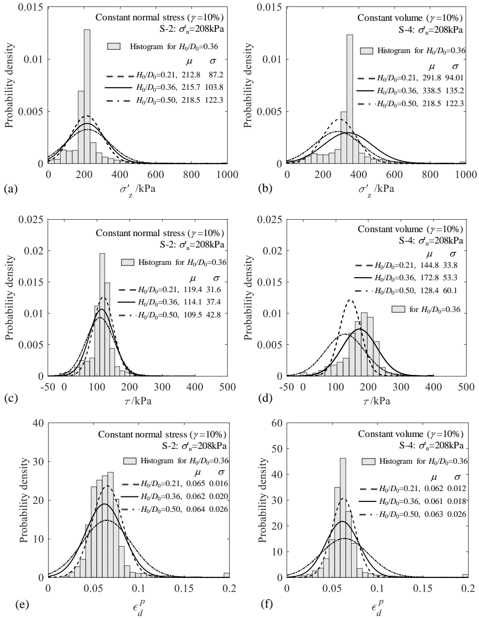
Figure 3.21 Probability distribution analysis with different aspect ratios at 10% shear strain: (a-b) for vertical stress \sigma'_z , (c-d) for shear stress \tau and (e-f) for deviatoric plastic strain \epsilon_d^p
