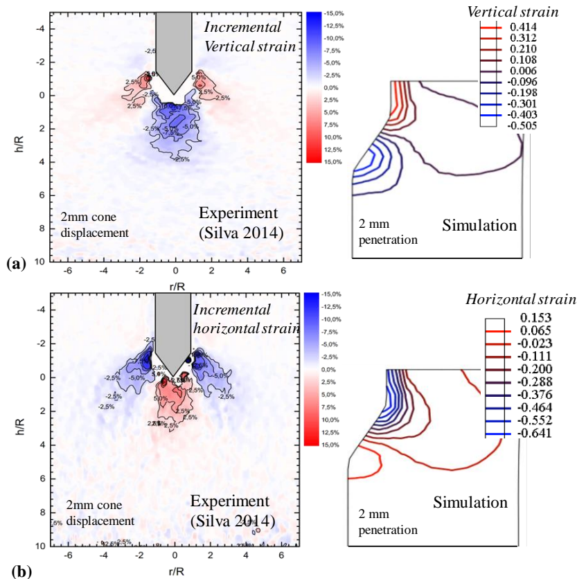
Figure 6.15 Comparison of strain profiles between experiment and simulation (a) vertical strain and (b) horizontal strain
