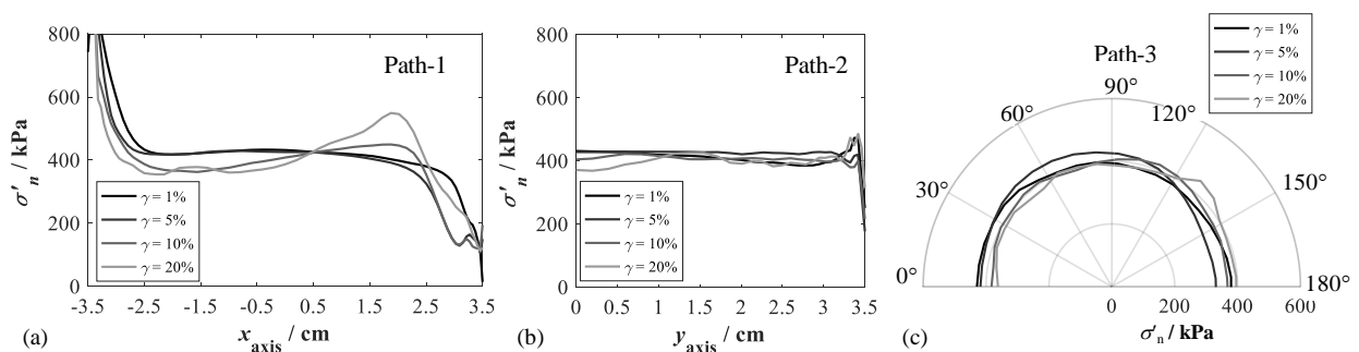
Figure 3.10 The distribution of vertical effective stress for constant normal stress test S-3 (a) along with path-1, (b) along with path-2 and (c) along with path-3
