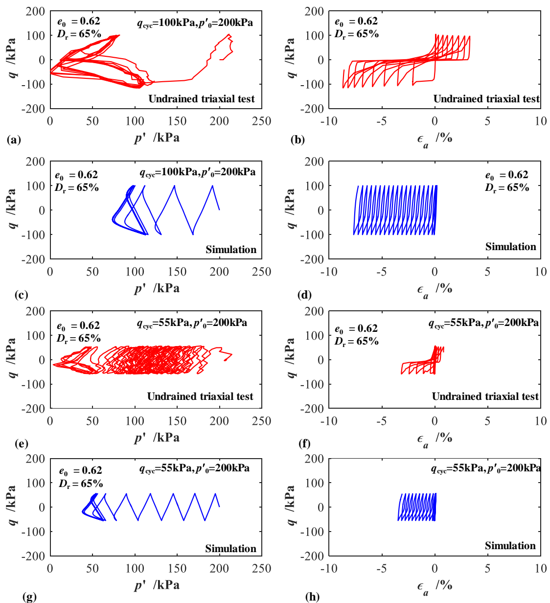
Figure 6.7 Comparison between experimental and numerical results of undrained cyclic tests on medium-dense Fontainebleau sand: (a)-(d) with q_{cyc} = 100 kPa and (e)-(h) with q_{cyc} = 55 kPa
