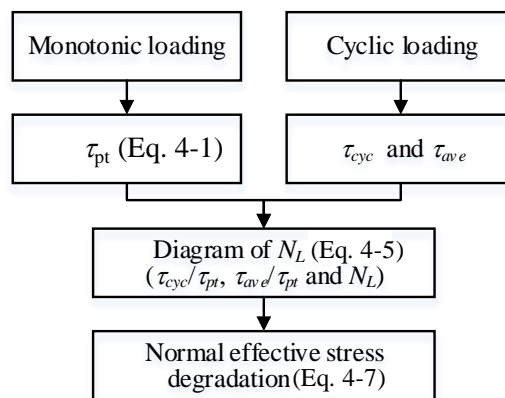
Figure 4.14 Calibration procedure for the degradation of the effective normal stress
