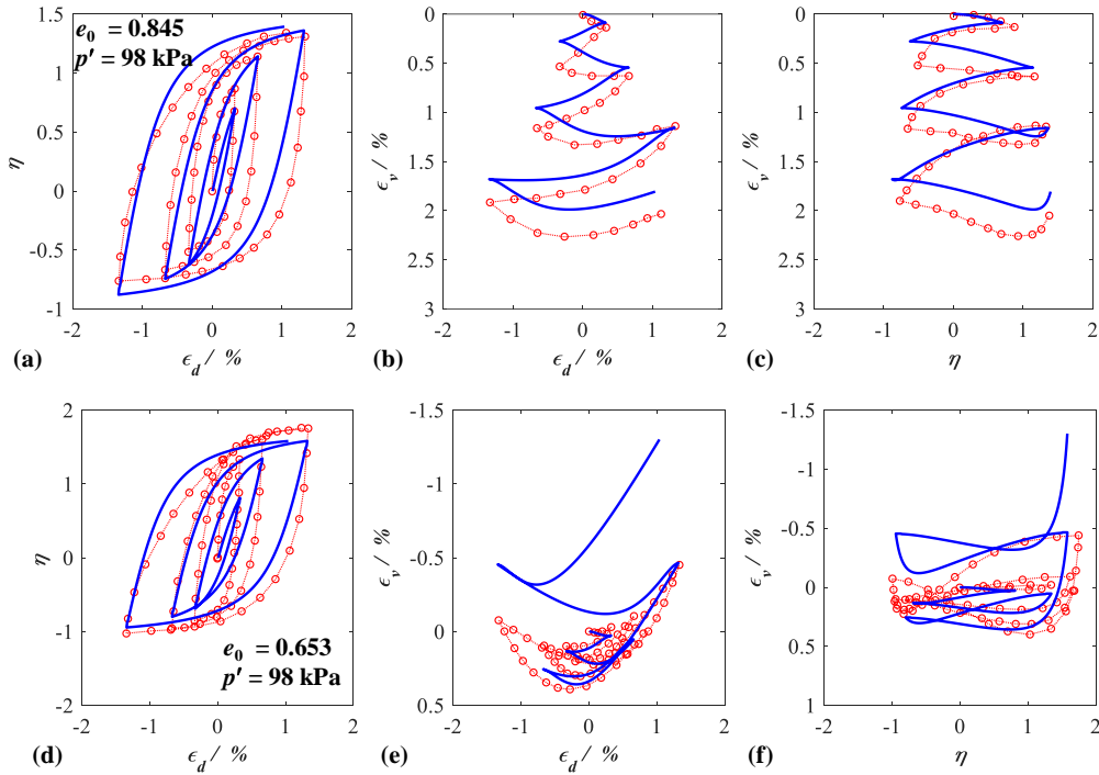
Figure 6.2 Comparison between experimental and numerical results of constant- p' drained cyclic tests on Toyoura sand: (a)-(c) loose specimen and (d)-(f) dense specimen
