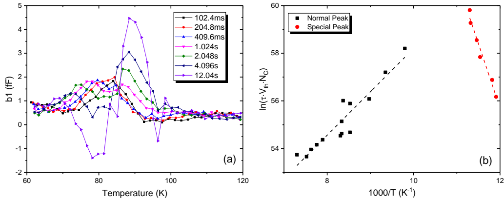
Figure 5.25. (a): DLTS spectra (b1) between 60 K and 120 K with 7 different period widths on Tungsten diode (S7) and (b) is its Arrhenius plot extracted.
