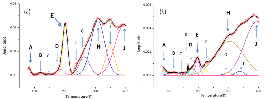
Figure 5.17. DLTS signal and the peak analysis by Origin on (a): diode (L) with T_p = 1 \text{ ms} , T_w = 100 \text{ ms} and (b): diode (S) with T_p = 1 \text{ ms} , T_w = 200 \text{ ms} between 80 K and 400 K. The sizes of the Alphabets represent the height of each individual peak.
