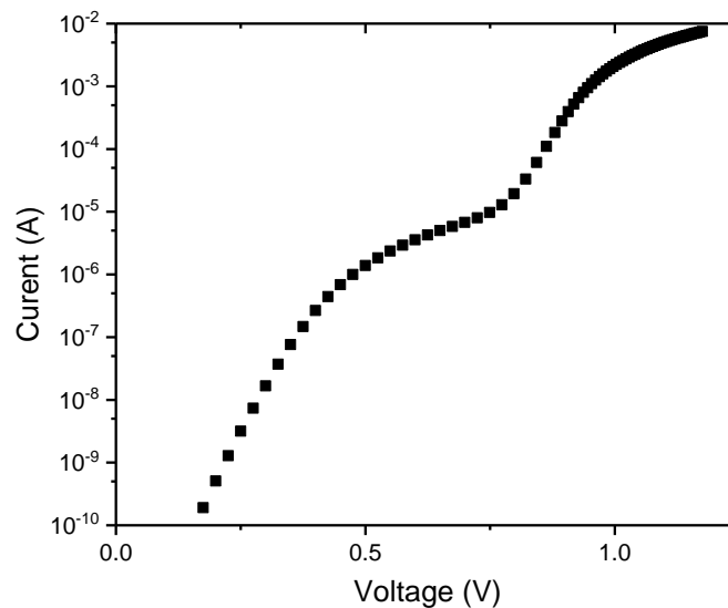
Figure 1.3. Double barrier phenomenon in Schottky diode.
