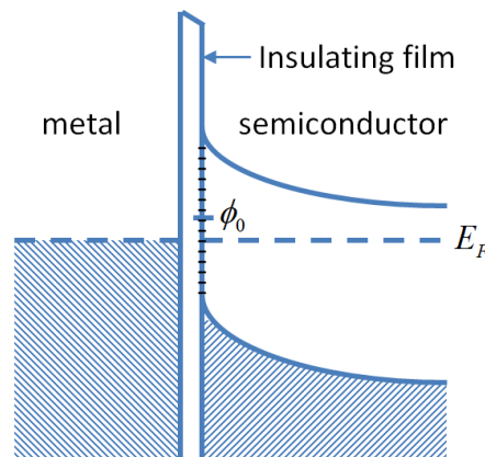
Figure 2.2. Metal-semiconductor contact with interface states.
