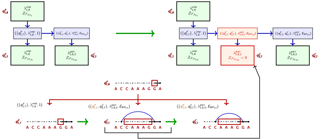
Figure 3.7: Linking the parent and children nodes in the data-structure for non-redundant sampling in tree \mathfrak{d}(w, \mathcal{Q}_{Zuk}, q_{1,9}^F, \rho_{Zuk}) . Here no secondary structure with pair (2, 8) was created beforehand, therefore node \lambda_{1,8,2}^{pair} is not yet created. If such structure is sampled the not gets inserted to its respective position, copying the order within DP scheme (\mathcal{Q}_{Zuk}, q_{1,9}^F, \rho_{Zuk}) .
