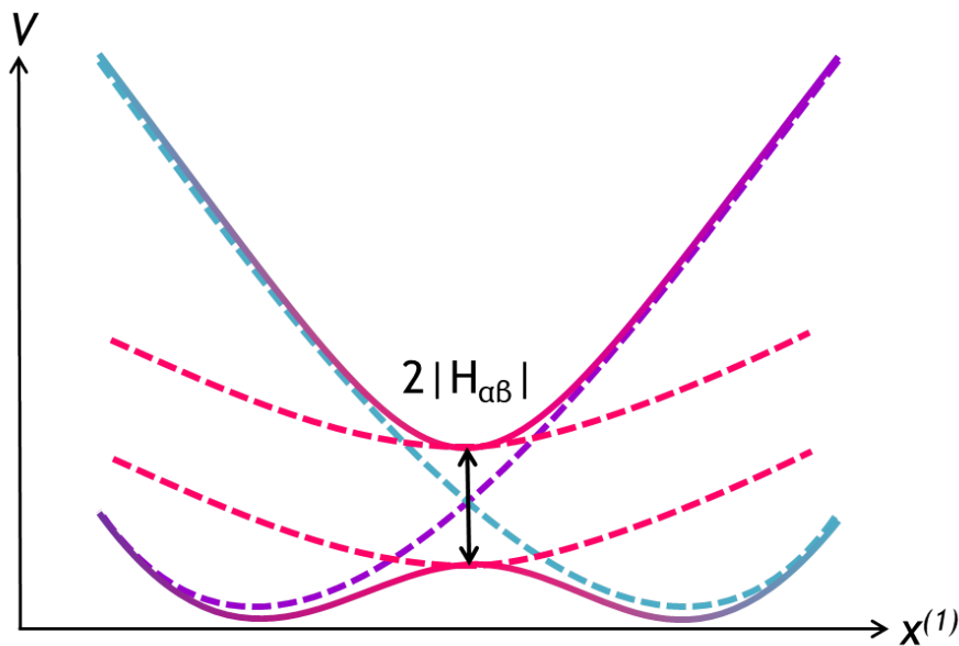
Figure 2.6: Electronic potentials along the mode x^{(1)} at a point displaced from the conical intersection along x^{(2)} (avoided crossing). Adiabatic potentials are in full line, diabatic potentials are in dashed line. x^{(1)} ( x^{(2)} ) is the tuning (coupling) mode for the diabatic states |\Phi_{\alpha}^{\text{dia}}; \mathbf{R}\rangle and |\Phi_{\beta}^{\text{dia}}; \mathbf{R}\rangle that tend asymptotically to the adiabatic states. At the avoided crossing, the adiabatic states are identical to the \pi/4 -rotated diabatic states |\Phi_{+}^{\text{dia}}; \mathbf{R}\rangle and |\Phi_{-}^{\text{dia}}; \mathbf{R}\rangle (pink dashed lines).
