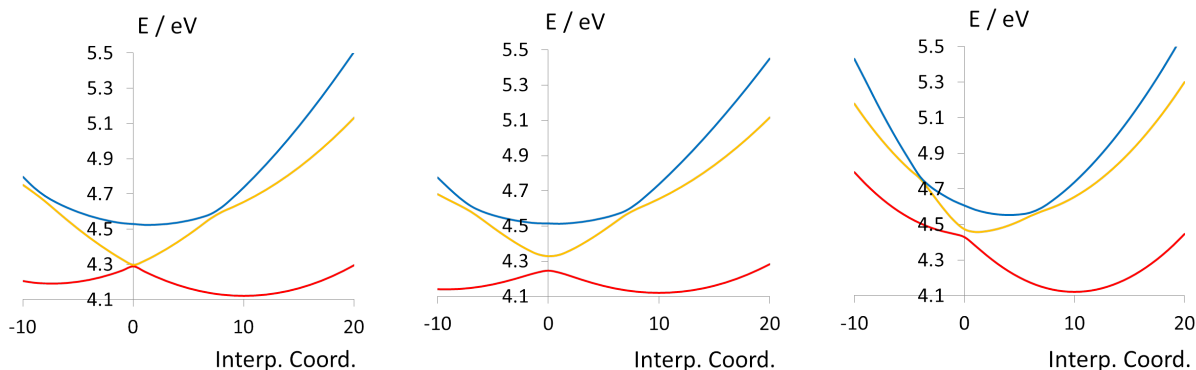
Figure 9.14: Evolution of the energies of the first three adiabatic states S_1 (red), S_2 (yellow), S_3 (blue) along the linear interpolations between TS_{A_1} (point 0) and minS_1 (point 10) on the left; between TS_{B_2} (point 0) minS_1 (point 10) in the center; between minS_0 (point 0) and minS_1 (point 10) on the right.
