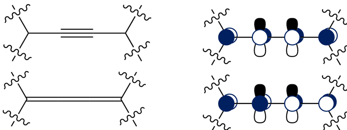
Figure 8.5: Orbital interaction of the alternated single-triple-single (top) and double-single-double (bottom) bonding schemes.
