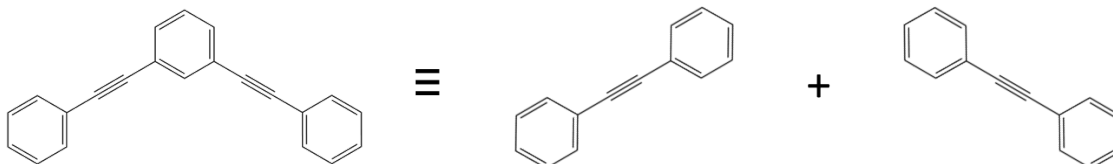
Figure 13.9: Pseudo-fragment decomposition of m22.
