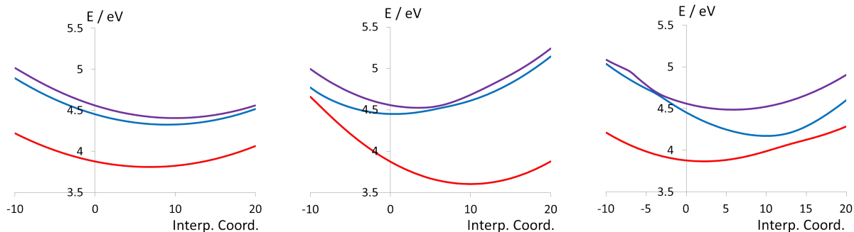
Figure 10.5: Evolution of S_1 (red), S_2 (blue), S_3 (purple) along the linear interpolations and extrapolations from minS_0 to minS_3 (left), minS_1 (middle), and minS_2 (right). Point 0 corresponds to minS_0 , point 10 corresponds to minS_3 , minS_1 and minS_2 , respectively.
