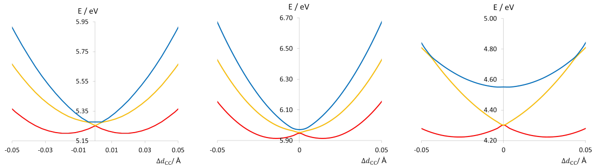
Figure 9.20: Evolution of the energies of the first three adiabatic states S_1 (red), S_2 (yellow), S_3 (blue) along the antisymmetric ( b_2 ) mode of elongation of the acetylene around CI_{FC} (left), CI_{B_2} (middle), and CI_{A_1} (right).
