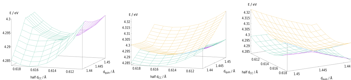
Figure 9.23: Evolution of the energies of the adiabatic states S_1 (green/purple) and S_2 (yellow/blue) around the lowest conical intersection along the symmetric elongations of acetylene and quinoidal bonds of TS_{A_1} .
