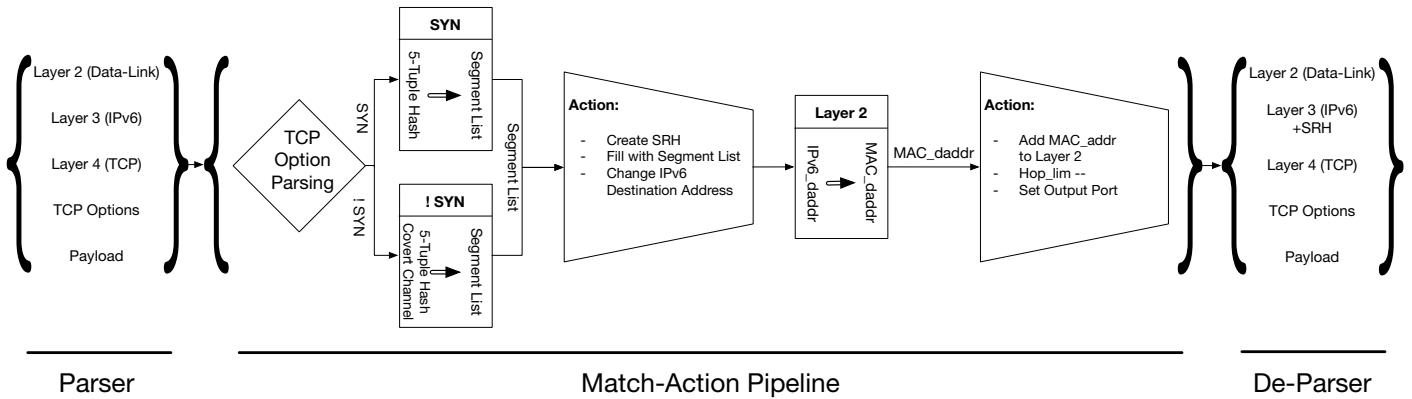
Figure 8.2 – SHELL P4 data-plane overview
