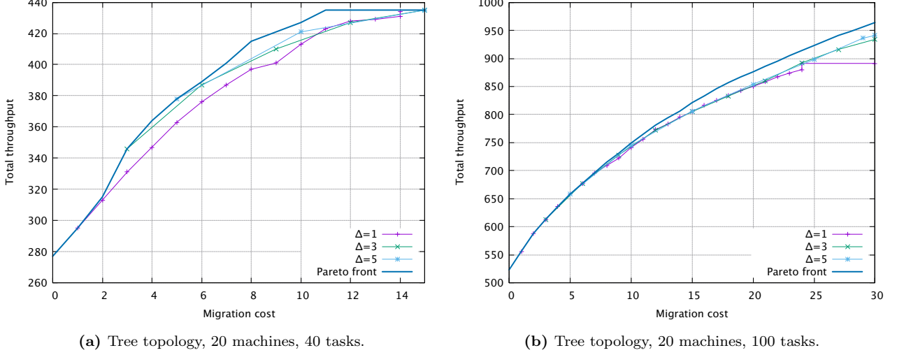
Figure 4.4 – Pareto front approximation: Exact Pareto front and approximate Pareto fronts from Algorithm 4 for \Delta \in \{1, 3, 5\} .
