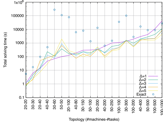
Figure 4.6 – Pareto front approximation: time to generate the approximate Pareto front, for up to B = 30 migrations. Exact Pareto front (Algorithm 3) vs approximate Pareto fronts (Algorithm 4) for \Delta \in \{1, 2, 3, 4, 5\} . 20 different scenarios.
