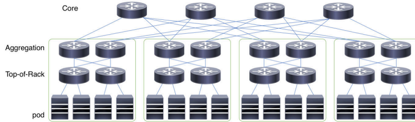
Figure 1.3 – Fat-tree data center network topology [35] with k = 4
