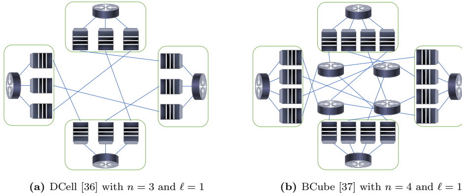
Figure 1.4 – Advanced data center network topologies
