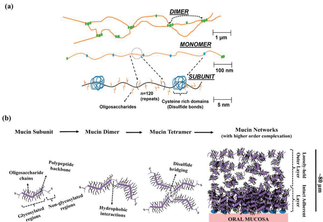
Figure 1.1. Structure of a mucin-like glycoprotein and its self-assembling in mucosa. (A) Basic structure of a glycoprotein subunit made of oligosaccharides pendant chains densely grafted on a protein core and cysteine rich domains. This repetition leads to the glycoprotein monomer which can self-assemble to form a dimer; (B) Illustration of the successive aggregation steps of glycoproteins mediated by hydrophobic interactions and cysteine moieties (disulfide bridging) to form the oral mucosa. From reference 17 .
