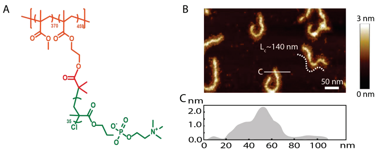
Figure 2.15. (A) Chemical structure of the bottle-brush polymer used in the study. (B) AFM picture of BB polymer deposited on mica surfaces from a 10 \mu\text{g}/\text{mL} polymer solution. (C) BB height profile of a perpendicular cross-section indicated with the white line in fig. 1B showing the contour of the polymer.
