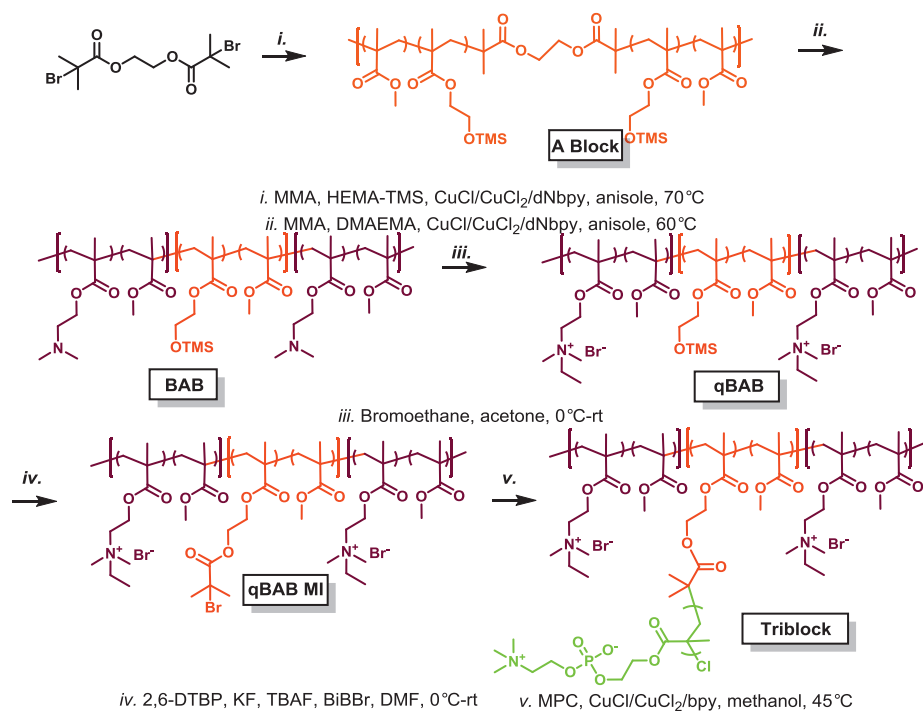
Figure 2.24. Synthesis of the triblock BB polymer
