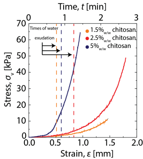
Figure 3.10. Compression study of chitosan hydrogels showing the critical strains for exudation of water for different chitosan hydrogels.
