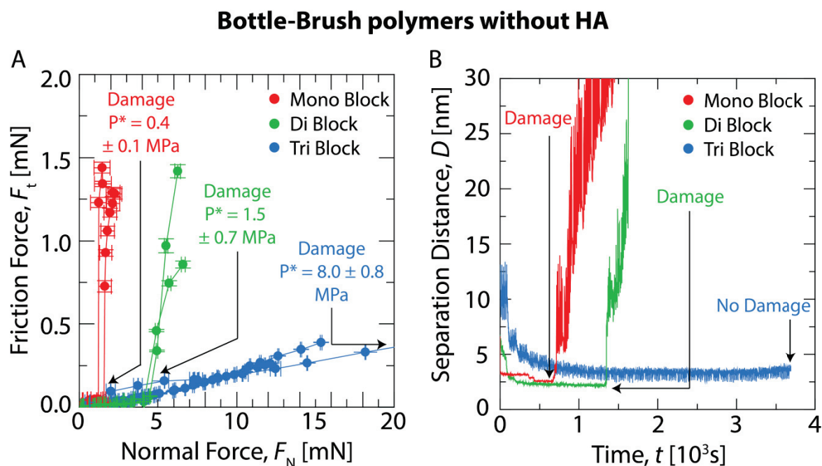
Figure 2.29. (A) Friction as a function of normal force for the mono, di and tri-blocks BB polymers at 100 \mu\text{g/mL} using the SFA. (B) Separation distance of the polymeric layer thickness as the function of time during tribotesting measured by the FECO fringes.
