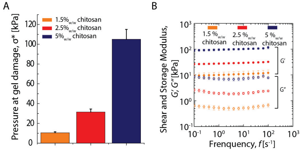
Figure 3.8. (A) Pressure at gel damage measured for the chitosan hydrogels on the DZ/DZ configuration and (B) shear and storage moduli of chitosan hydrogels.
