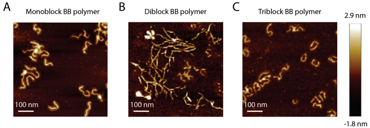
Figure 2.27. AFM pictures of the (A) monoblock, (B) di and (C) triblock BB polymers deposited on freshly cleaved mica surfaces at a concentration of 15 \mu\text{g/mL} .
