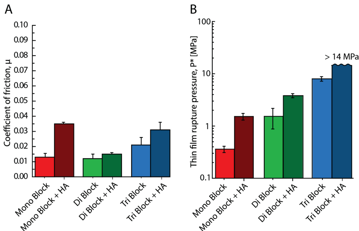
Figure 2.31. Histograms of the tribological results of the bioinspired fluid made of 100 \mu\text{g/mL} of BB polymer in presence or absence of 1.5 MDa HA at 1 \text{mg/mL} . (A) CoF as a function of the lubricant system and (B) the lubricating film rupture pressure, P^* , of the different lubricating systems.
