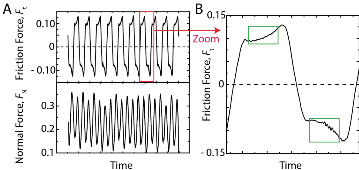
Figure 3.7. (A) Typical friction and normal forces profiles for 2.5 % w/w chitosan gels on the DZ/DZ configuration at a speed of v = 5 mm/s and (B) zoom in the friction profile showing no
