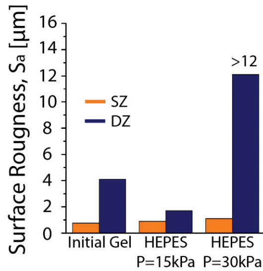
Figure 3.12. Quantitative analysis of gel roughness after 10^4 cycles at 5mm/s and under an applied load equals to 100% of elastic modulus of 2.5 % w/w chitosan hydrogel (30 kPa) in 0.1M HEPES buffer pH 7.4. The analyzed area was 20% of the total wear track.
