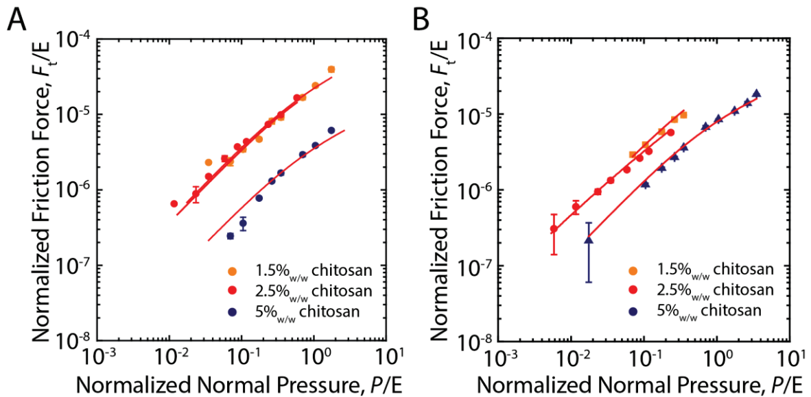
Figure 3.9. Friction forces as a function of normal pressure for (A) SZ/SZ configuration and (B) DZ/DZ configuration. Red lines are fitting obtained from Eq. 1.
