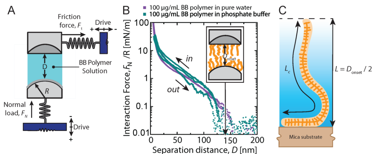
Figure 2.16. (A) SFA experimental setup used for normal force profiles and tribology experiments. (B) Interaction force profiles across BB solution at 100 \mu\text{g/mL} in pure water and in a phosphate buffer at 150 mM NaCl and pH 7.4. (C) Schematic representation of the BB polymer conformation on the mica substrate with its characteristic dimensions.
