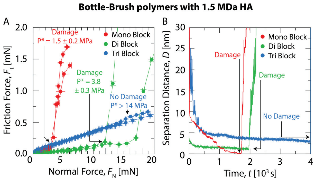
Figure 2.30. (A) Friction as a function of normal force for the mono, di and tri-blocks BB polymers at 100 \mu\text{g/mL} with 1.5 MDa HA at 1 \text{ mg/mL} using the SFA. (B) Separation distance of the polymeric layer thickness as function of time during tribotesting. Each stepwise decrement of the separation distance corresponds to an increase of the applied load.
