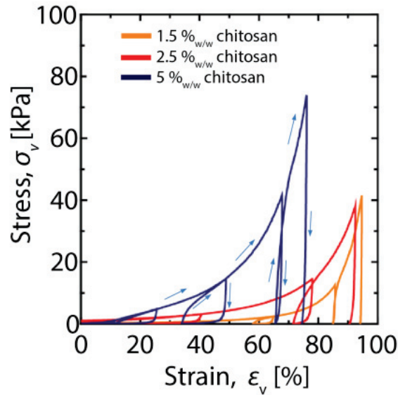
Figure 3.5. Stress versus strain curves of chitosan hydrogels
