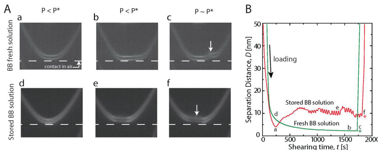
Figure 2.22. Evolution of FEKO fringe shape with pressure for (A) BB polymer fresh solution (a-c), and 3 months aged at 22°C BB polymer solution (d-f) White arrows, in A-c and f, highlight the region of wear initiation; (B) Separation distance as a function of time for fresh and stored BB polymer solutions. Initiation of wear is indicated by an asterisk.
