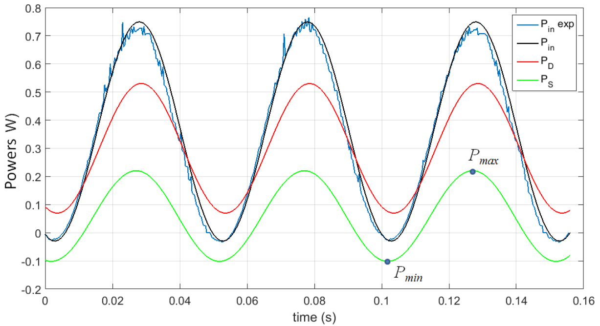
Figure 3.27 : General power analysis. The simulation and experimental input power ( P_{in\,exp} and P_{in} ) are plotted on the same graph to highlight the coherence. P_D is defined as the sum of the dissipated power ( P_{R0} , P_{bm} , and P_{eff} ) and P_S is the sum of P_{mechanic} and P_{Jm} . P_{max} and P_{min} are found for P_S but can be applied to the other power sources.
