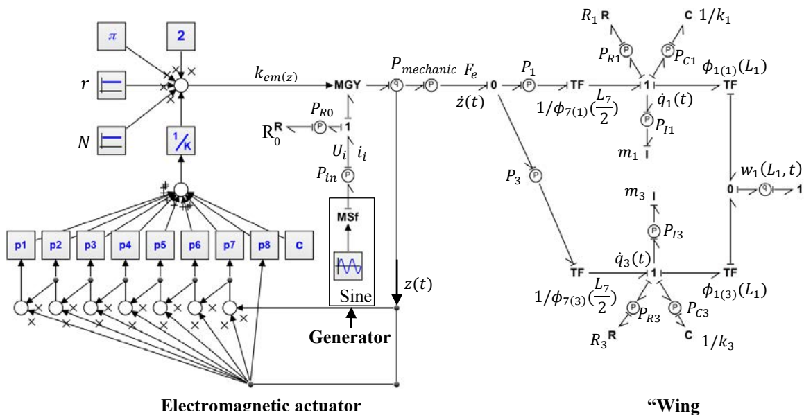
Figure 4.9: Global OVMI Bond Graph model.
