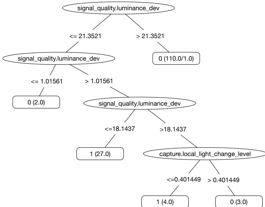
FIGURE 4.5 – An excerpt of the decision tree built from a sample of 500 configurations/-videos
