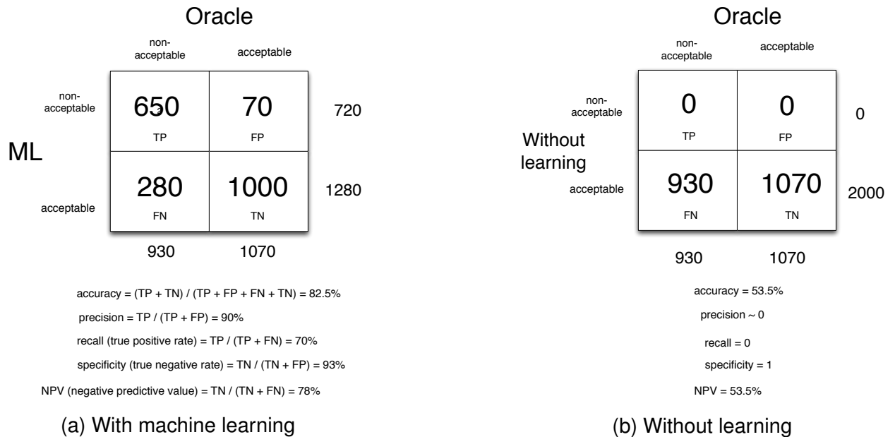
FIGURE 5.4 – Confusion matrix and classification metrics : with machine learning vs without learning (example)
