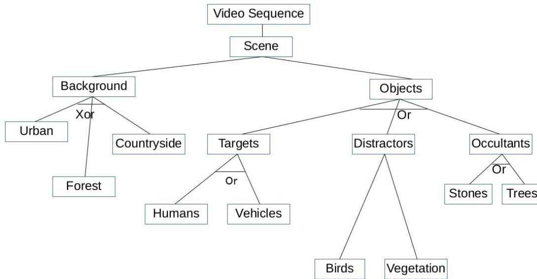
FIGURE 2.2 – A feature model representing how to create a Video Sequence
