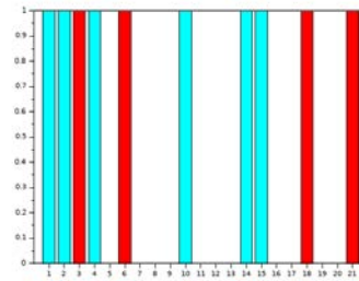
FIGURE 6.5 – The number of bins activated with the smaller test suite composed of 5 test cases that maximizes the dispersion score.
