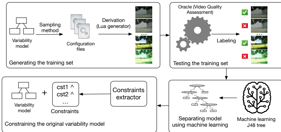
FIGURE 4.4 – Learning method on the video generator
