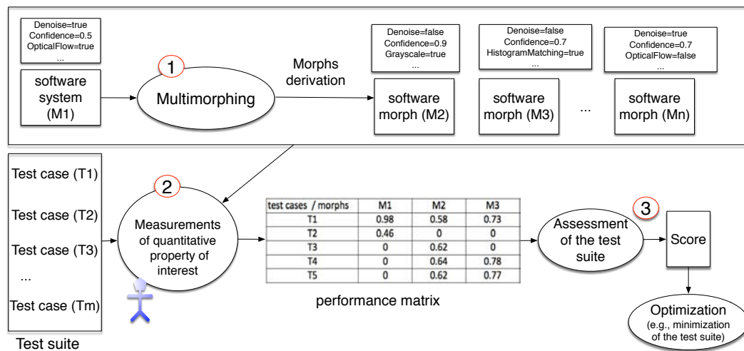
FIGURE 6.1 – Multimorphic process : morphs are automatically produced (e.g., thanks to parameters) ; for each morph test suite is executed and performance measurements are gathered ; a dispersion score is finally computed to characterize the quality of a test suite
