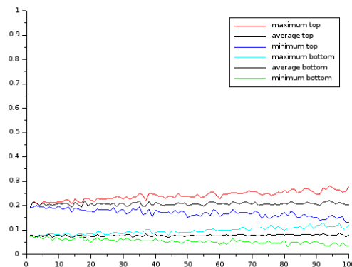
FIGURE 6.3 – Stability results for the property precision ; X-axis : number of morphs removed ; Y-axis : dispersion score
