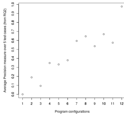
FIGURE 6.7 – Average precision measures over the 5 videos from RQ2. On X-axis are the CV morphs : first, the 6 first morphs that are supposed to perform moderately badly ; the 6 last morphs are supposed to be good. Y-axis reports the averaged precision measure over the test suite.
