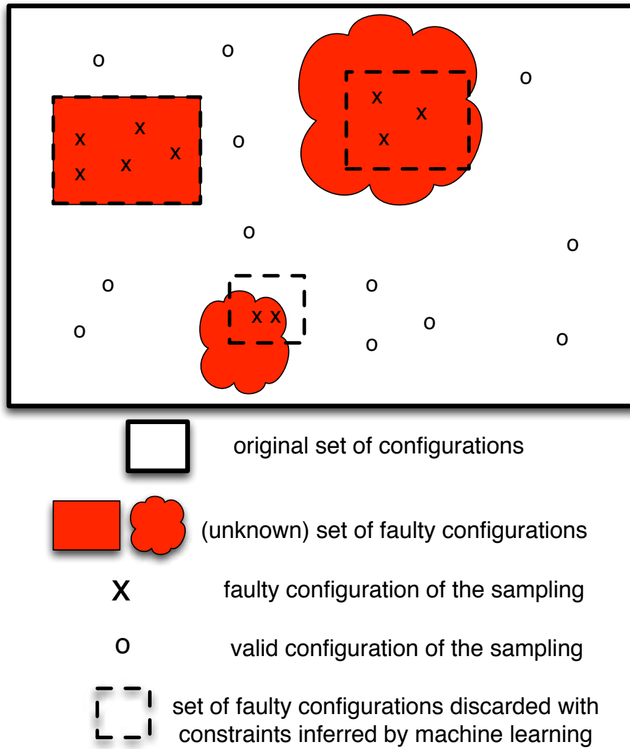
FIGURE 4.2 – Constraining the configuration space
