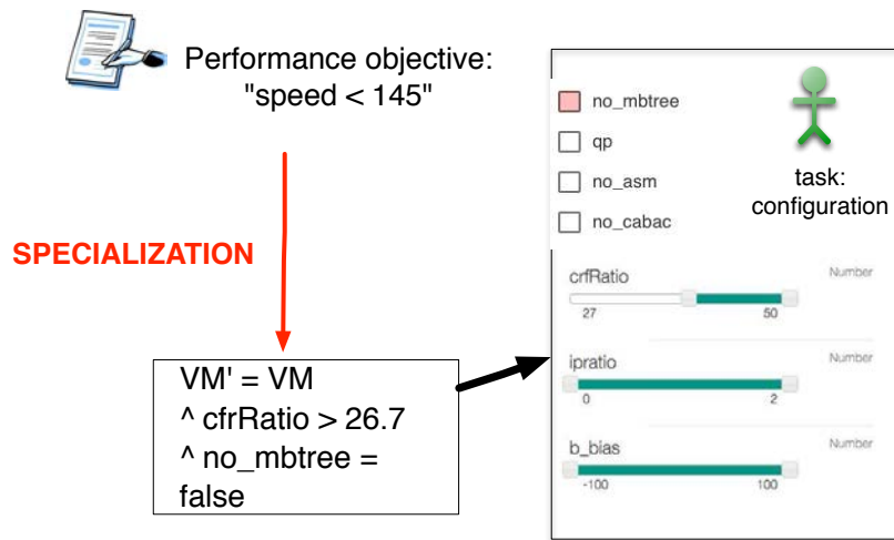
FIGURE 5.1 – Configuration of a specialized x264. Given a performance objective, the specialization method infers and fixes some options values (no_mbtrees and cfrRatio); users still have some flexibility to configure other options.
