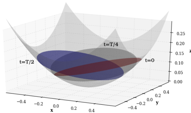
Figure 4.5 – Analytical solution of prop. 6, 3D planar surface in a parabolic bowl: free surface at t = 0 (red), t = \tau/4 (dark grey), t = \tau/2 (blue), with the period \tau defined by \tau = 2\pi/\omega .
