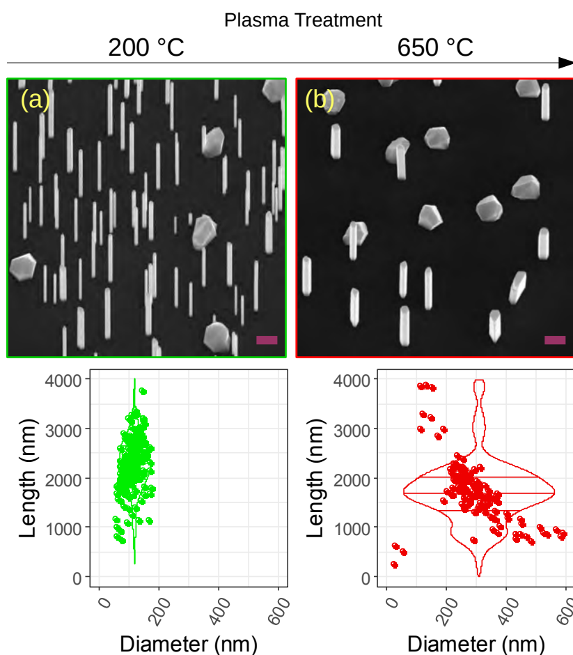
Figure 4.5 – Plasma treatment at low and high temperature. The SEM images on top corresponds to low (left) and high (right) temperature plasma treatment. The scatter plots on the bottom corresponds to the SEM images on top and show the evolution of nanowire length as a function of the diameter. The violin plots show the statistical distribution. The In Flux is 3.1 \times 10^{-8} Torr and As Flux is 2.4 \times 10^{-5} Torr . Growth temperature is 410 °C. Scale bars is 500 nm.
