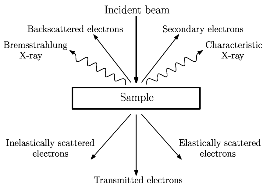
Figure 2.8 – Electron Matter Interactions
