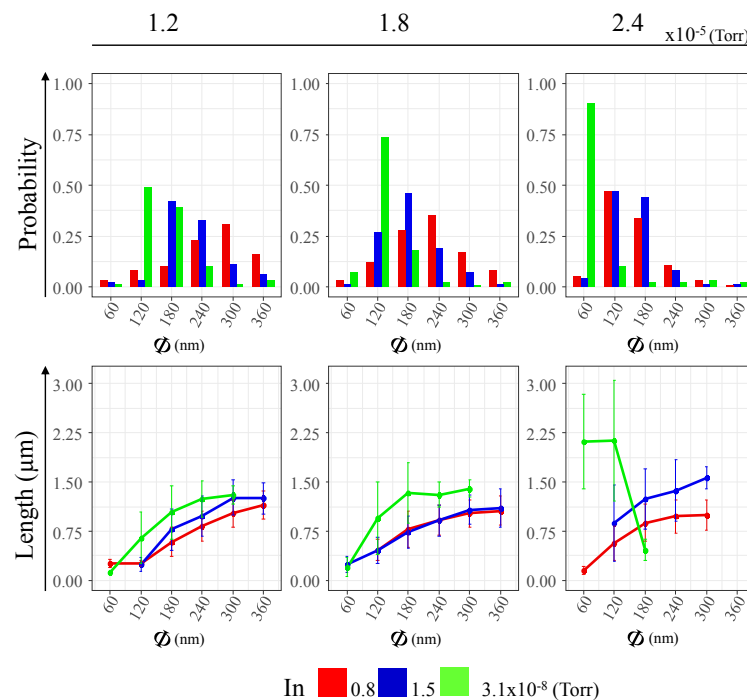
Figure 4.10 – Statistic plots for the H 2 -gas treated surfaces corresponding to the figure (1e) process. Nanowires are grouped in families of different diameters (See chapter 2 section 2.4). The three colors (red, blue, green) correspond to different indium fluxes. On top, the proportion of each family is reported as a function of the arsenic flux. On bottom, the mean length of each family is reported as a function of the arsenic flux. These statistic graphs allow to evaluate the influence of the indium and arsenic fluxes on the diameter and the length of the InAs nanowires.
