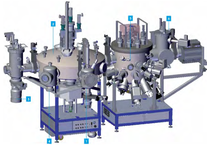
Figure 2.1 – Riber MBE-412. (1) The loading/unloading chamber, (2) the cluster, (3) the preparation chamber, (4) the parking, (5) the growth chamber and (6) the vacuum system. ( http://www.riber.com/assets/files/documentation/mbe412-imp2.pdf )
