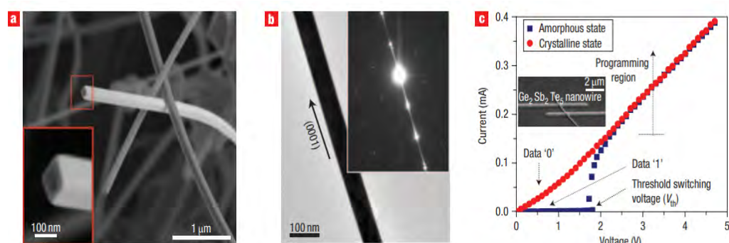
Figure 1.6 – Phase Change Memory with GeSbTe nanowires. (a) SEM image , (b) TEM image and (c) electrical characterisation (Lee. et al. 38 )
