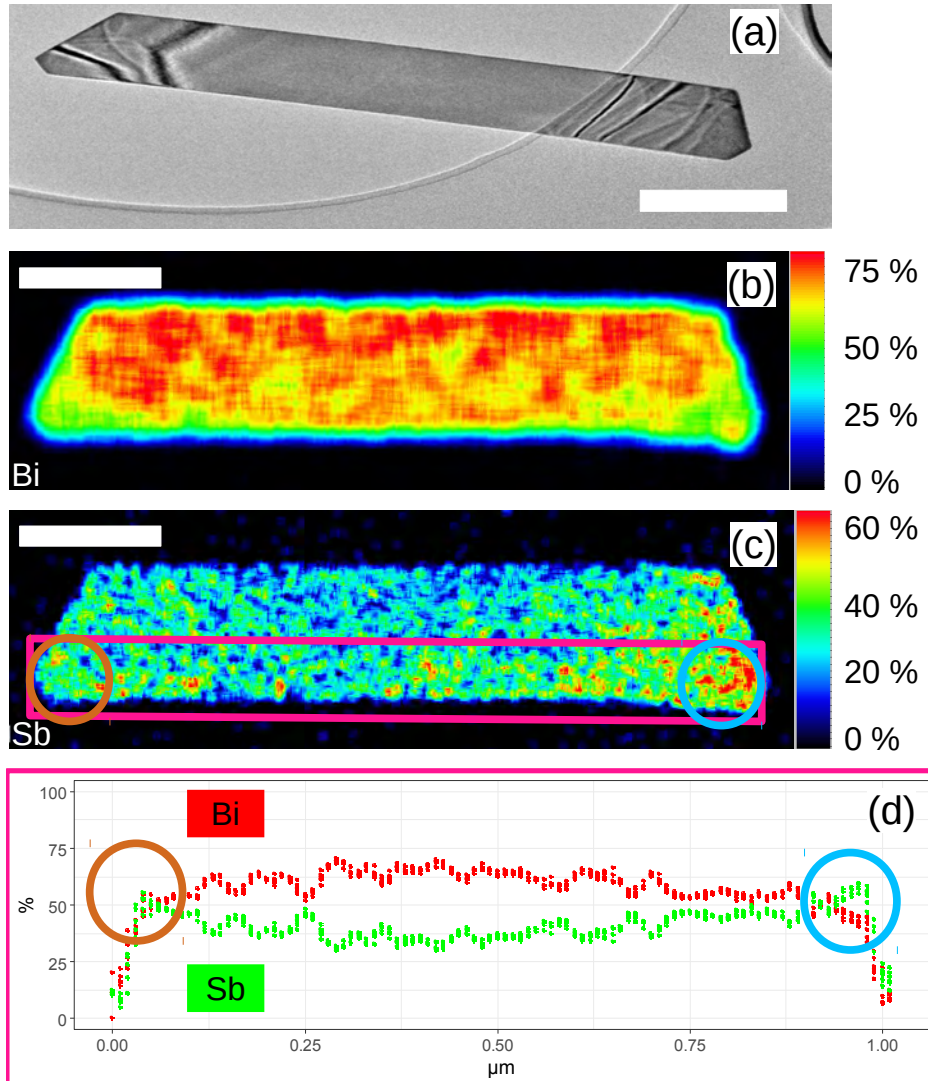
Figure 5.17 – EDX mapping of a Bi_{1-x}Sb_x nanoflake from figure. 5.11 (a) low resolution TEM image of the flake, (b) Bi compositional mapping of the flake, (c) Sb compositional mapping of the flake and (d) EDX mapping of the pink region of (c) with Bi in Red and Sb in Green. The two circles in (c) and (d); (brown in left and cyan in right) in (d) correspond to an increase of the Sb composition. Scale bars are 250nm.
