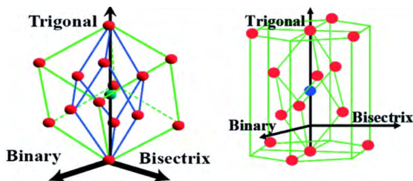
Figure 5.8 – Crystalline structure of the \text{Bi}_{1-x}\text{Sb}_x alloys. (Tang et al. 317 )
