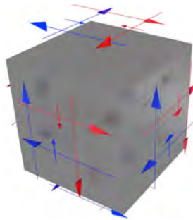
Figure 5.4 – 3D Sketch of a 3D Topological Insulator. The long arrows represent the momentum while small arrows represent the spin.
