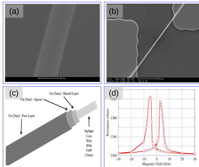
Figure 1.5 – Nanowire based spin-valve. (a) Close up scanning electron microscope image of a typical Ni/NiO nanowire. (b) Scanning electron microscope image of an isolated nanowire spin valve on an insulating substrate with 150 nm thick Ta contacts for magnetoresistance measurements. (c) Schematic of the implemented spin valve multilayer on a nanowire core. The first CoO shell biases the Co reference layer. A Cu spacing layer is then followed by the Co reference layer. (d) Magnetoresistive response of a nanowire spin valve at 10 K following a 30-kOe field cool at 380 K. The magnetoresistance value is approximately 9%. (Chan et al. 27 )
