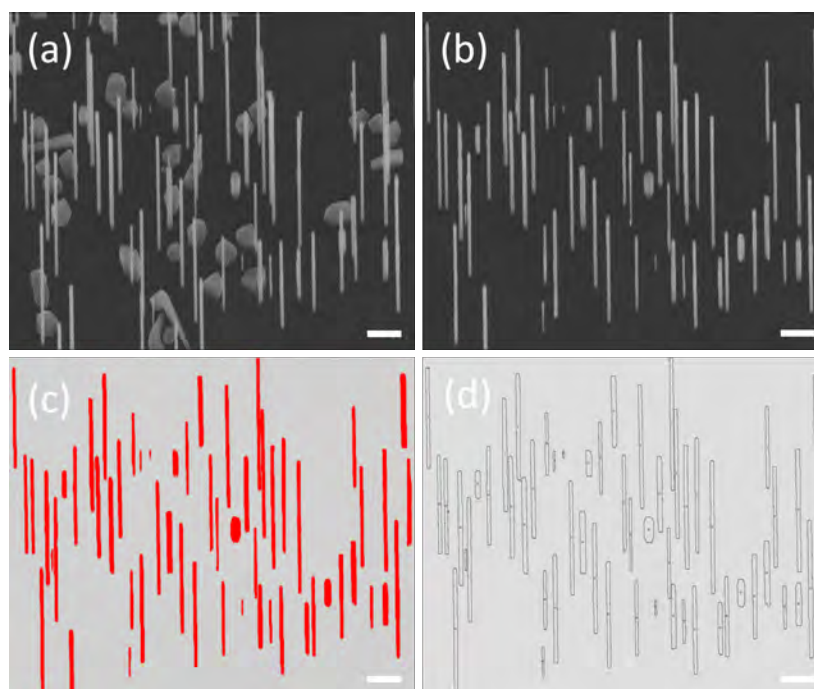
Figure 2.13 – Image Processing Steps. (a) Original SEM image, (b) image segmentation: separating overlapping nanowires, (c) image inversion and thresholding and (d) particle detection. Scale bars are 500nm.
