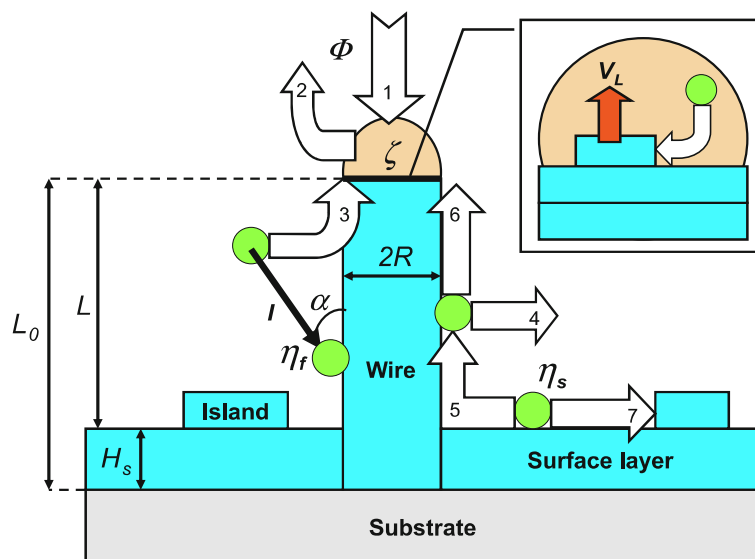
Figure 3.1 – Kinetics of the VLS mechanism. (Dubrovskii 199 )
