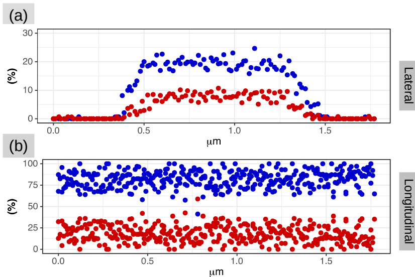
Figure 5.16 – EDX profiles of a \text{Bi}_{1-x}\text{Sb}_x nanowire. (a) in the lateral direction and (b) in the longitudinal direction
