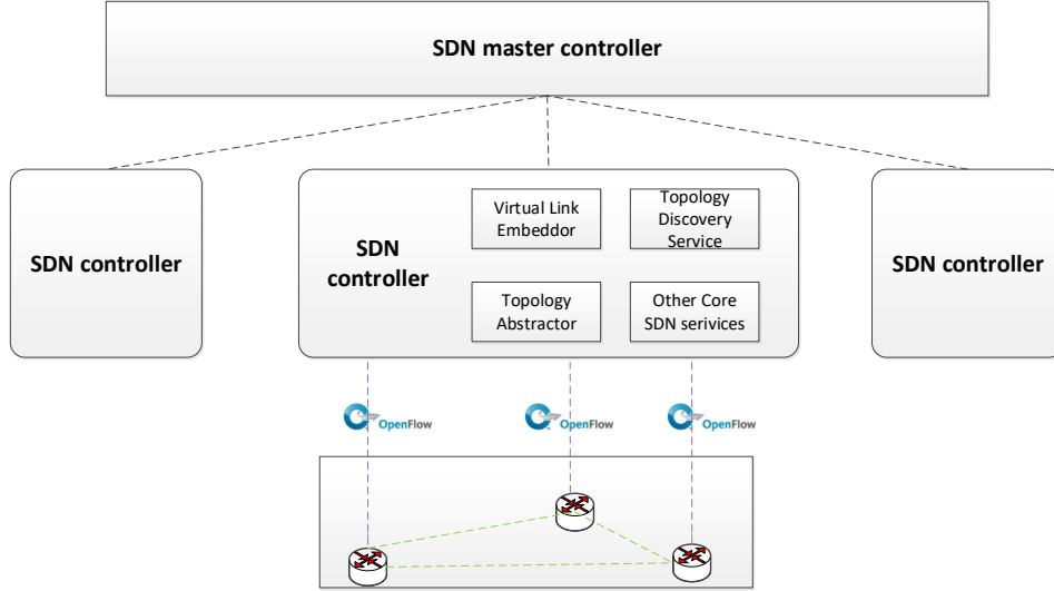
FIGURE 5.1 – Illustration of a two level-hierarchy of controllers for multi-domain networking
