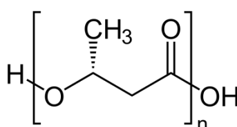
Figure 85. Polyhydroxybutyrate.
