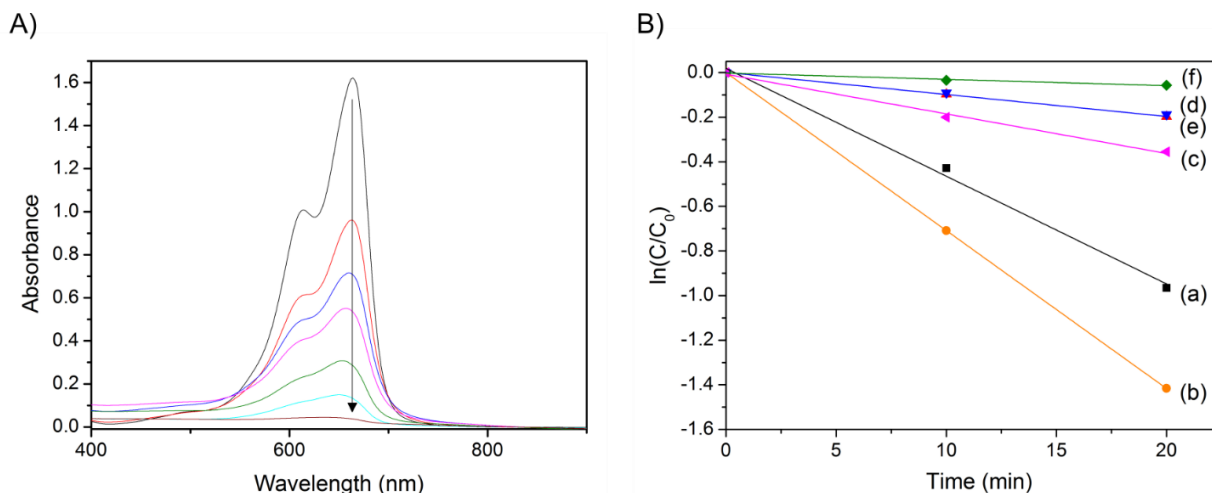
Figure 9. (A) Absorbance change in the visible range of methylene blue solution after various illumination time for 0.1 wt% NiO-TiO 2 : before irradiation (black), 10 min (red), 20 min (blue), 30 min (magenta), 40 min (olive), 50 min (cyan) and 60 min (purple). (B) Pseudo-first order kinetic expressed by \ln(C/C_0) vs irradiation time t of the degradation of MB for the pure TiO 2 (a, black), NiO/TiO 2 containing 0.1 (b, orange), 0.2 (c, magenta), 0.5 (d, blue), 1.0 (e, red), and 10 wt % (f, olive).
