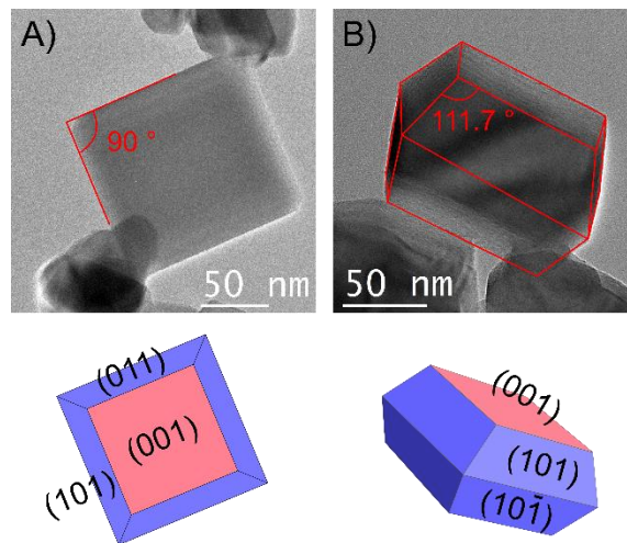
Figure 2. Bright field TEM images of the pure TiO 2 recorded along (A) the [001] zone axis and (B) the tilted along the [010] direction.
