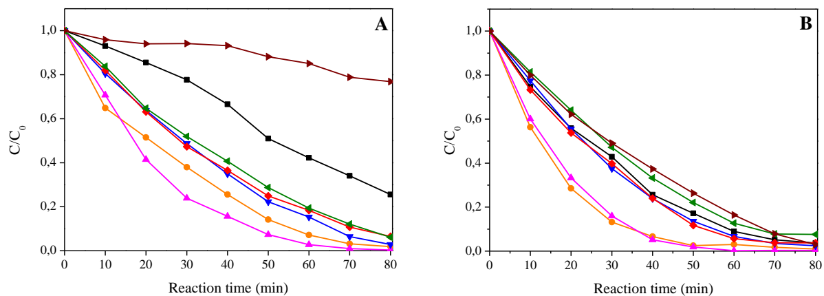
Fig. S7: Kinetic of the degradation of MB ( A , left) and MO ( B , right) of pure \text{TiO}_2 (black), 0.1wt% \text{NiO-TiO}_2 (orange), 0.25wt% \text{NiO-TiO}_2 (magenta), 0.5wt% \text{NiO-TiO}_2 (blue), 1wt% \text{NiO-TiO}_2 (red), 2wt% \text{NiO-TiO}_2 (olive) and 10 wt% \text{NiO-TiO}_2 (brown) nanomaterials.
