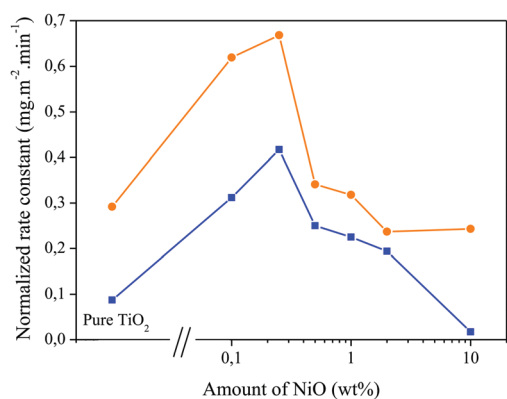
Fig. 8 Normalized rate constant K_{norm} as a function of the NiO amount for the degradation of MB (squares, blue) and MO (circles, orange).
