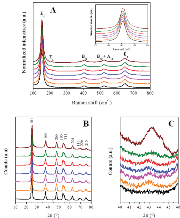
Fig. 2 (A) Raman spectra (inset: expansion of the 100–200 cm -1 region); (B) XRD patterns; (C) expansion of the 2θ region for the pure TiO 2 (black), 0.1 wt% NiO–TiO 2 (orange), 0.25 wt% NiO–TiO 2 (magenta), 0.5 wt% NiO–TiO 2 (blue), 1 wt% NiO–TiO 2 (red), 2 wt% NiO–TiO 2 (olive) and 10 wt% NiO–TiO 2 (brown) nanomaterials.
