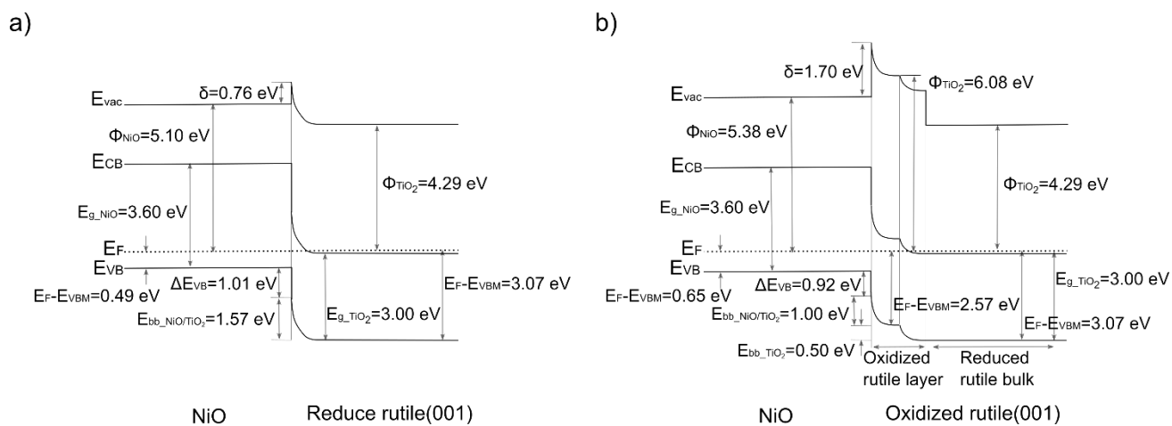
Figure S2. Band energy diagrams of p-NiO/n-TiO 2 for reduced and oxidized rutile (001)
