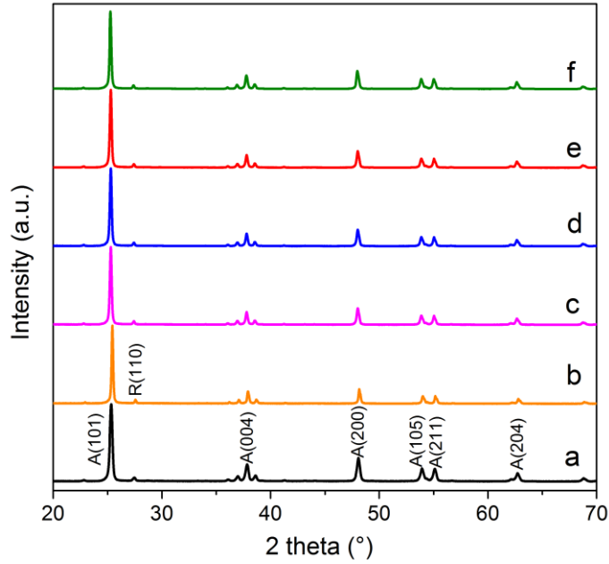
Figure 1. XRD pattern of the pure TiO 2 (a, black), 0.1 (b, orange), 0.2 (c, magenta), 0.5 (d, blue), 1.0 (e, red), and 10 wt % (f, olive) NiO-TiO 2 composites.
