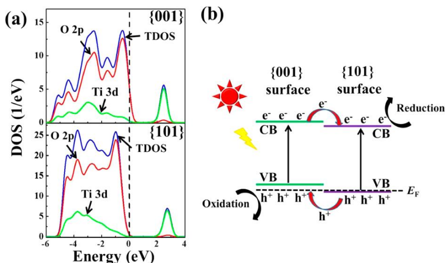
Figure 2.24. (a) Density of states plots for anatase (101) and (001) surfaces. (b) Energy junction at the interface between (101) and (001) surfaces described based on the calculation. Reproduced from ref 112 .
