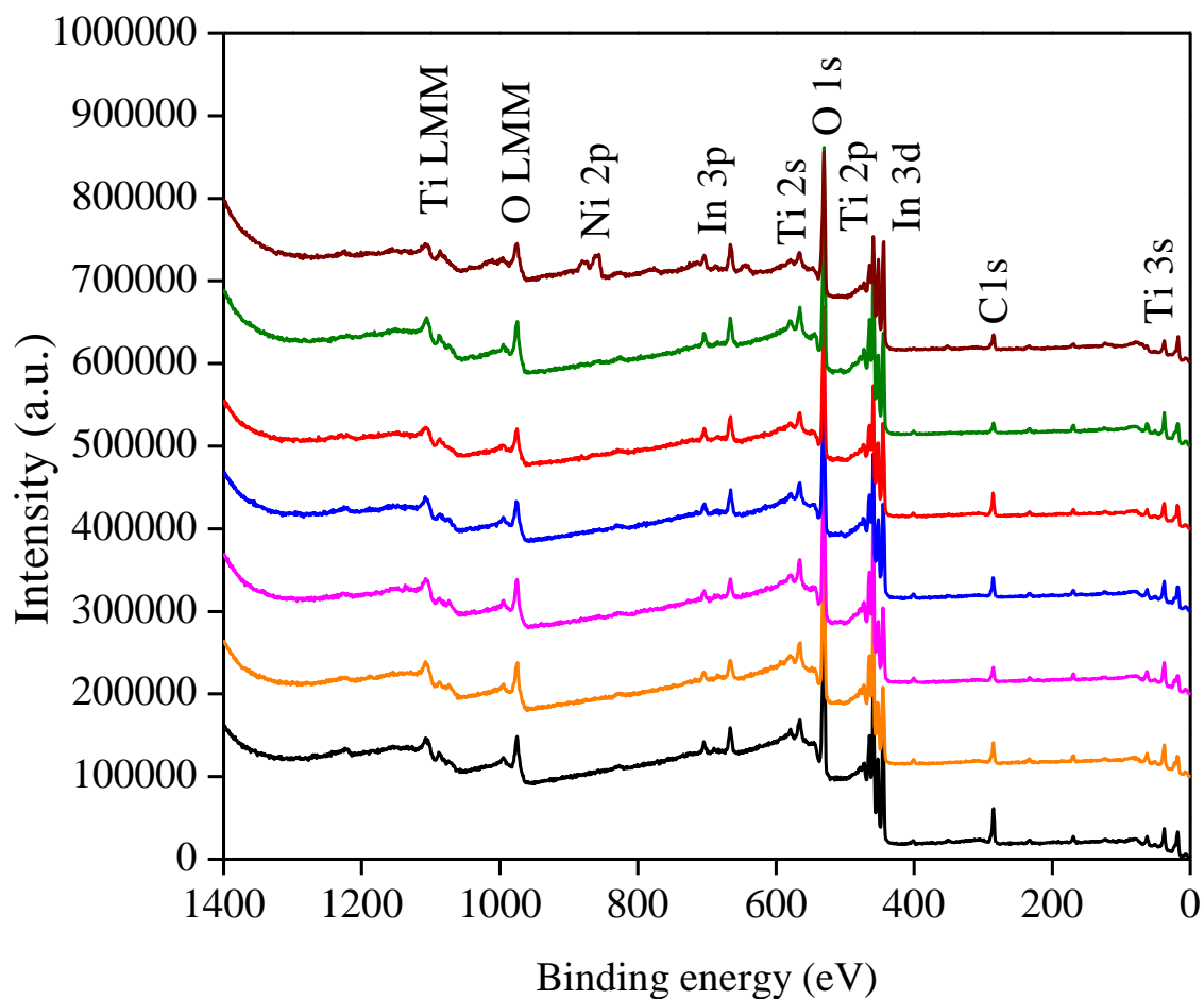
Fig. S6: XPS survey spectra of pure \text{TiO}_2 (black), 0.1wt% NiO- \text{TiO}_2 (orange), 0.25wt% NiO- \text{TiO}_2 (magenta), 0,5wt% NiO- \text{TiO}_2 (blue), 1wt% NiO- \text{TiO}_2 (red), 2wt% NiO- \text{TiO}_2 (olive) and 10 wt% NiO- \text{TiO}_2 (brown) nanomaterials.
