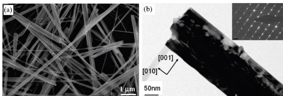
Figure 2.29. (a) SEM image and (b) bright-field TEM image of anatase nanobelts. The inset is a selected area electron diffraction pattern taken along the [100] direction of the nanobelt. Reproduced from ref 158 .
