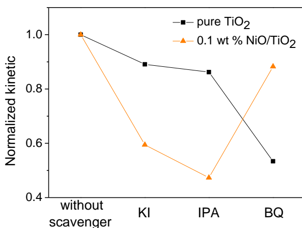
Figure 10. Kinetic rate constants for MB decomposition normalized by that without scavengers for pure TiO 2 (black) and 0.1wt% NiO/TiO 2 (orange) without scavengers or in the presence of potassium iodide (KI), isopropanol (IPA), and 1,4-benzoquinone (BQ).
