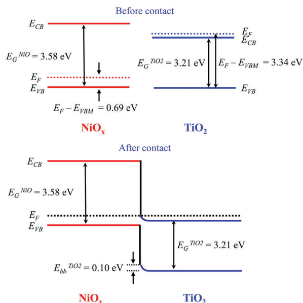
Fig. 6 Energy band alignment at the interface of \text{NiO}_x and \text{TiO}_2 . E_F , E_{CB} , E_{VB} , E_G^{\text{NiO}} , E_G^{\text{TiO}_2} , and E_{bb}^{\text{TiO}_2} represent the Fermi level, the conduction band minimum, the valence band maximum, the band gap of \text{NiO}_x , band gap of \text{TiO}_2 , and band bending, respectively.
