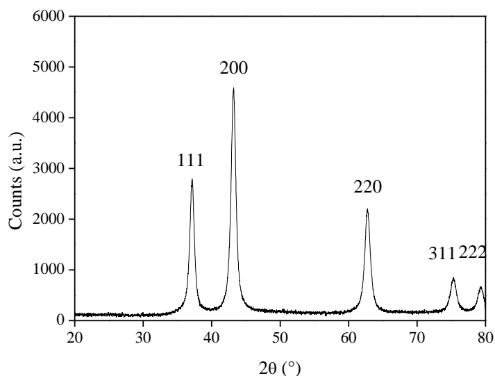
Fig. S1: XRD pattern of pure NiO synthesized by the SFCD route.
