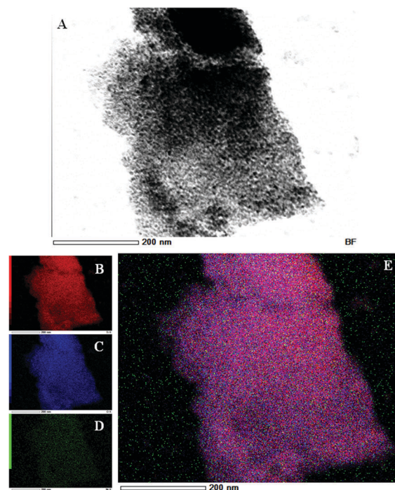
Fig. 3 (A) Bright field STEM micrograph of the 2 wt% NiO–TiO 2 nanomaterials and EDX elemental mapping of (B) Ti, (C) O, and (D) Ni. (E) 3-Colour image obtained by superimposed chemical elemental mapping.
