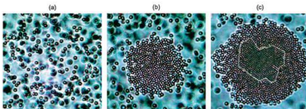
Figure 2.27. Two step nucleation observed for colloidal particles. a) Initial dilute liquid phase. b) Amorphous dense droplets. c) Crystalline nuclei created from the amorphous phase. Reproduced from ref 141 .
