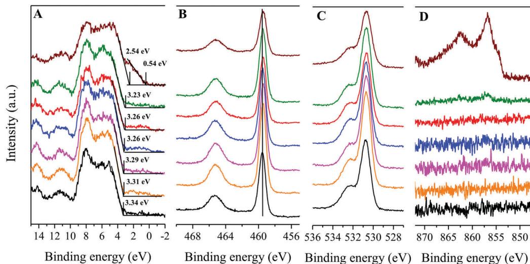
Fig. 5 High resolution XPS spectra of the valence band (A), Ti 2p_{3/2} (B), O 1s (C), and Ni 2p_{3/2} (D) for the pure \text{TiO}_2 (black), 0.1 wt% NiO– \text{TiO}_2 (orange), 0.25 wt% NiO– \text{TiO}_2 (magenta), 0.5 wt% NiO– \text{TiO}_2 (blue), 1 wt% NiO– \text{TiO}_2 (red), 2 wt% NiO– \text{TiO}_2 (olive) and 10 wt% NiO– \text{TiO}_2 (brown) nanocomposites.
