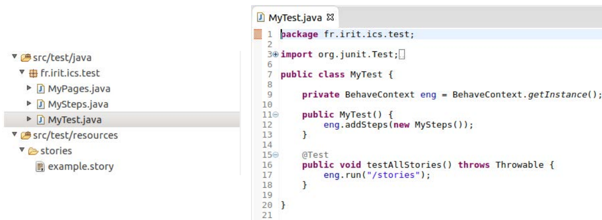
Figure 77. Package tree (on the left) and MyTest class (on the right).
