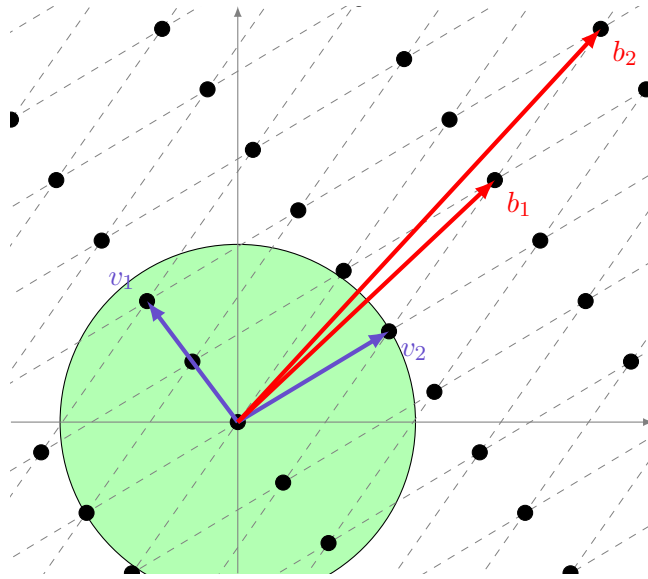
Figure 2.11: Approximate Shortest Independent Vector Problem ( SIVP_\gamma ).
