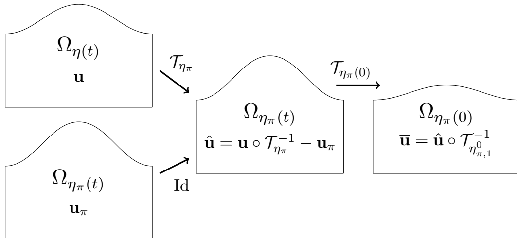
Figure 1.3: The changes of variables used in Chapter 4. (\mathbf{u}_\pi, \eta_\pi) are the velocity and beam displacement of the periodic solution around which we want to stabilise the perturbed solution, with velocity and beam displacement (\mathbf{u}, \eta) .
