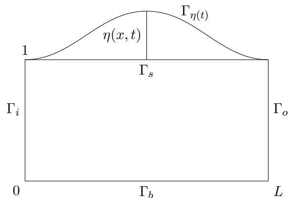
Figure 1.1: Domain \Omega_{\eta(t)}
