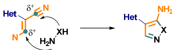
Figure 1.3. A schematic representation of the synthesis of 4-hetaryl-5-aminopyrazoles from acyclic \alpha -hetaryl- \beta -enaminonitriles.
