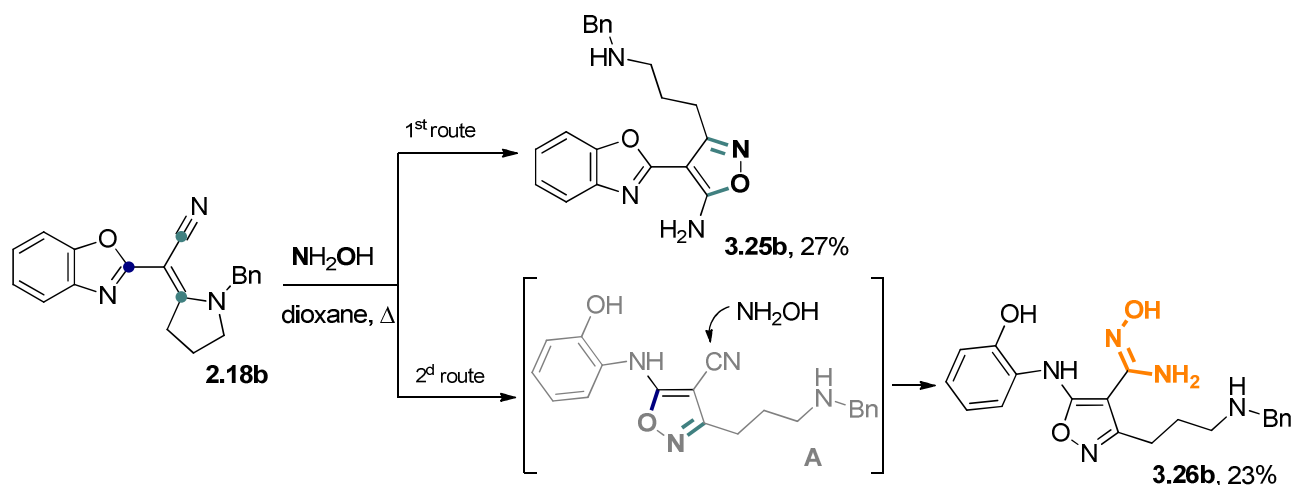
Scheme 3.10. Reaction of benzoxazol-2-yl-2-(1-benzylpyrrolidin-2-ylidene)acetonitrile 2.18b with hydroxylamine.
