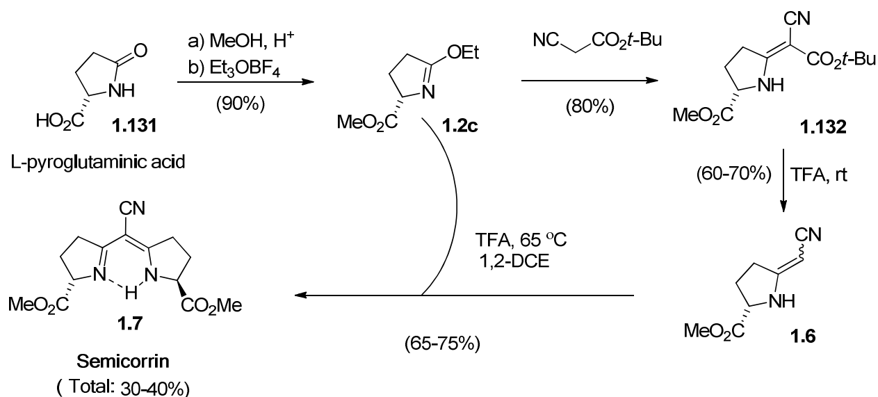
Scheme 1.47. Semicorrins synthesis.
