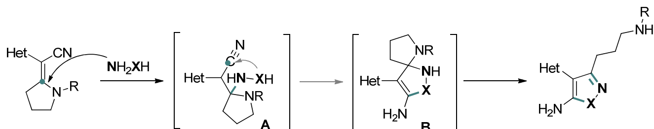
Scheme 3.2. Proposed mechanism for the ring conversion.
