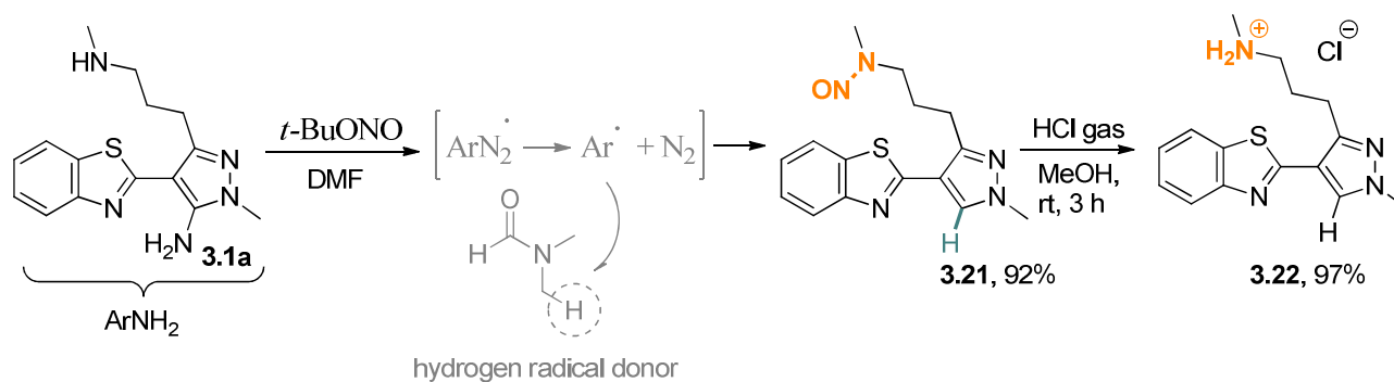
Scheme 3.7. Reductive deamination of 4-benzothiazol-2-ylpyrazole 3.1a .
