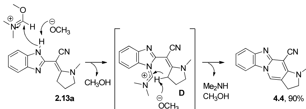
Scheme 4.4. Proposed mechanism for reaction of 2-(1H-benzo[d]imidazol-2-yl)-2-(1-methylpyrrolidin-2-ylidene)acetonitrile 2.13a with DMF DMA.
