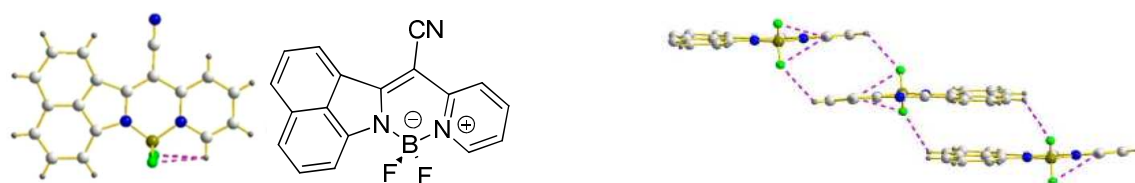
Figure 1.11. a) X-ray structural analysis of 1.120 . b) Aggregates 1.120 with head-to-tail packing
