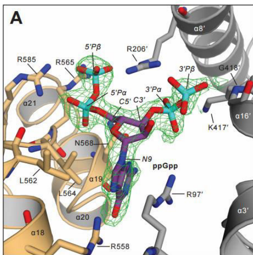
Figure 56. 3D structure of the ppGpp binding site in LdcI . A) The key residues for ppGpp binding are indicated in the figure: R97, R206, G416, K417, L562, L564, R565, N568, R585. B) Sequence alignment of LdcA ( P. aeruginosa ) and LdcI , LdcC , AdiA ( E. coli ). We find that the conserved L562, R565 and R585 are replaced by alanine, proline, and glycine respectively in LdcA . The analysis was performed by I. Kandiah.
