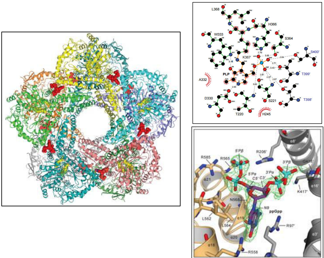
Figure 24.- The decameric structure of the lysine decarboxylase LdcI from E. coli (left). Each monomer is shown in a particular color, ppGpp residues are displayed in red. Right, up : Residues of the PLP Binding site and the important residues for stabilizing the PLP cofactor. Right, down : ppGpp binding site, the ppGpp is shown in the electron density while important residues belonging to LdcI are displayed as cartoon in beige or gray. Nitrogen are displayed in blue, oxygen atoms are in red, phosphate atoms are in cyan, the carbon atoms from the ppGpp molecule are shown in violet or black as shown in the upper figure 254,284,300 .
