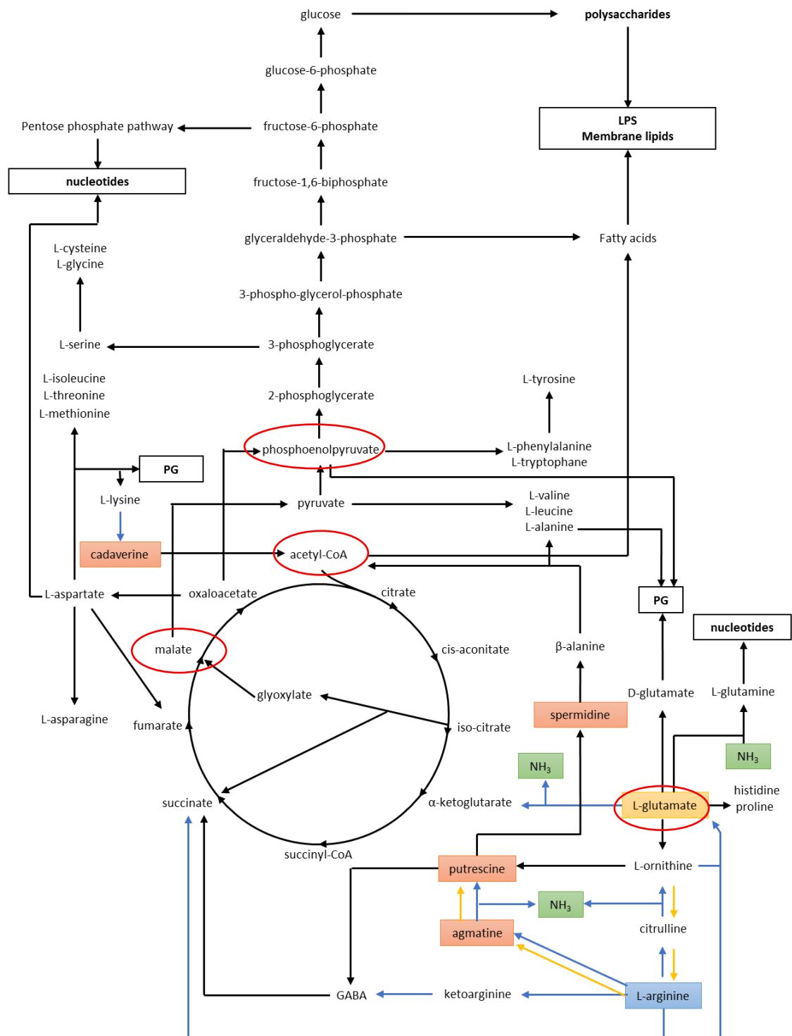
Figure 60: Diagram of central carbon and nitrogen metabolism when P. aeruginosa grows on glutamate. Glutamate is assimilated into the Krebs Cycle by the activity of the NADH-Glutamate dehydrogenase, or by the activity of transaminases. The diagram also shows the effect of the activation of ArgR by the addition of L-arginine (blue), ArgR activation modifies the pathways in blue arrows, yellow arrows represent the pathways in absence of arginine. Red circles highlight metabolites that show different utilization compared to growth in glucose. Built from KEGG and MetaCyc databases.
