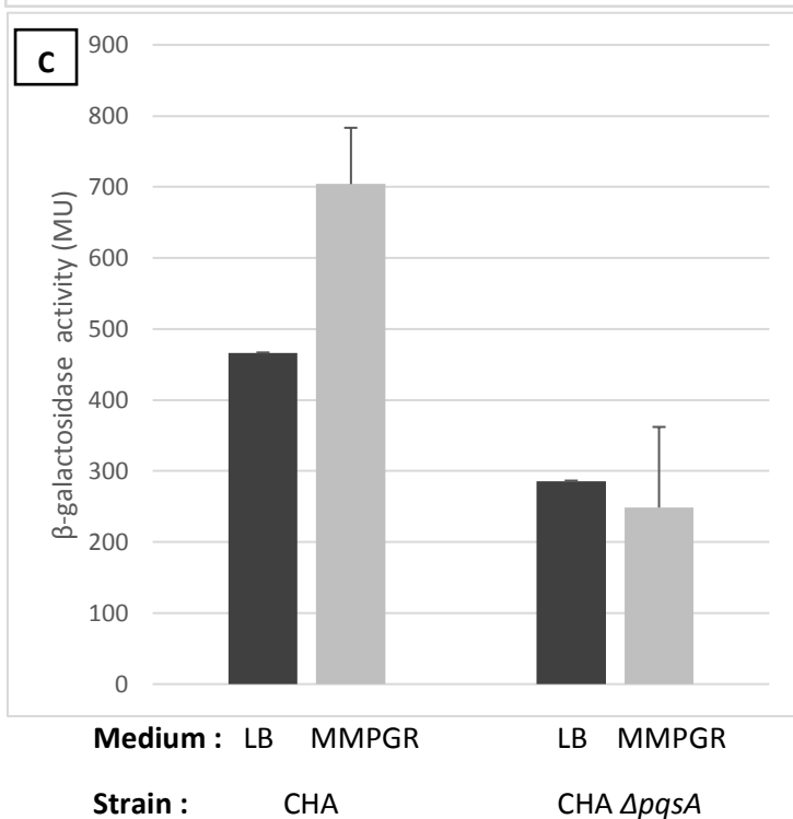
Figure 36. Expression profile of pldcA-lacZ fusions in CHA strains in different media. A) \beta -galactosidase activity of CHA:: pldcA-lacZ (blue), CHA \Delta rpoS :: pldcA-lacZ (yellow) and CHA \Delta lasI\Delta rhII :: pldcA-lacZ (orange), when growing in LB medium (well-aerated cultures). B) \beta -galactosidase activity of CHA:: pldcA-lacZ (blue) and CHA \Delta pqS A :: pldcA-lacZ (gray), when growing in LB medium (well-aerated cultures) and C) in stationary phase (overnight cultures) in either LB or Minimal medium with 20mM Glutamate + 20mM Arginine. For A) and B), growth curves are represented in the same graph in the secondary OD600nm axis.
