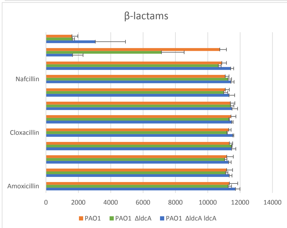
Figure 44. Effect of Cephalosporines and \beta -lactams in growth fitness of PAO1, PAO1 \Delta ldcA, PAO1 \Delta ldcA ldcA.
