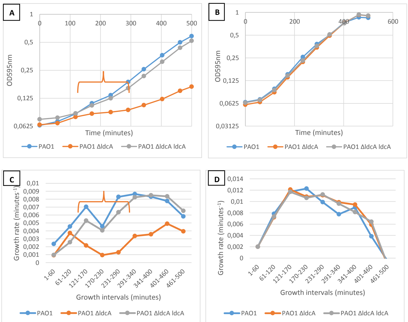
Figure 47. Growth of PAO1, PAO1 \Delta IdcA , PAO1 \Delta IdcA IdcA in minimal medium with Glucose or Glutamate. A) Growth curve in MMP Glutamate 20mM. B) Growth curve in MMP Glucose 20mM of the same strains. C) and D) Curves representing the growth rate of each growth interval of curves A and B respectively. Curves C and D allow to see the variation of the growth rate throughout cell growth. Experiments were performed at least 3 times with two independent mutants and their complement strains.
