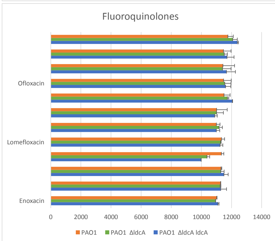
Figure 43. Effect of Aminoglycosides and Fluoroquinolones in growth fitness of PAO1, PAO1 \Delta ldcA, PAO1 \Delta ldcA ldcA.
