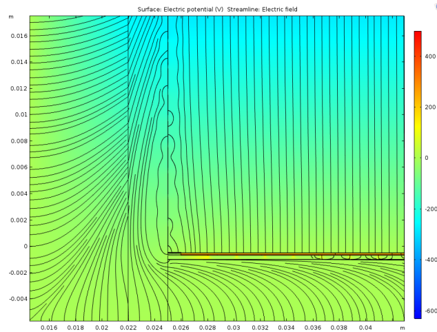
Figure 8.11. Anode corner where the Micromegas plane has been made flush with the wall of the TPC and the distance between the field cage and Micromegas mesh is 0.5 mm, and same as the inter-electrode spacing in the field cage. Distances are shown in meters.
