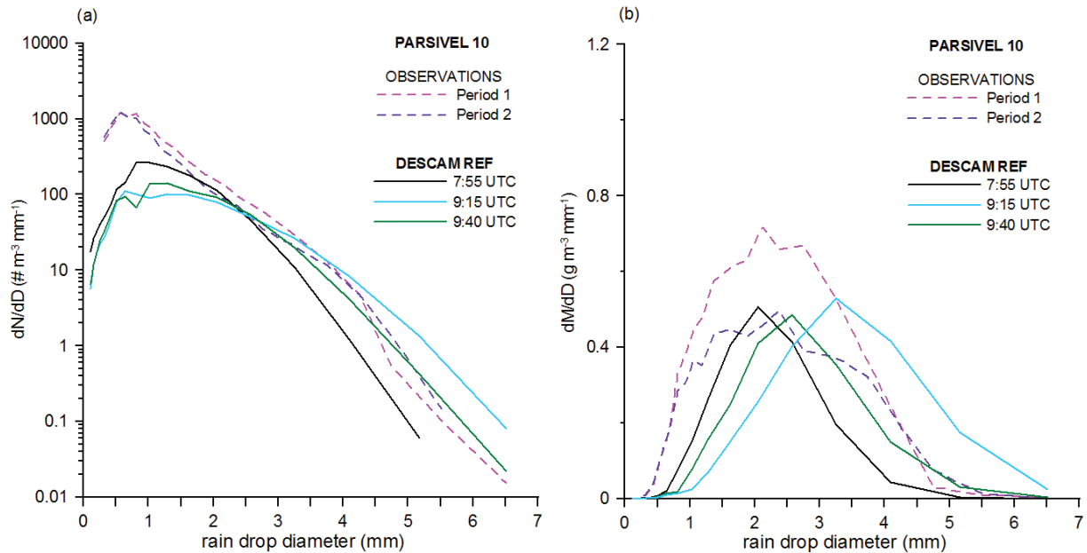
Figure 4.18: (a) Number density distributions of droplets ( m^{-3} mm^{-1} ) by the Parsivel 10 observations (dashed lines) during the Period 1 and Period 2 and the DESCAM reference (REF) simulation results at different moments and (b) corresponding mass size distributions ( g m^{-3} mm^{-1} ). The simulated mean rain water content at 7:55 UTC, at 9:15 UTC and at 9:40 UTC is 0.97 g m^{-3} , 1.35 g m^{-3} and 1.11 g m^{-3} respectively.
