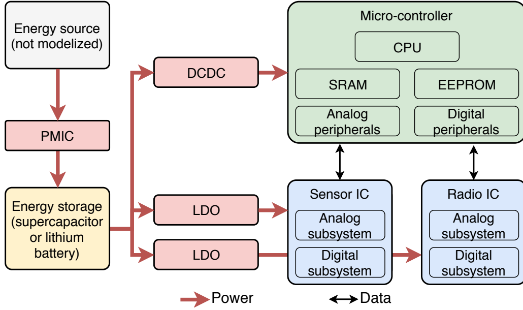
Figure 1.16: WSN model used for the lifetime estimation of components.
