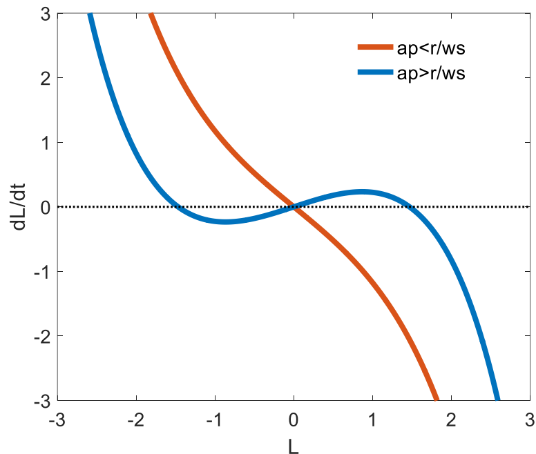
Figure S2: The Pitchfork Bifurcation
