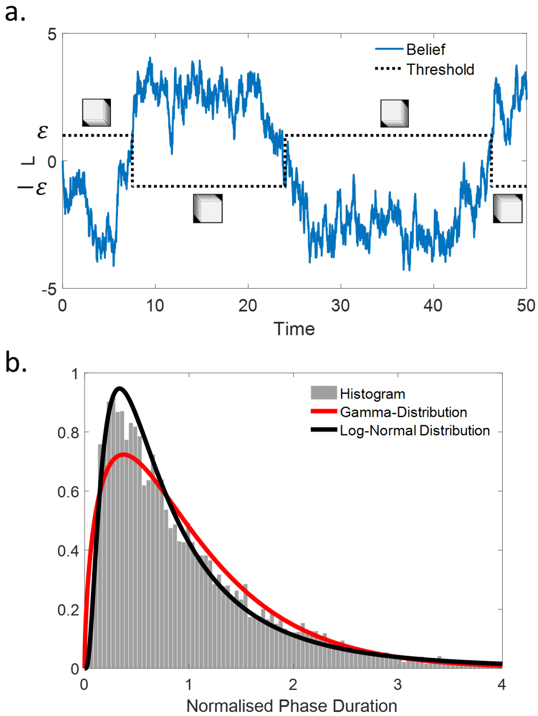
Figure S4: MAP with hysteresis and histogram. (a.): A switch occurs only if there is substantial evidence for the opposite interpretation (more conservative decision criterion). (b.) With this additional assumption, the model predicts gamma (or log-normal)-distributed phase duration histograms
