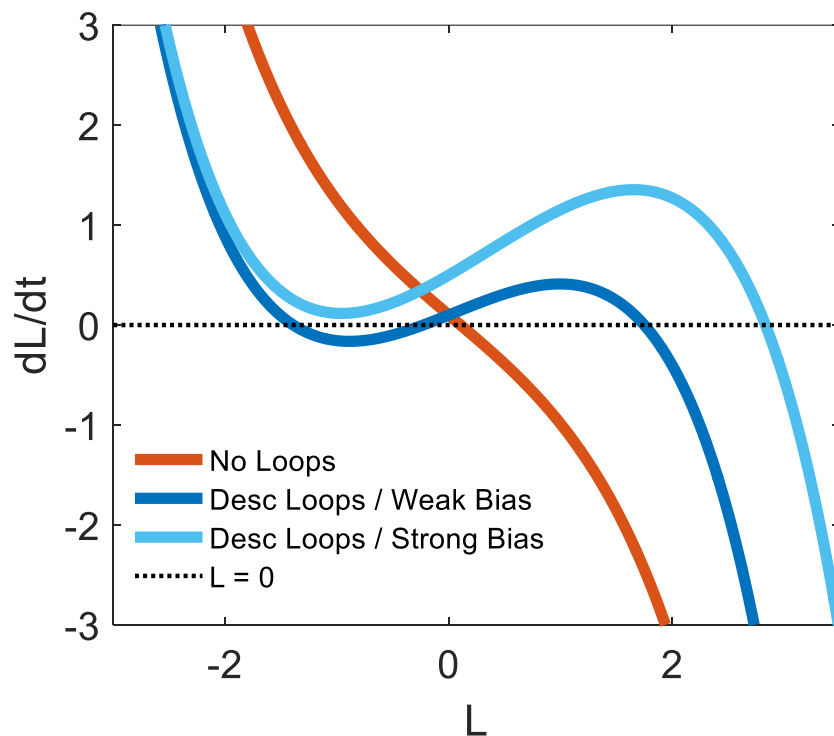
Figure S3: The Saddle-Node bifurcation. The light blue curve corresponds to an extremely strong implicit bias (the system gets stuck to interpretation 1)
