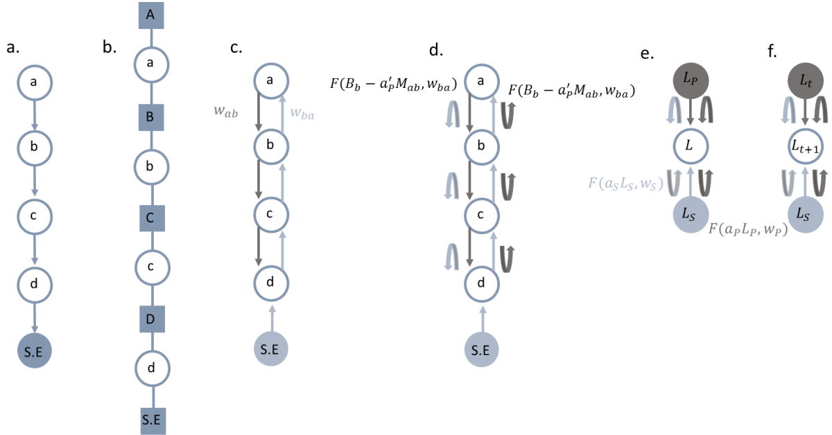
Figure S1: BP and discrete model. (a.): The generative model as Bayesian network. (b.): The factor graph. (c.): Belief propagation. (d.): Circular inference. (e.): A simplified model for circular inference [25]. (f.): The discrete model.
