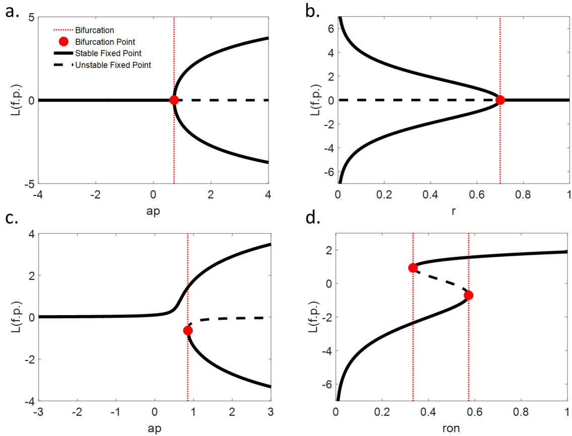
Figure 4: Bifurcation Diagrams. Descending loops change the dynamical behaviour of the system ((a.,b.): Pitchfork bifurcation for symmetrical systems; (c.,d.): Saddle-Node bifurcation for asymmetrical systems). When transition rates become too small, the fixed points go to infinity and the system becomes unstable (b.). Additionally, bistability can exist in a narrow range around symmetry (d.).
